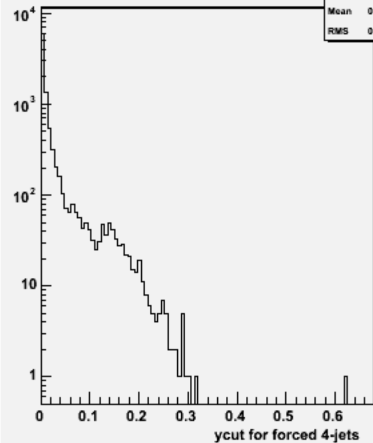
Ycut for 4-jets :w101621 uun2e2e2n2_o
