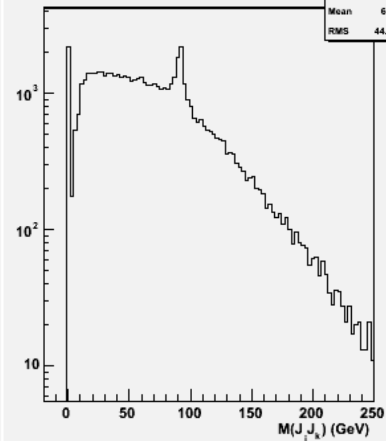
2jets mass(All comb)w101621 uun2e2e2n2_o
