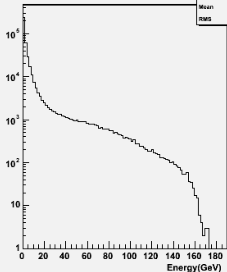
Particle Energy : w101621 uun2e2e2n2_o
