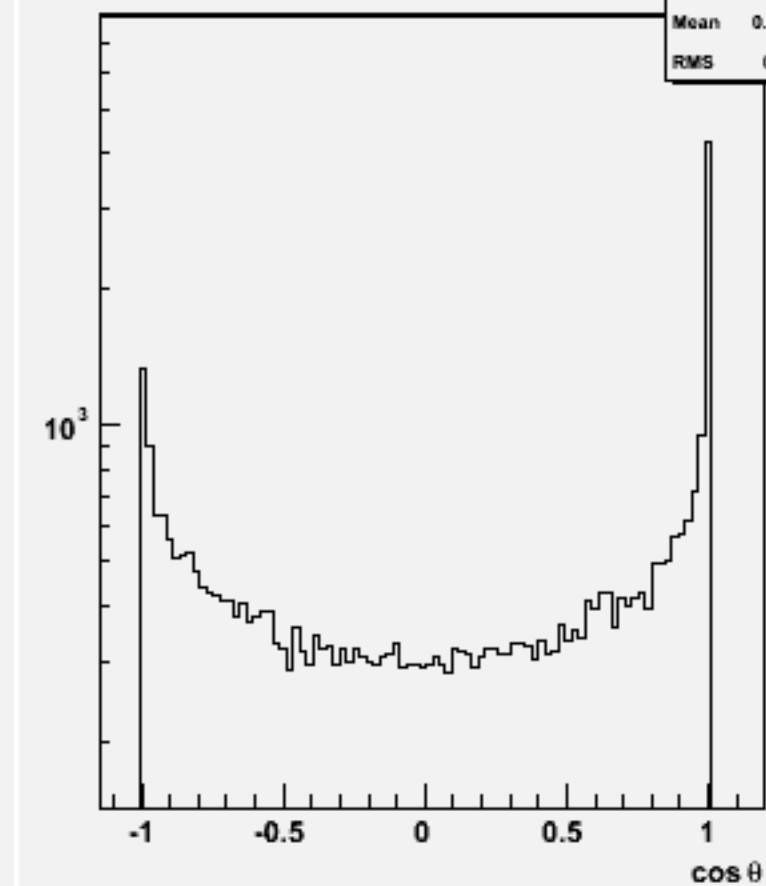
Jet cos \theta (All jets)w101621 uun2e2e2n2_o
