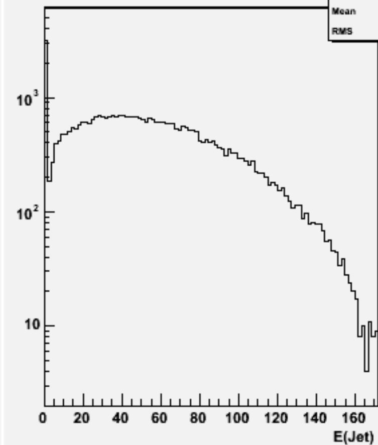
Jet energies(All jets)w101621 uun2e2e2n2_o
