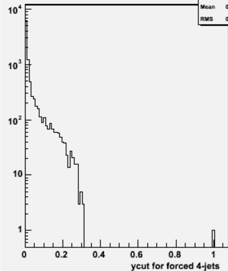
Ycut for 4-jets :w101620 uun2e2e2n2_o
