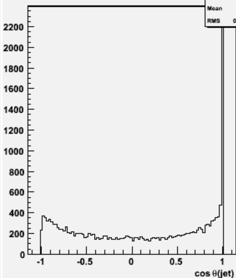
cos \theta for 2-jets :w101620 uun2e2e2n2_o
