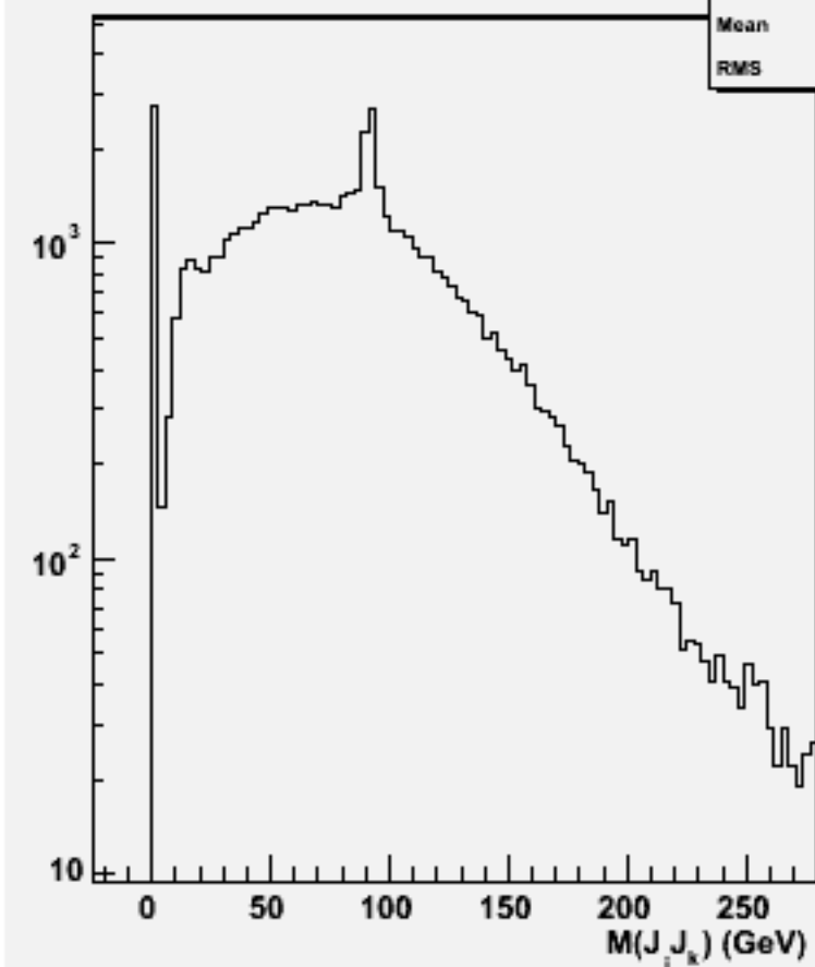
2jets mass(All comb)w101620 uun2e2e2n2_o
