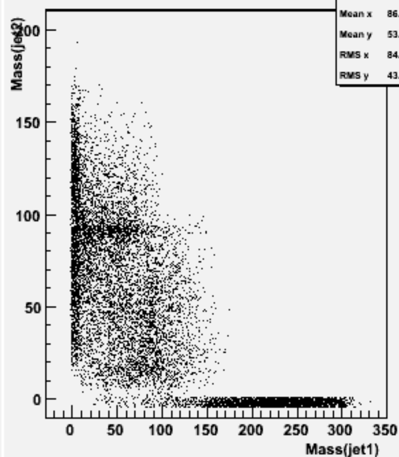
Jet mass for forced 2-jets : w101620 uun2e2e2n2_o
