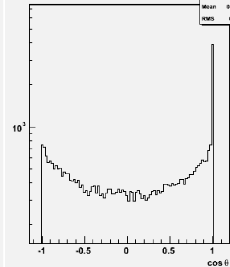
Jet cos \theta (All jets)w101620 uun2e2e2n2_o
