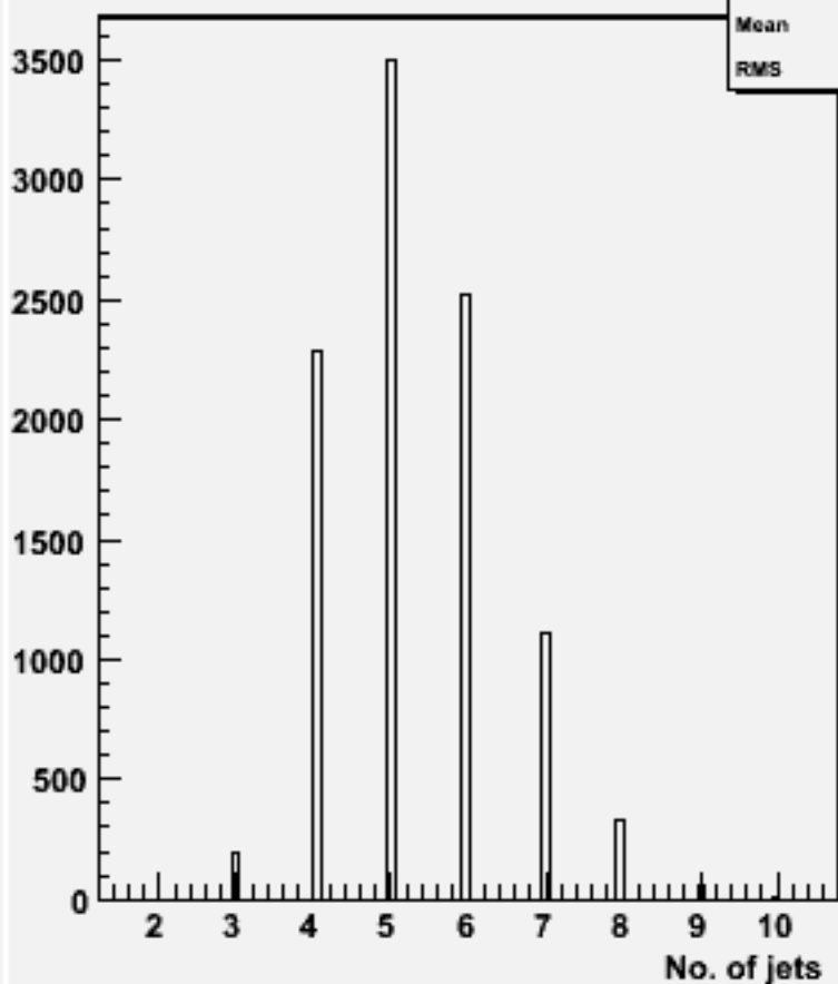
No. jets (ycut=0.001) : w101620 uun2e2e2n2_o
