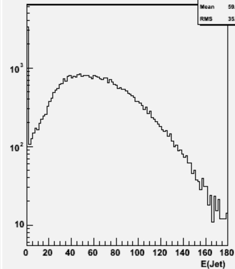
Jet energies(All jets)w101620 uun2e2e2n2_o
