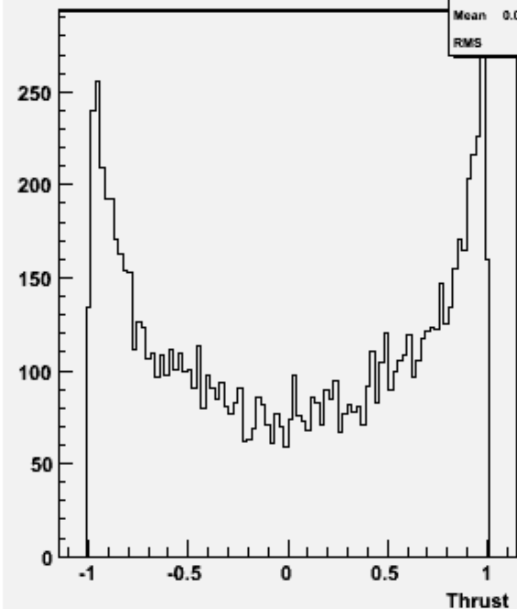
cos \Theta (thrust) w101620 uun2e2e2n2_o
