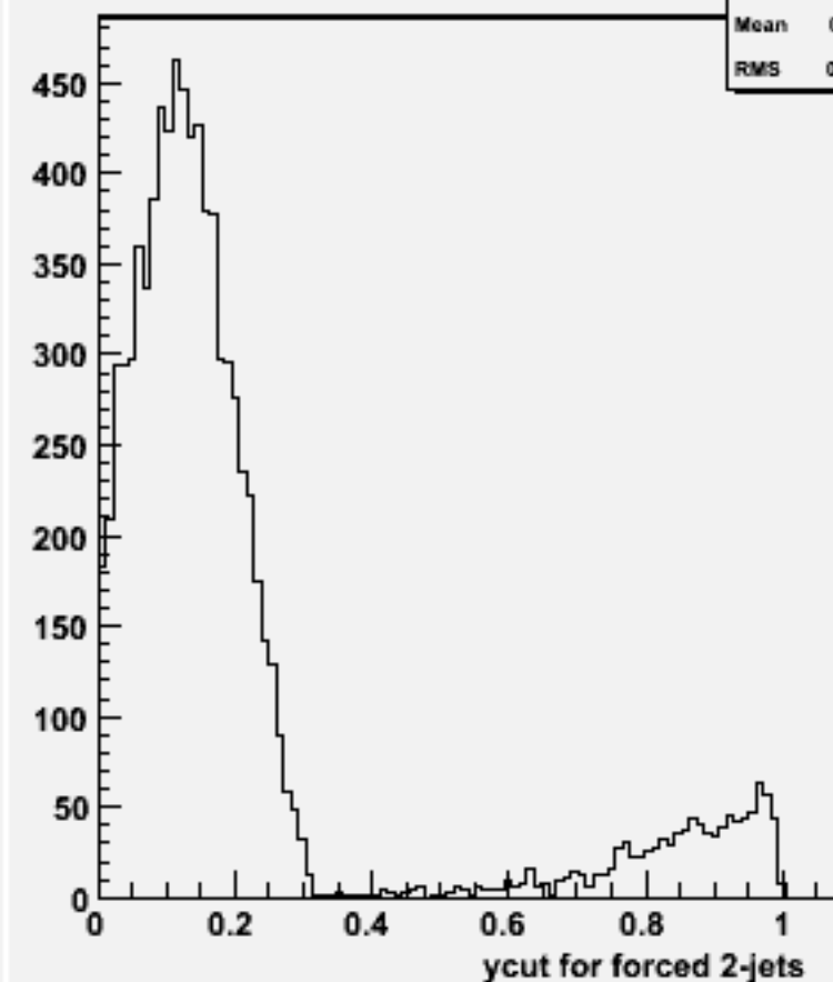
Ycut for 2-jets :w101620 uun2e2e2n2_o
