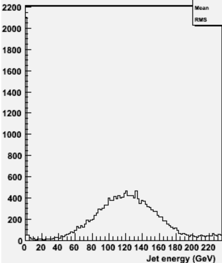
energy for 2-jets :w101620 uun2e2e2n2_o
