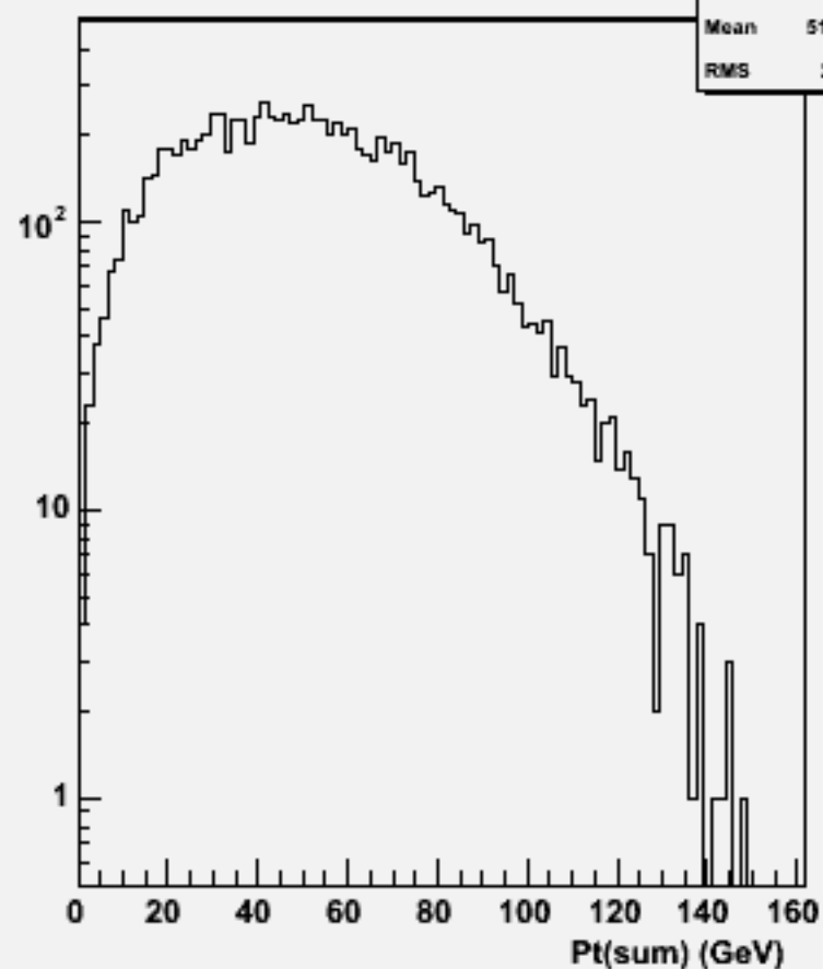
Pt Sum: w101617 uun2e2e1n1_o
