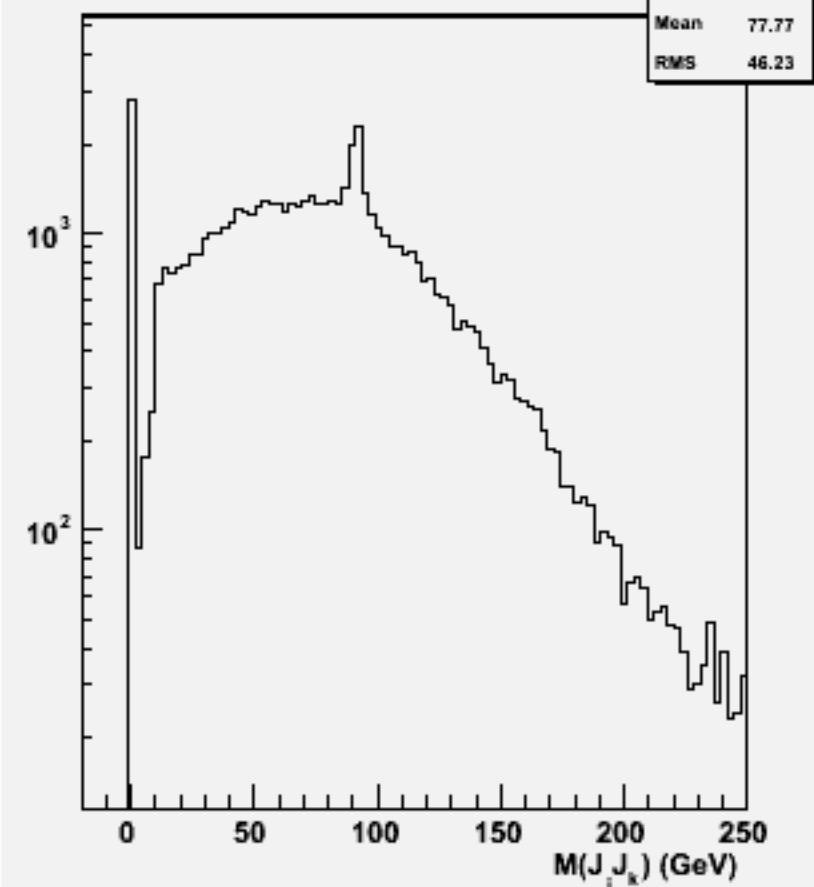
2jets mass(All comb)w101617 uun2e2e1n1_o
