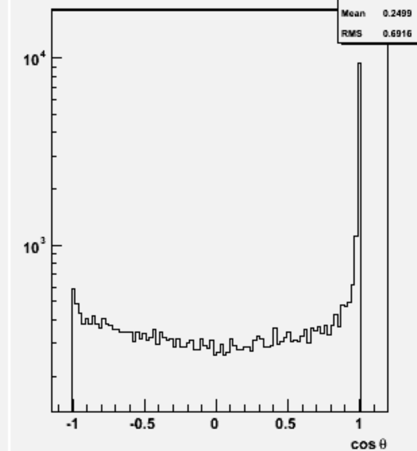
Jet cos \theta (All jets)w101616 uun2e2e1n1_o
