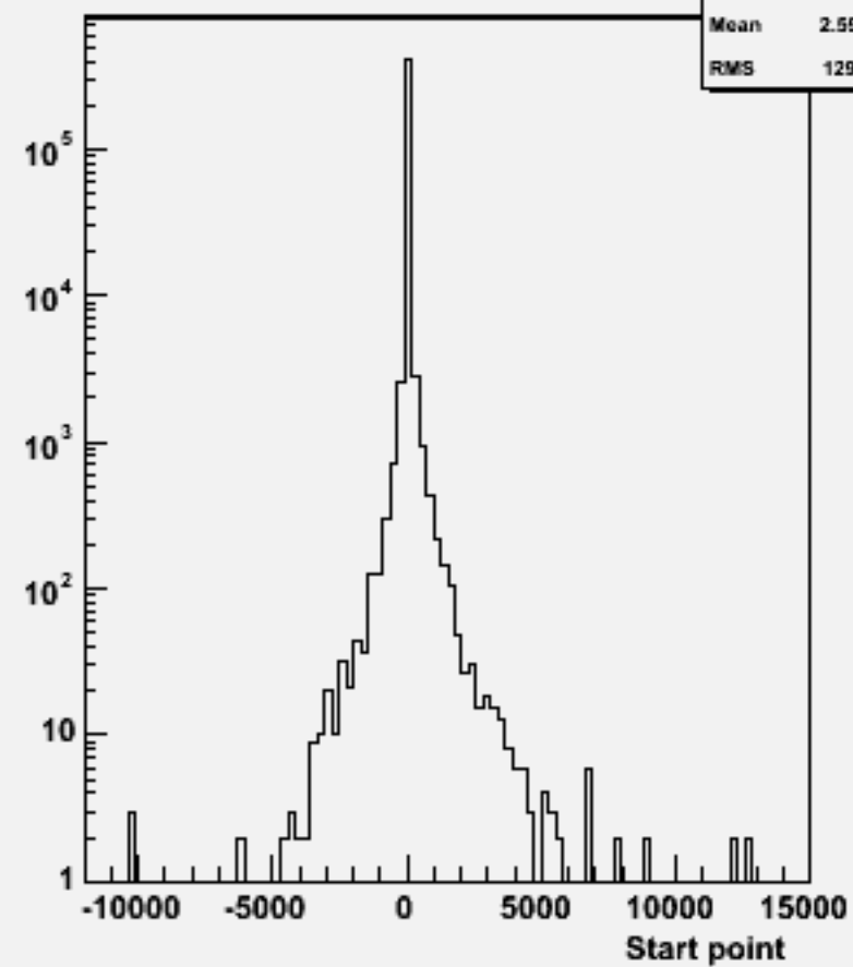
Start point Z : w101616 uun2e2e1n1_o
