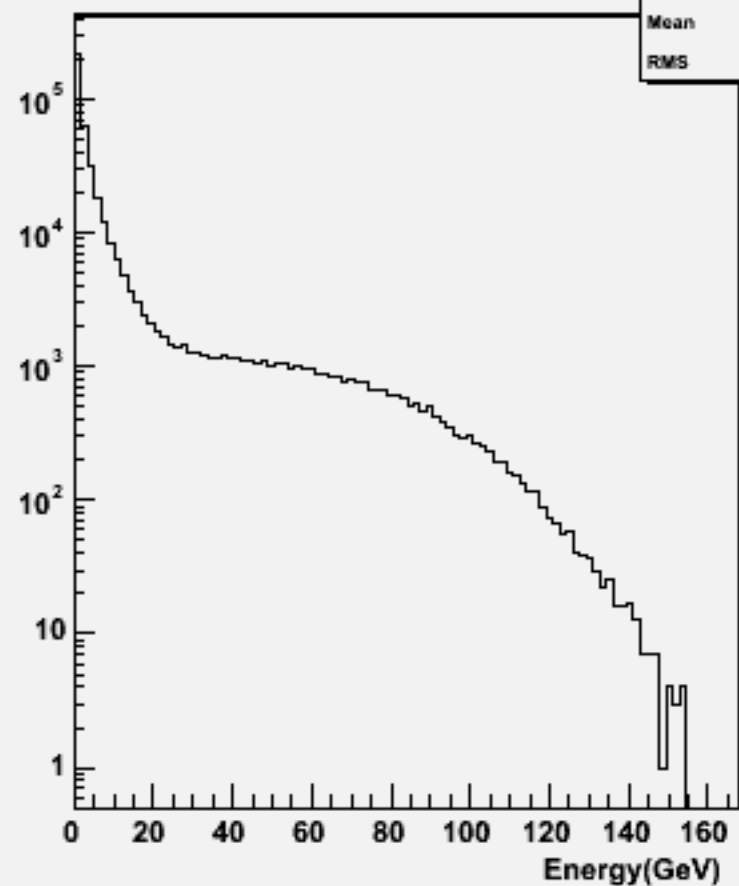
Particle Energy : w101616 uun2e2e1n1_o
