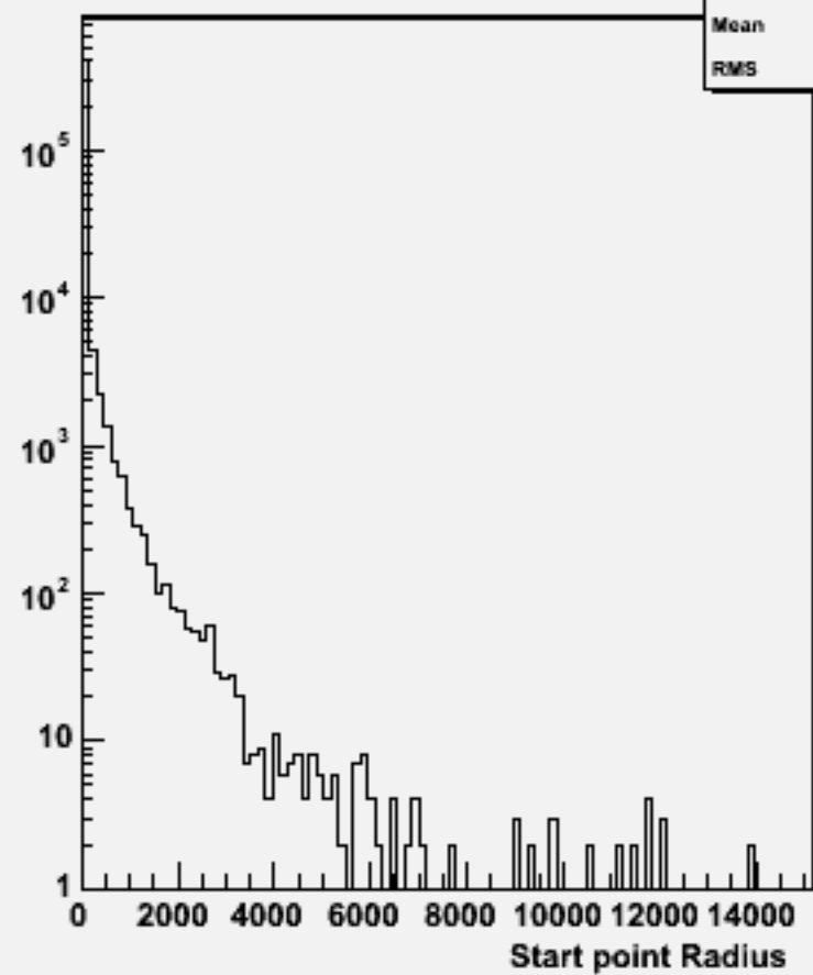
Start point R : w101616 uun2e2e1n1_o
