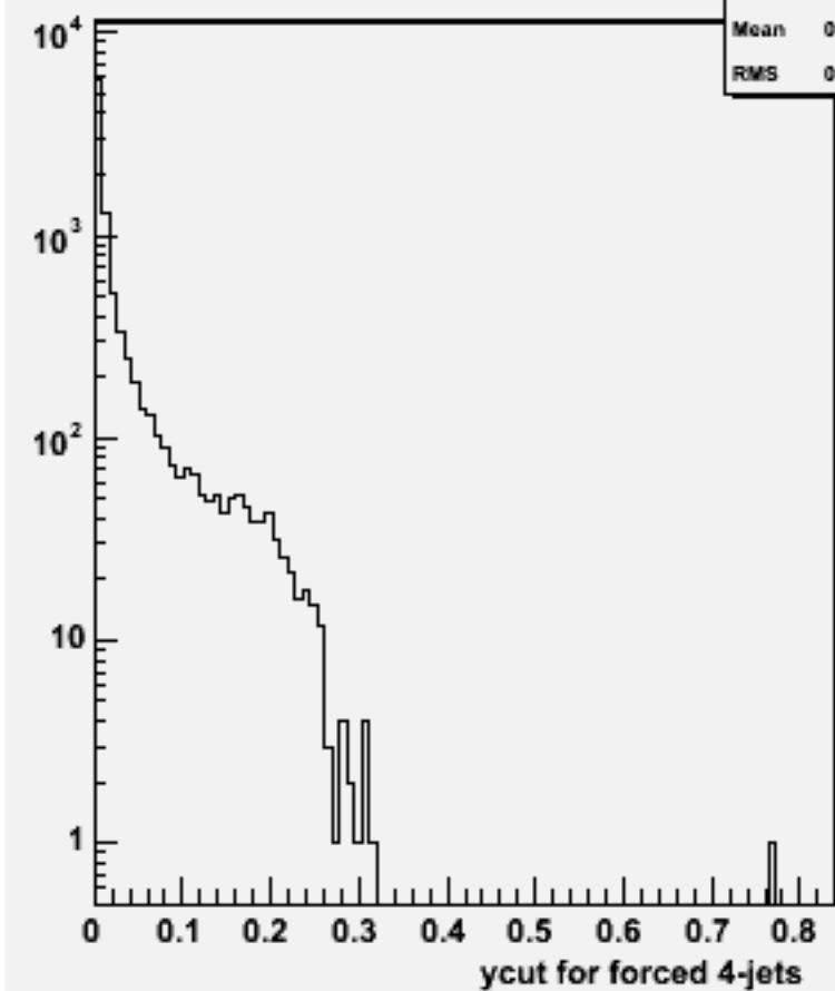
Ycut for 4-jets :w101616 uun2e2e1n1_o
