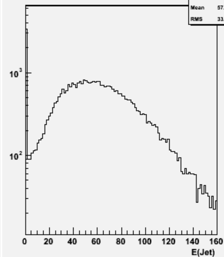
Jet energies(All jets)w101616 uun2e2e1n1_o
