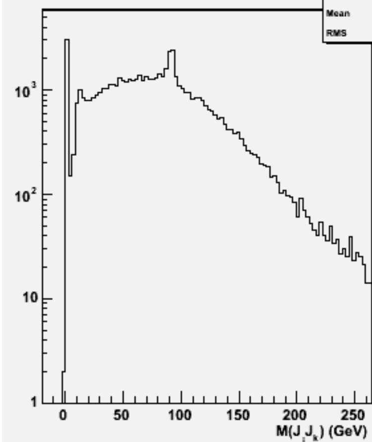
2jets mass(All comb)w101616 uun2e2e1n1_o
