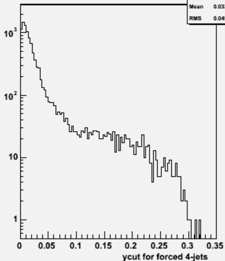
Ycut for 4-jets :w101613 uun1e1sc_o
