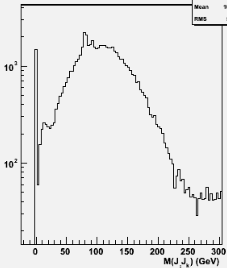
2jets mass(All comb)w101613 uun1e1sc_o
