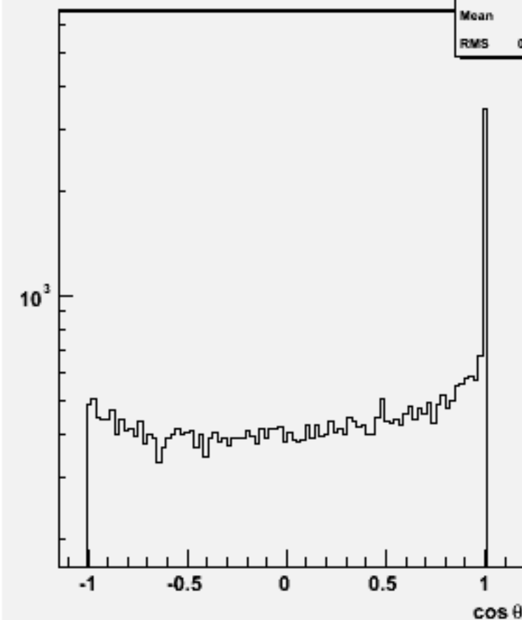
Jet cos \theta (All jets)w101613 uun1e1sc_o
