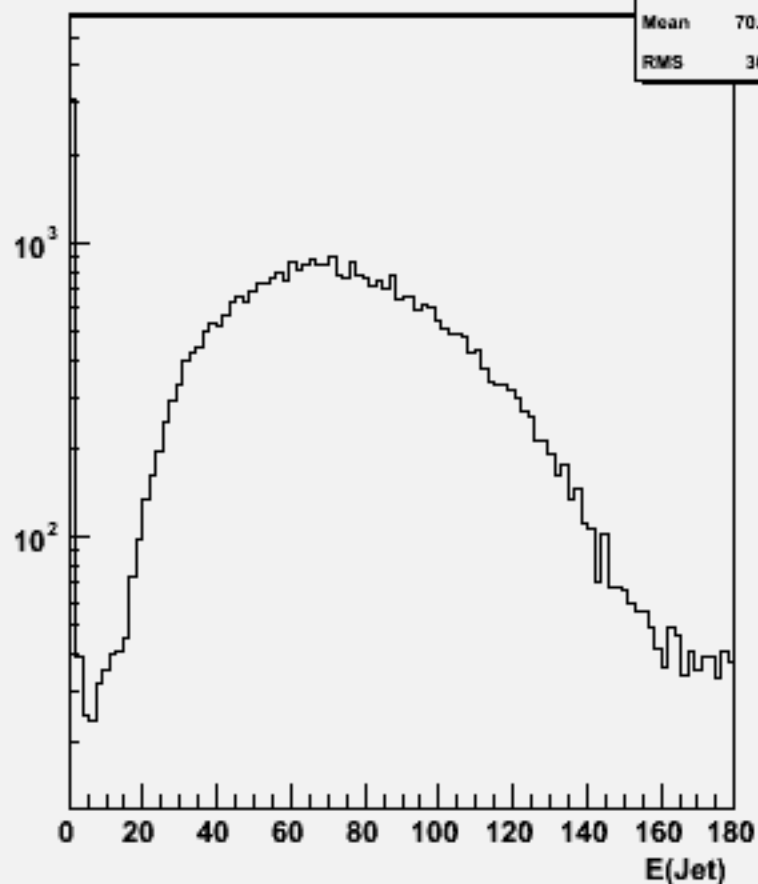
Jet energies(All jets)w101613 uun1e1sc_o
