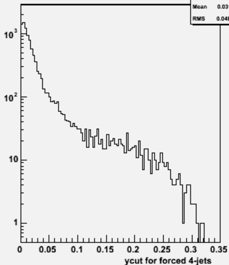
Ycut for 4-jets :w101612 uun1e1sc_o
