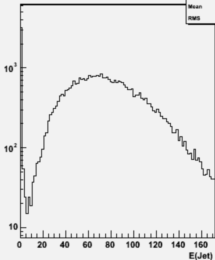
Jet energies(All jets)w101612 uun1e1sc_o
