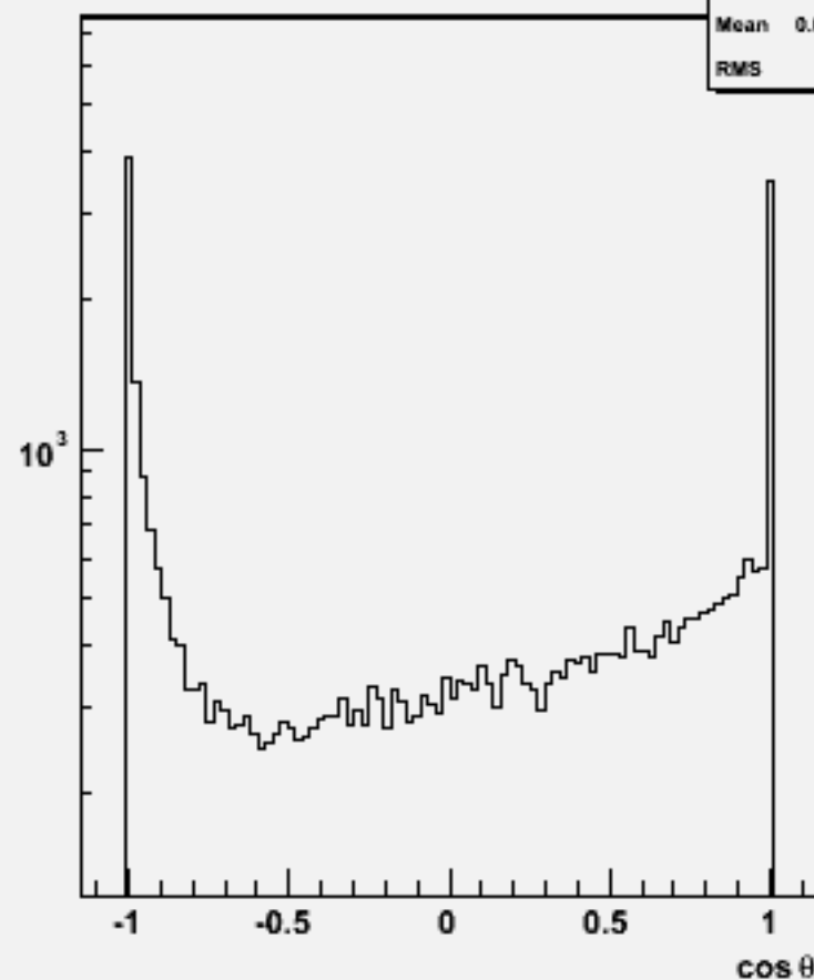
Jet cos \theta (All jets)w101612 uun1e1sc_o
