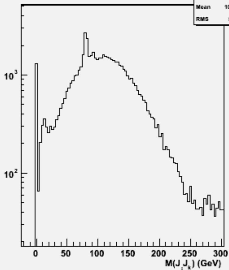
2jets mass(All comb)w101612 uun1e1sc_o
