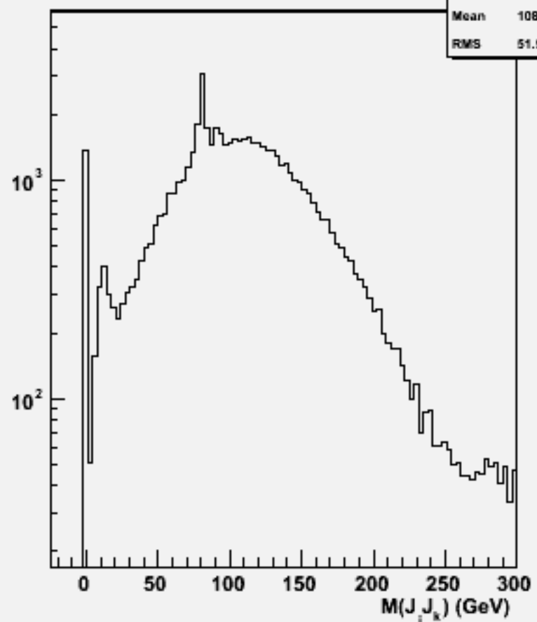
2jets mass(All comb)w101611 uun1e1sc_o
