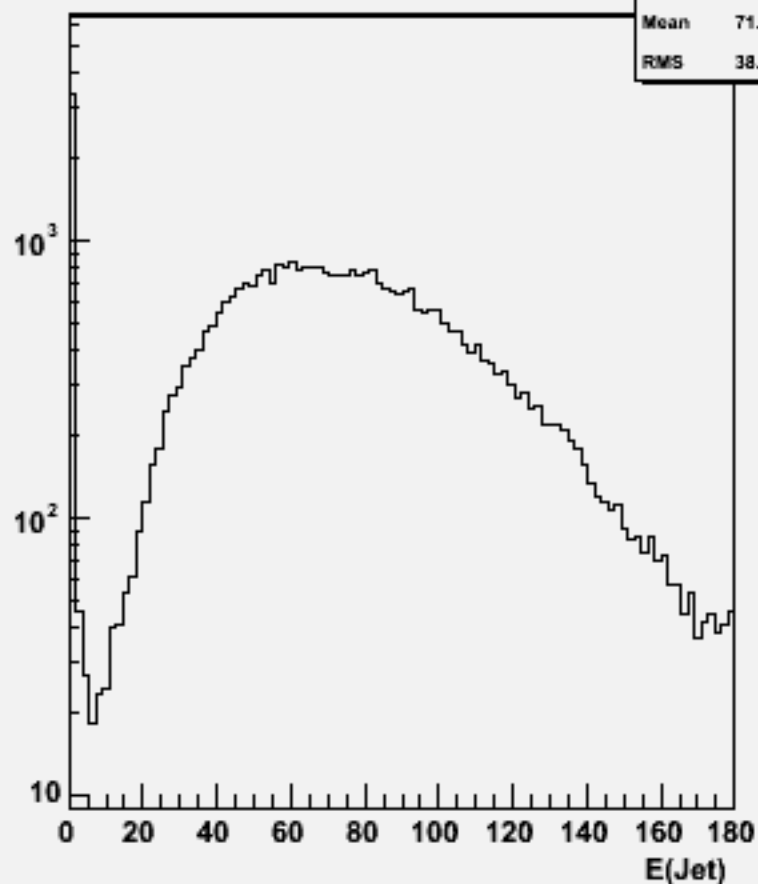
Jet energies(All jets)w101611 uun1e1sc_o
