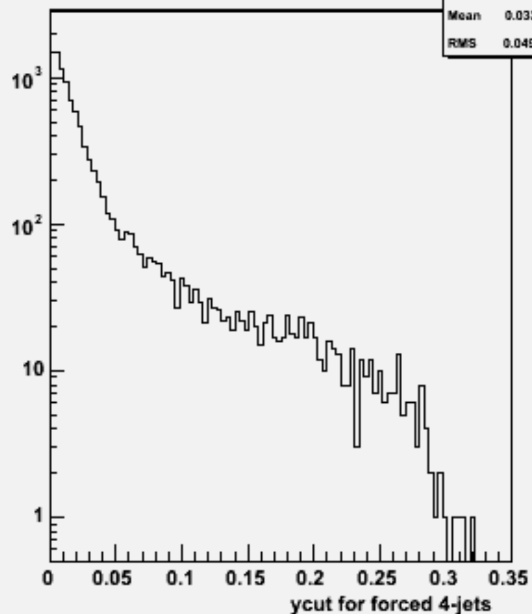
Ycut for 4-jets :w101611 uun1e1sc_o
