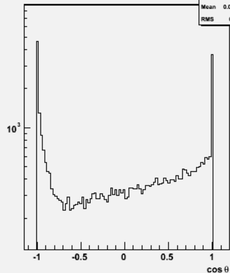
Jet cosθ (All jets)w101611 uun1e1sc_o
