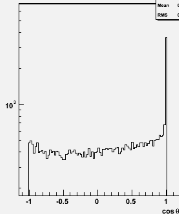
Jet cosθ (All jets)w101609 uun1e1du_o
