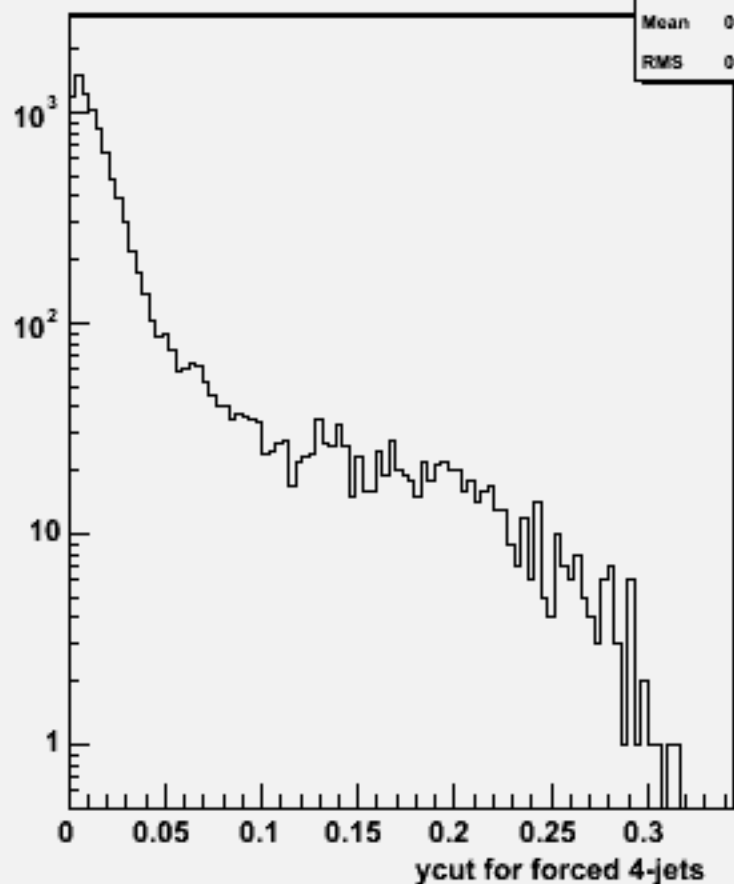
Ycut for 4-jets :w101609 uun1e1du_o
