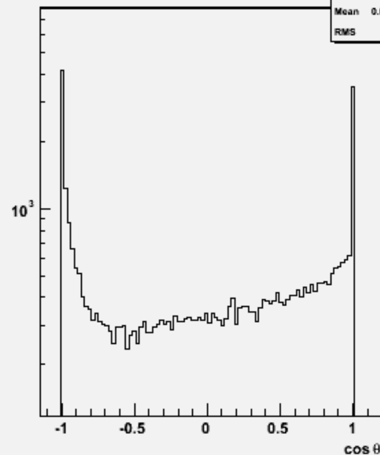
Jet cosθ (All jets)w101608 uun1e1du_o
