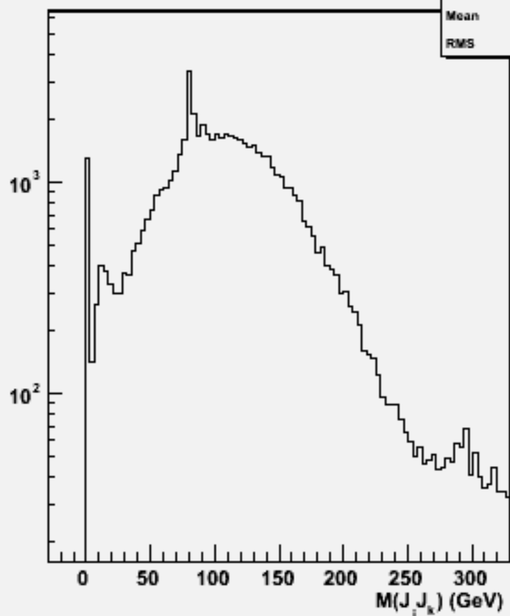
2jets mass(All comb)w101608 uun1e1du_o
