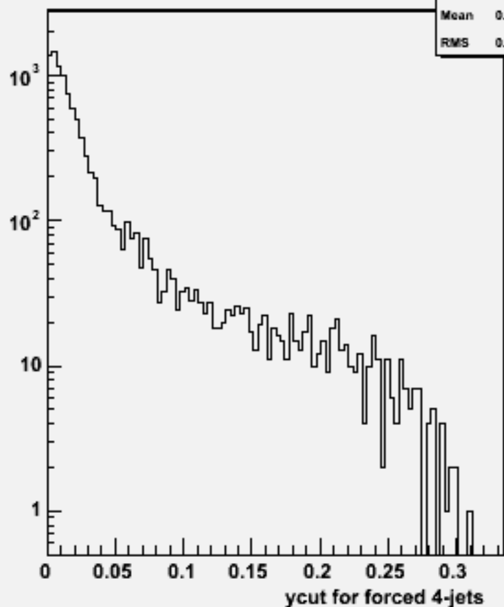
Ycut for 4-jets :w101608 uun1e1du_o
