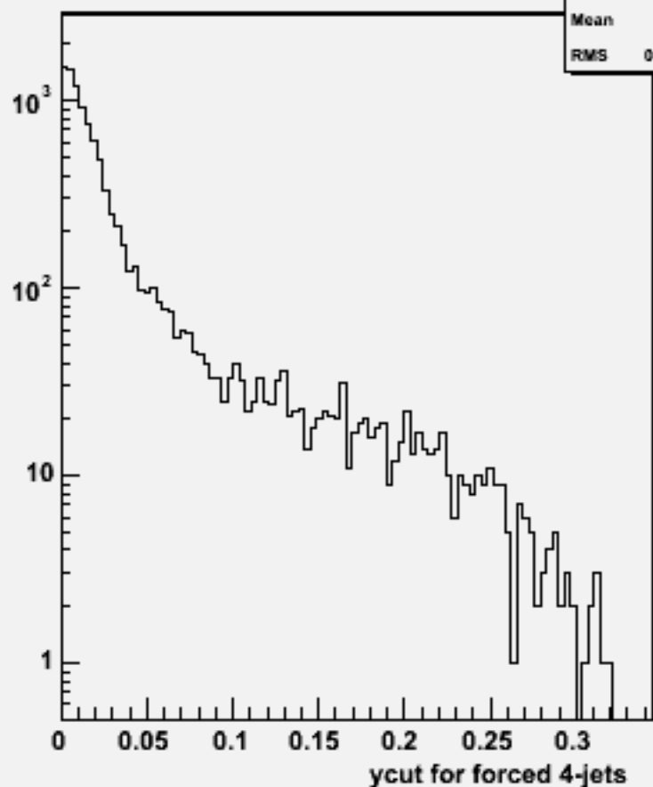
Ycut for 4-jets :w101607 uun1e1du_o
