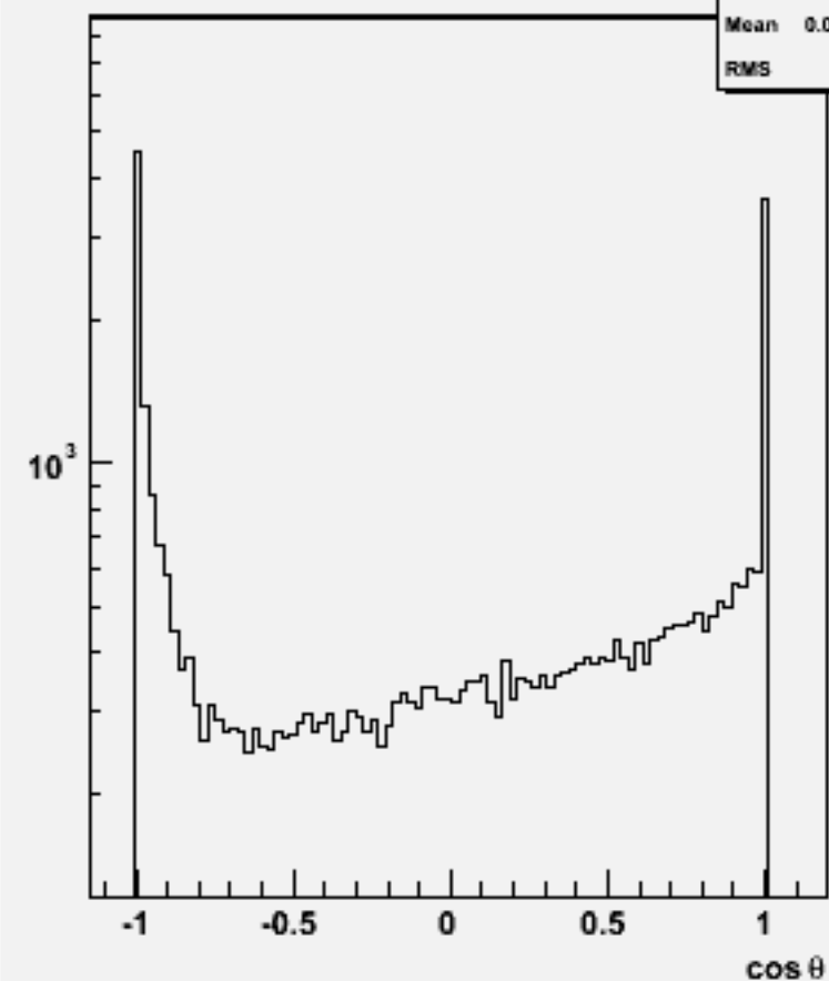
Jet cos \theta (All jets)w101607 uun1e1du_o
