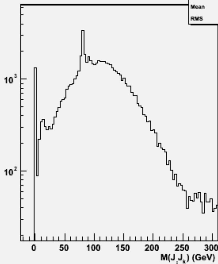
2jets mass(All comb)w101607 uun1e1du_o
