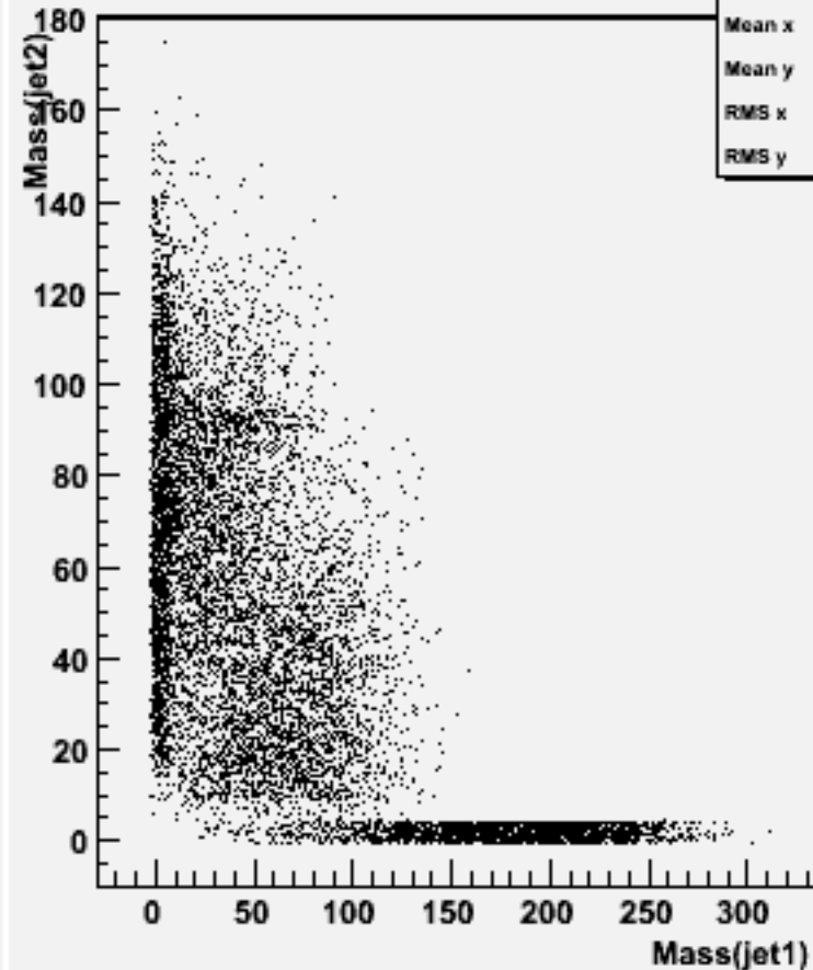
Jet mass for forced 2-jets : w101605 uun1e1e3n3_o
