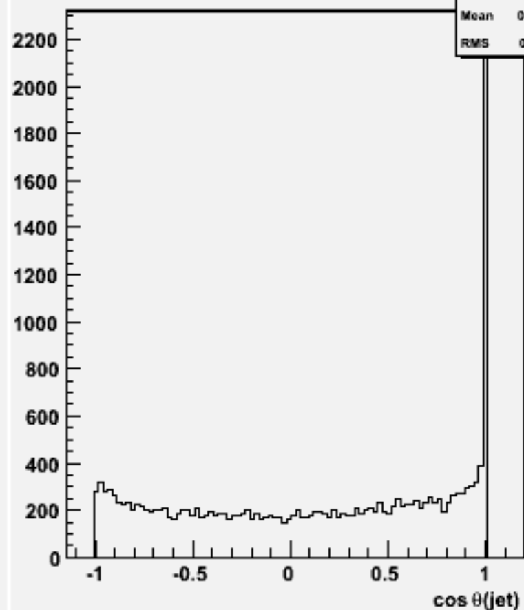
cos \theta for 2-jets :w101605 uun1e1e3n3_o
