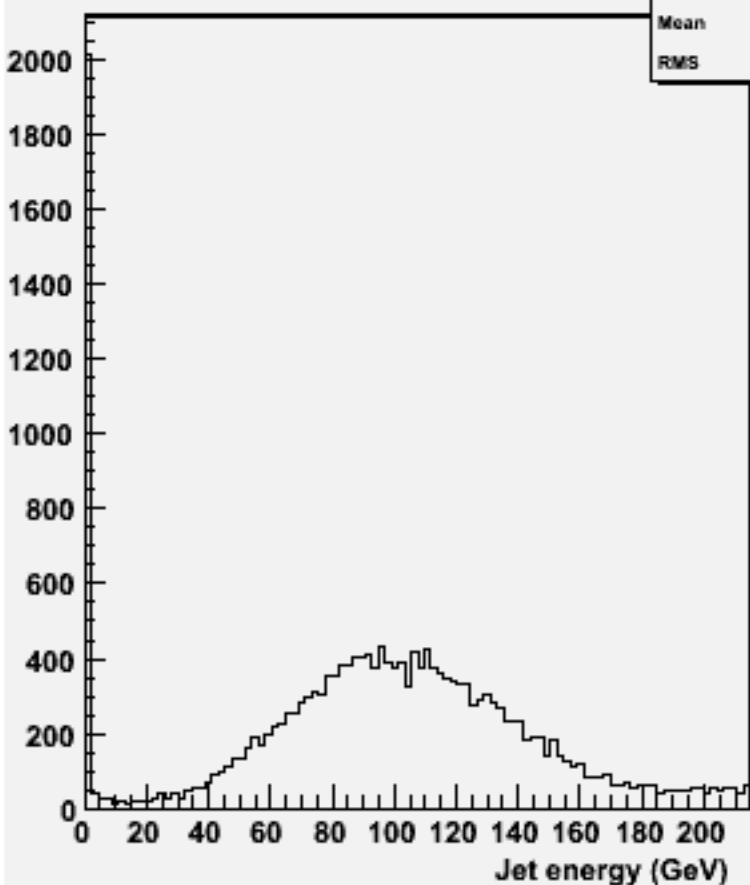
energy for 2-jets :w101605 uun1e1e3n3_o
