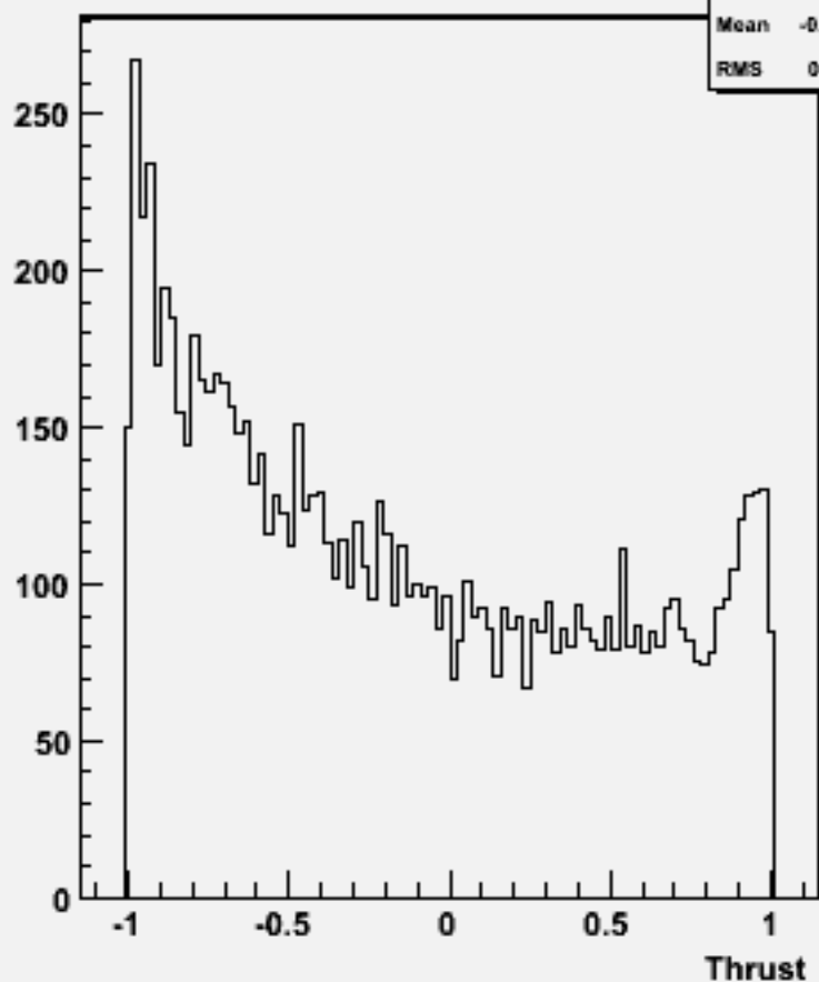
cos \Theta (thrust) w101605 uun1e1e3n3_o
