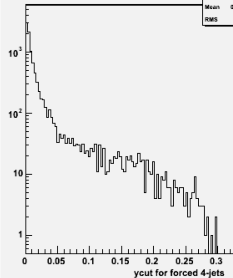
Ycut for 4-jets :w101605 uun1e1e3n3_o
