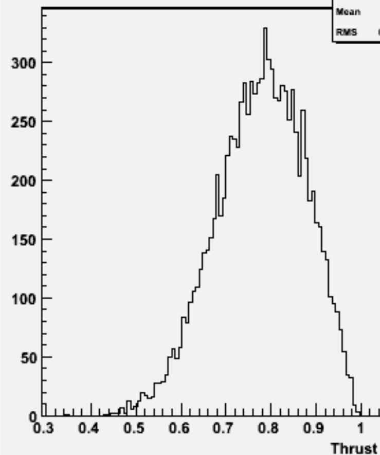
Thrust w101605 uun1e1e3n3_o
