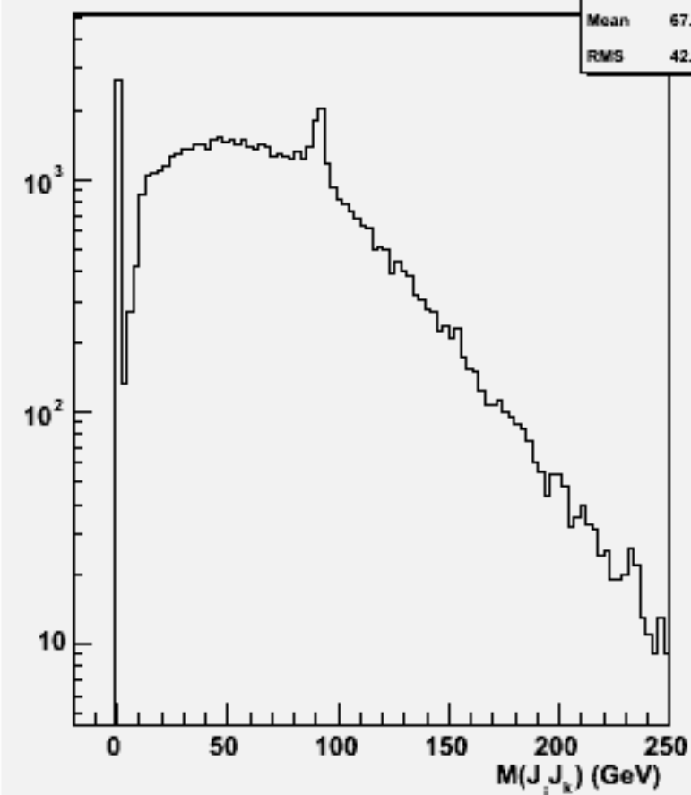
2jets mass(All comb)w101605 uun1e1e3n3_o
