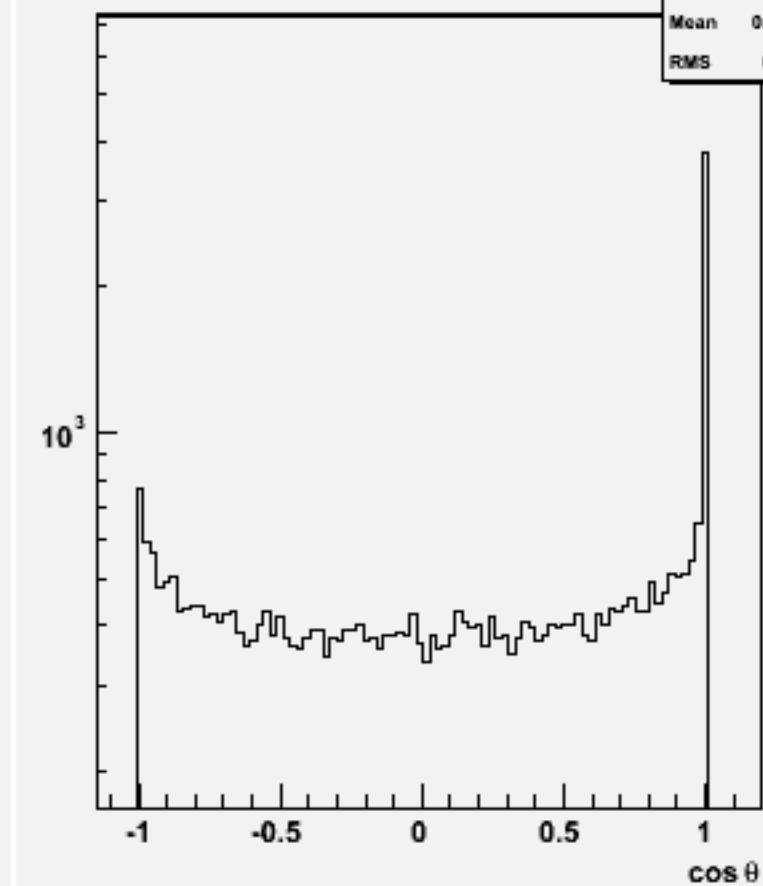
Jet cos \theta (All jets)w101605 uun1e1e3n3_o
