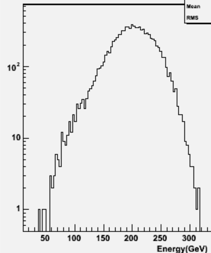
Thrust w101605 uun1e1e3n3_o
