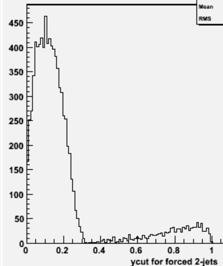
Ycut for 2-jets :w101605 uun1e1e3n3_o
