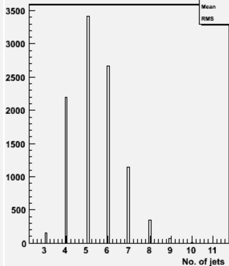
No. jets (ycut=0.001) : w101605 uun1e1e3n3_o
