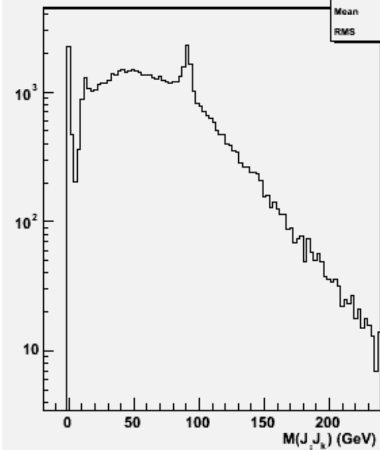
2jets mass(All comb)w101603 uun1e1e3n3_o
