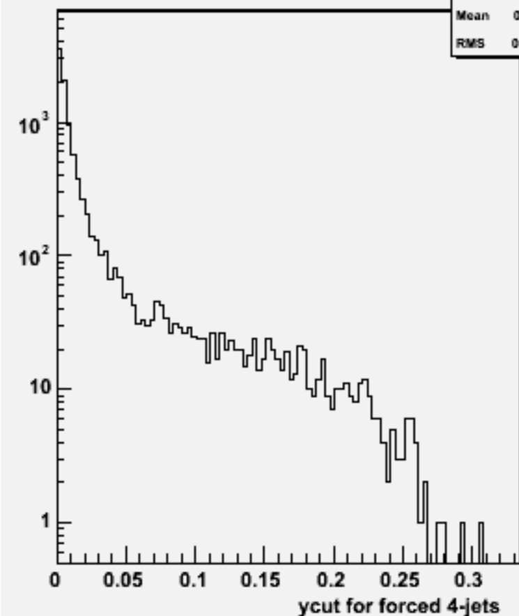
Ycut for 4-jets :w101603 uun1e1e3n3_o
