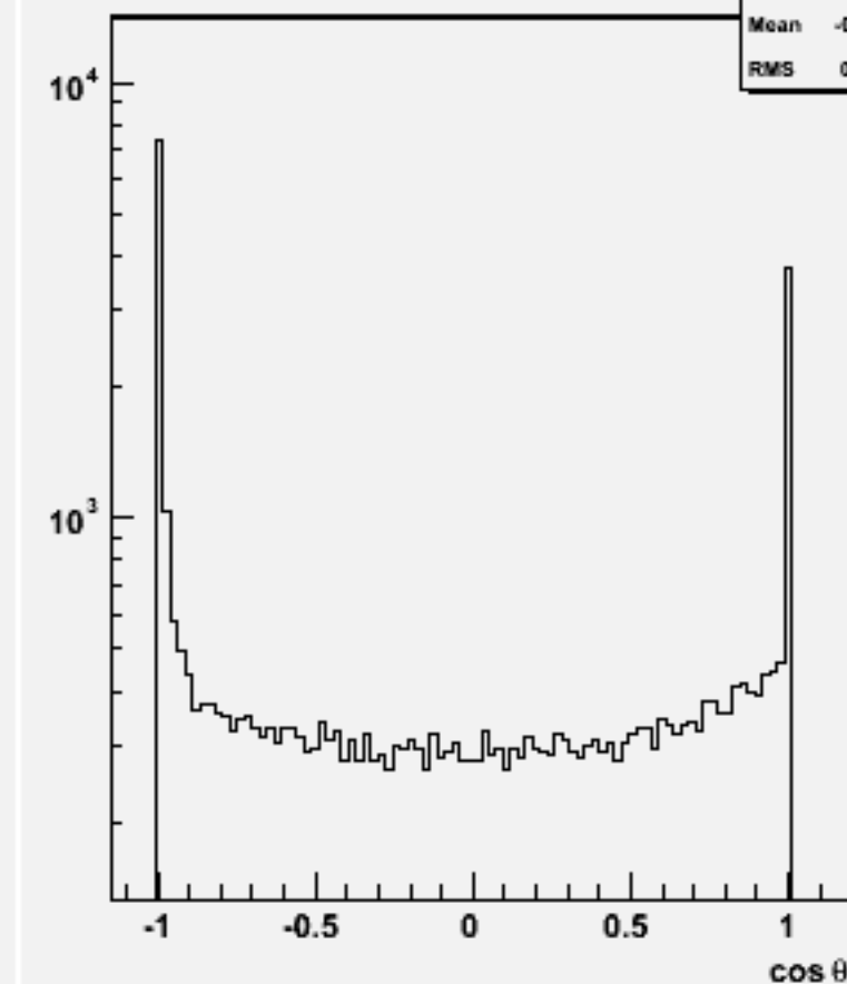
Jet cos \theta (All jets)w101603 uun1e1e3n3_o
