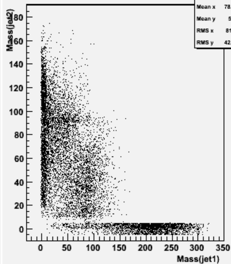
Jet mass for forced 2-jets : w101598 uun1e1e1n1_o
