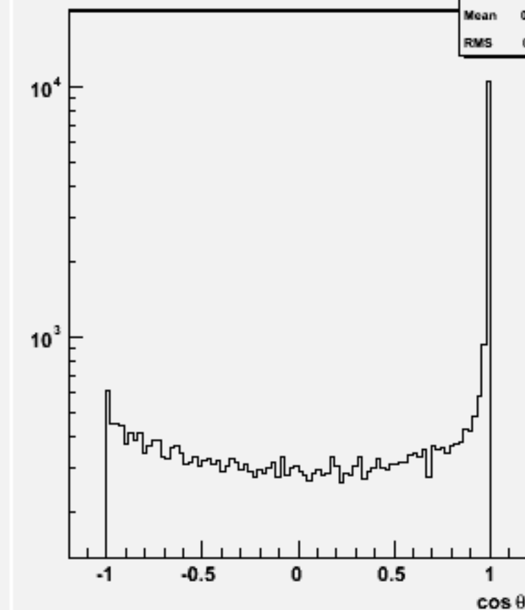
Jet cos \theta (All jets)w101598 uun1e1e1n1_o
