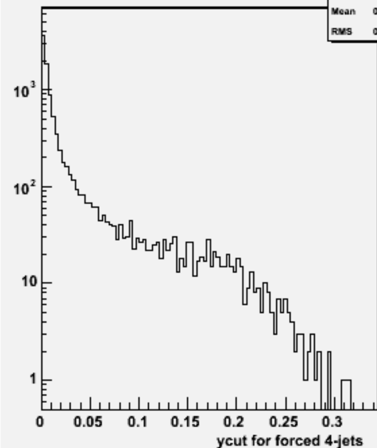
Ycut for 4-jets :w101598 uun1e1e1n1_o
