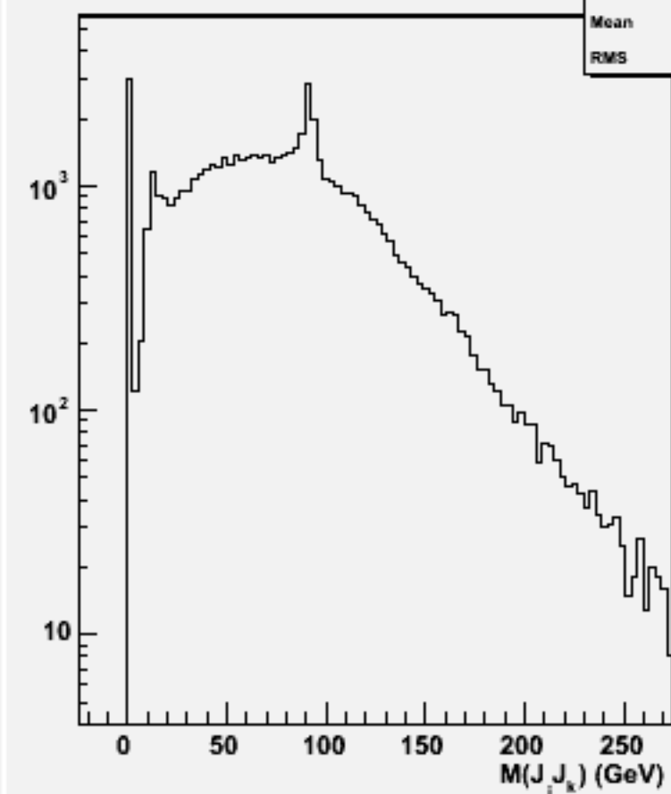
2jets mass(All comb)w101598 uun1e1e1n1_o
