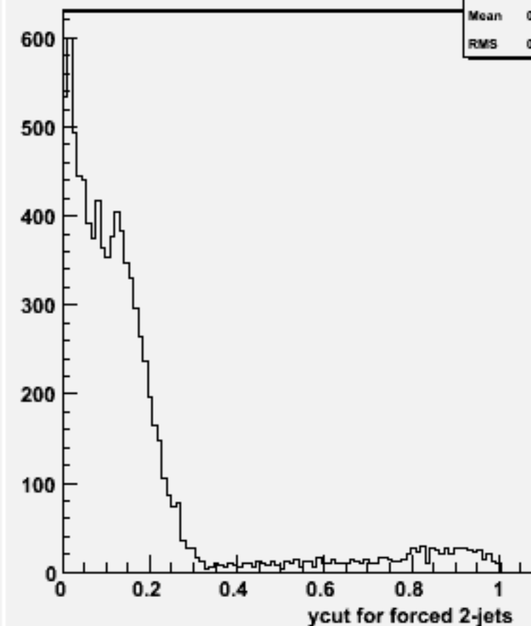
Ycut for 2-jets :w101597 uun1e1e1n1_o
