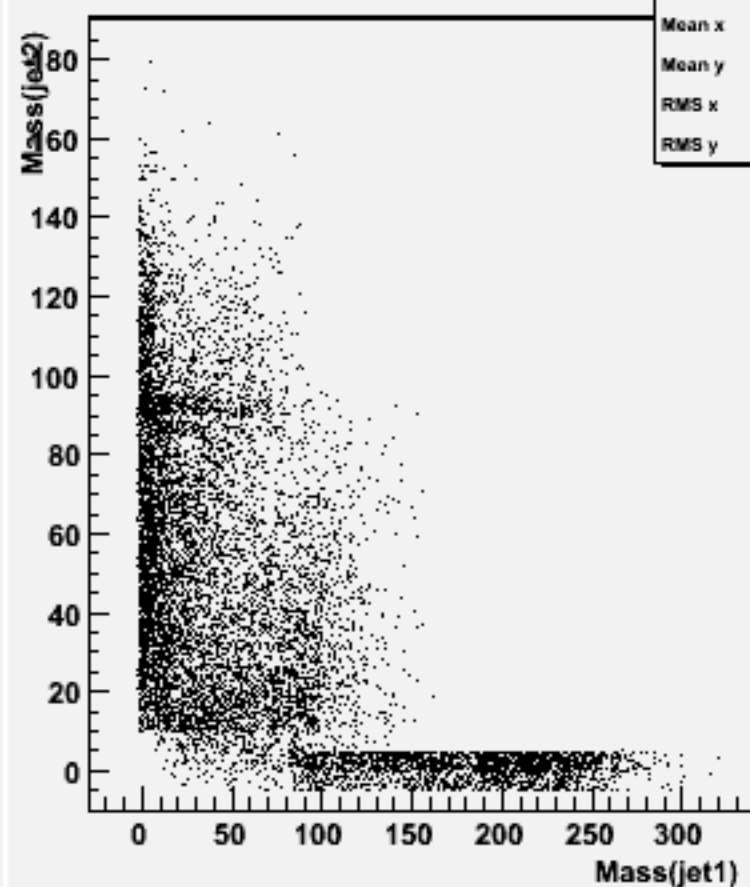
Jet mass for forced 2-jets : w101597 uun1e1e1n1_o
