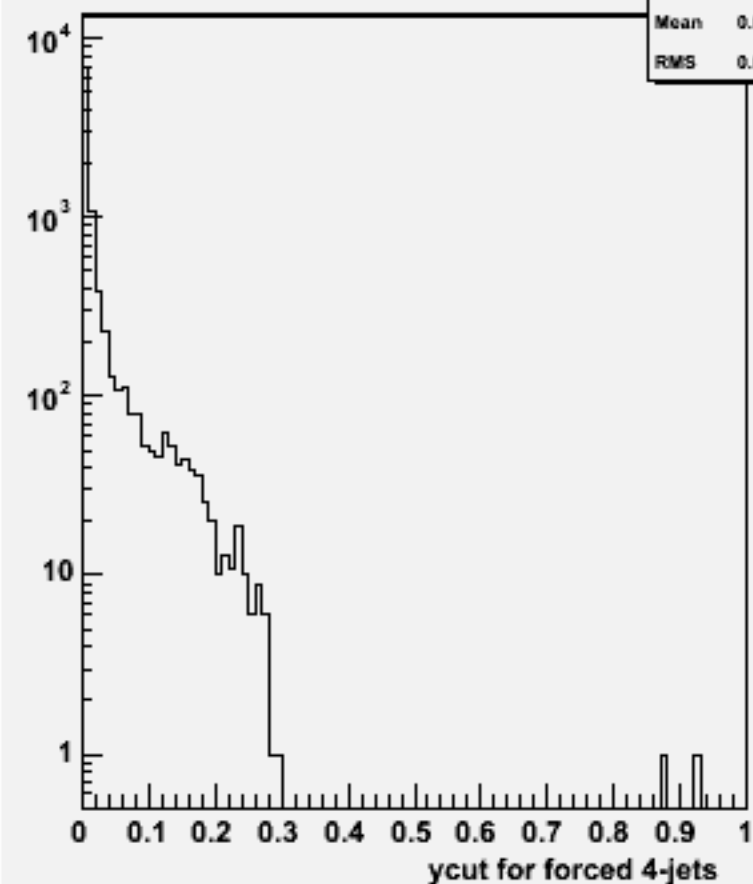
Ycut for 4-jets :w101597 uun1e1e1n1_o
