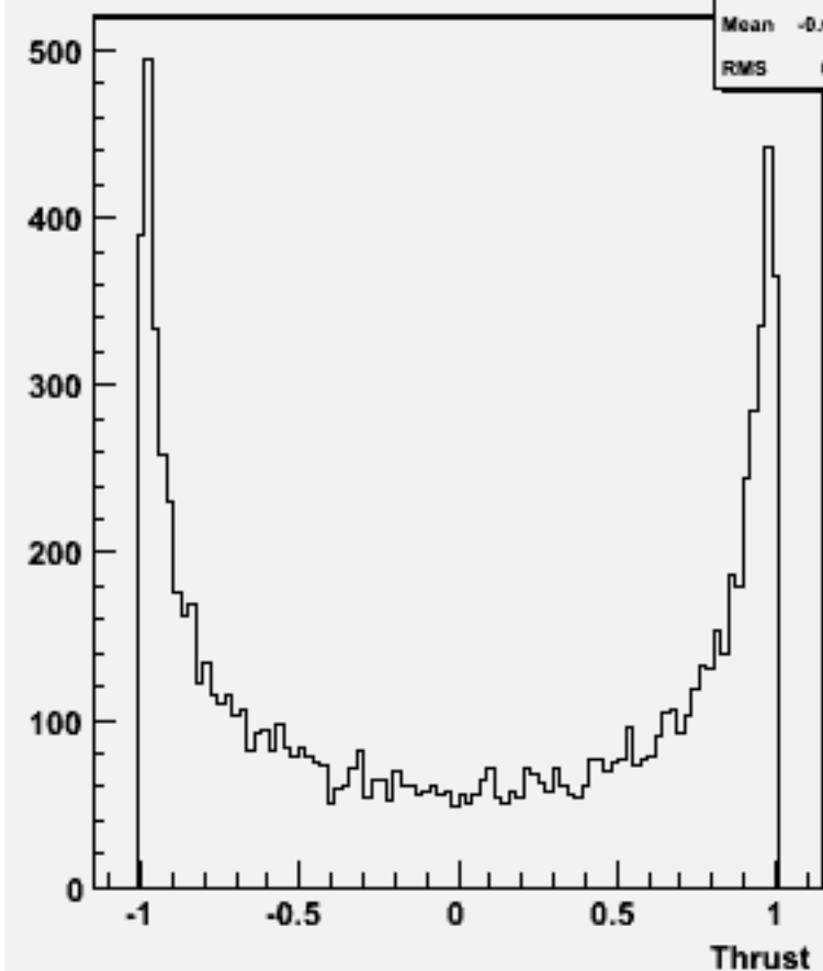
cos \Theta (thrust) w101597 uun1e1e1n1_o
