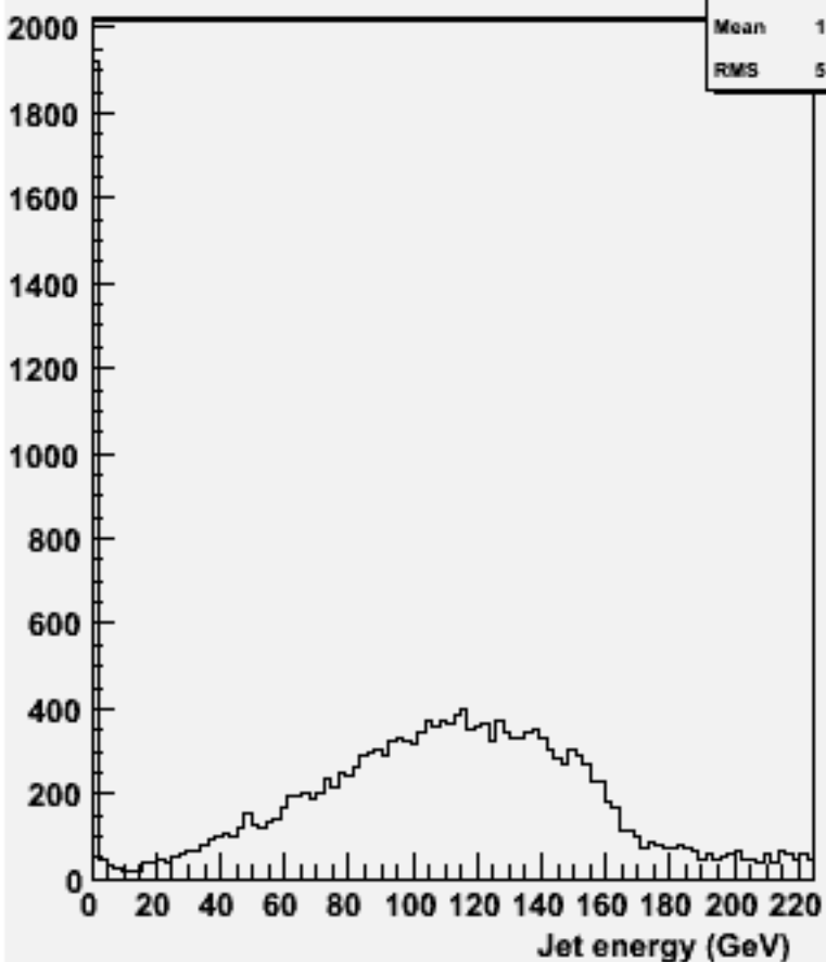
energy for 2-jets :w101597 uun1e1e1n1_o
