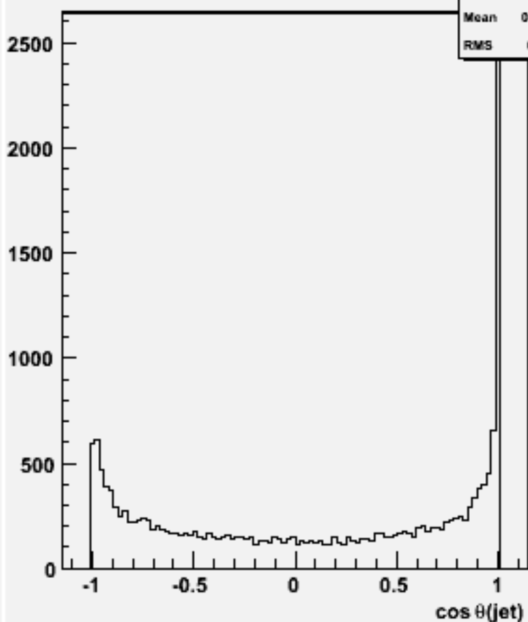
cos \theta for 2-jets :w101597 uun1e1e1n1_o
