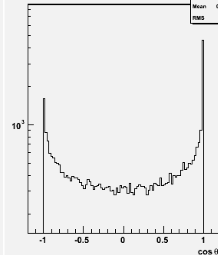
Jet cos \theta (All jets)w101597 uun1e1e1n1_o
