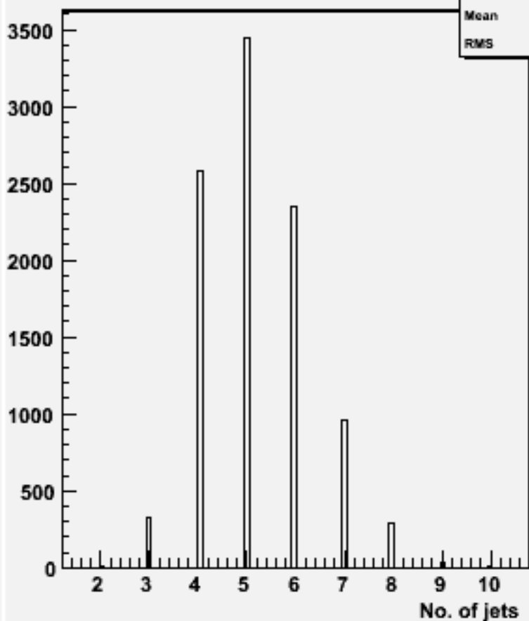
No. jets (ycut=0.001) : w101597 uun1e1e1n1_o
