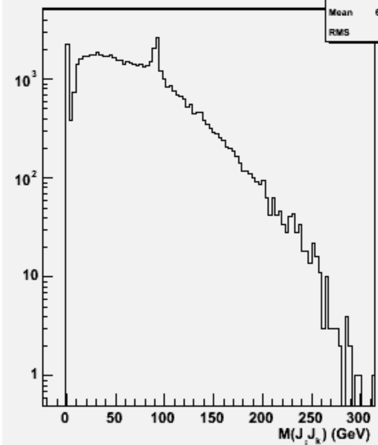
2jets mass(All comb)w101597 uun1e1e1n1_o
