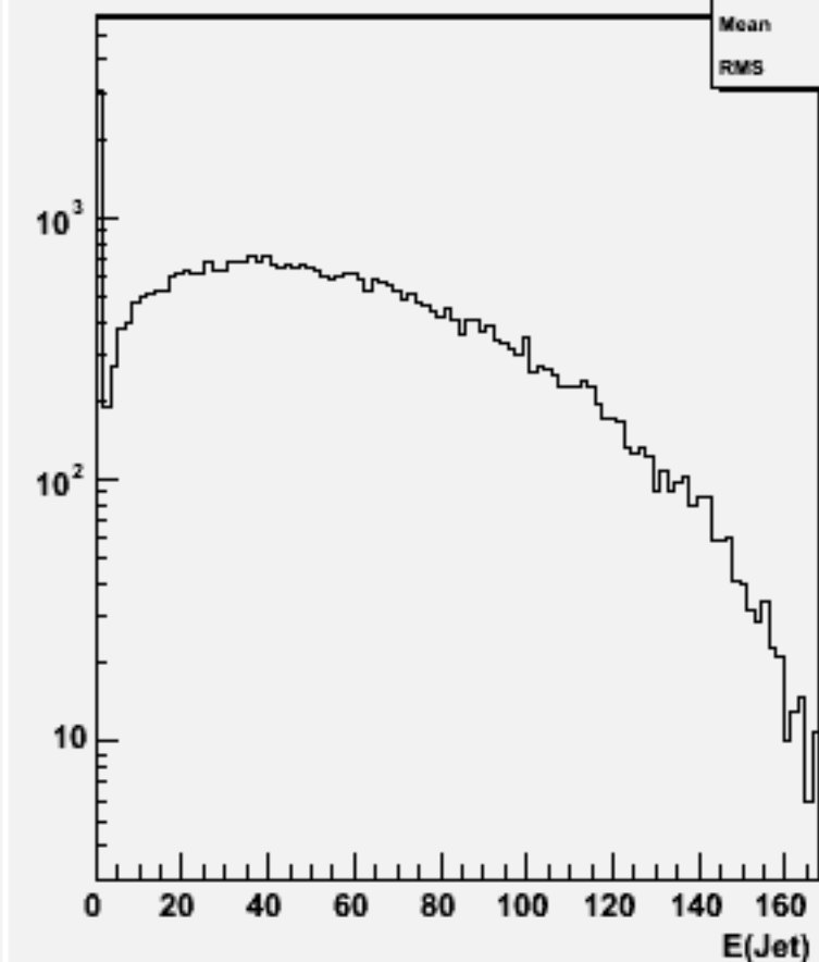
Jet energies(All jets)w101597 uun1e1e1n1_o
