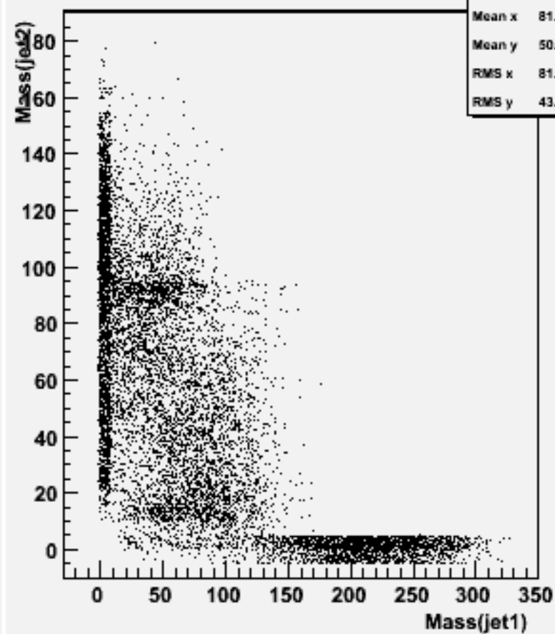
Jet mass for forced 2-jets : w101595 uun1e1e1n1_o
