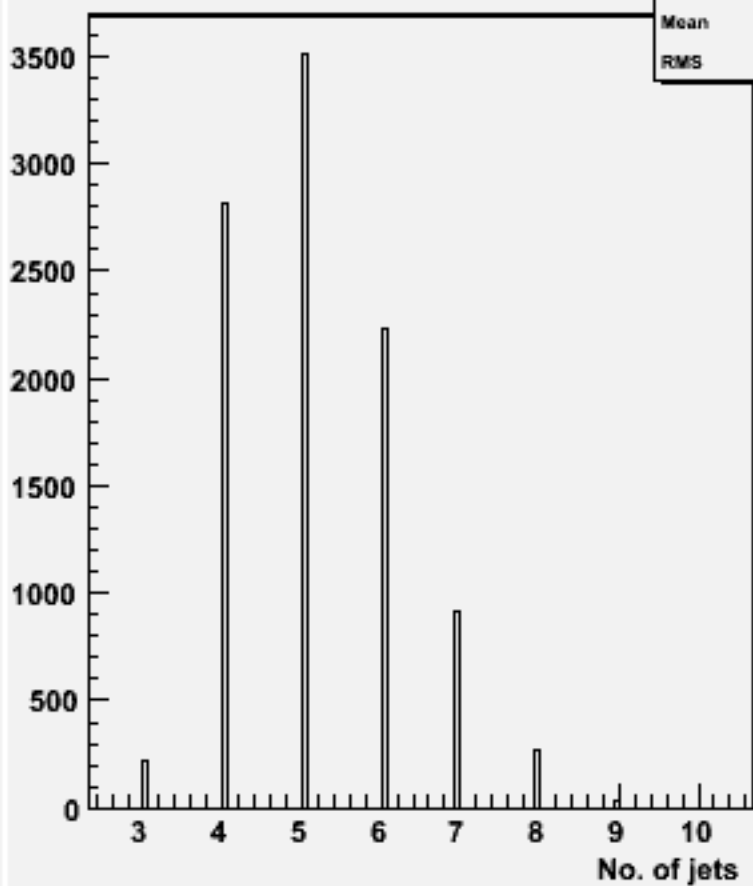
No. jets (ycut=0.001) : w101595 uun1e1e1n1_o
