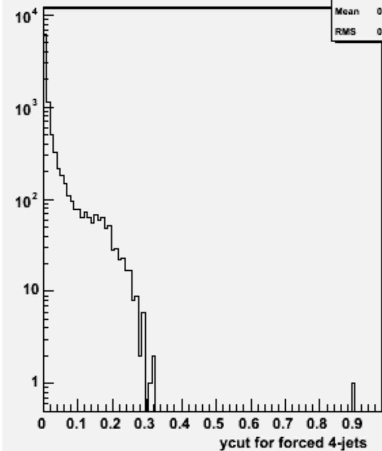
Ycut for 4-jets :w101595 uun1e1e1n1_o
