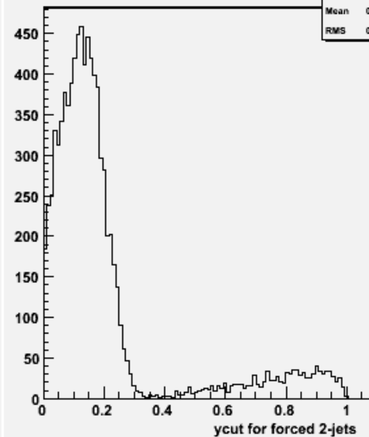
Ycut for 2-jets :w101595 uun1e1e1n1_o
