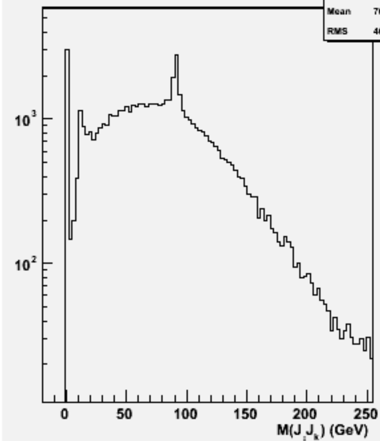
2jets mass(All comb)w101595 uun1e1e1n1_o
