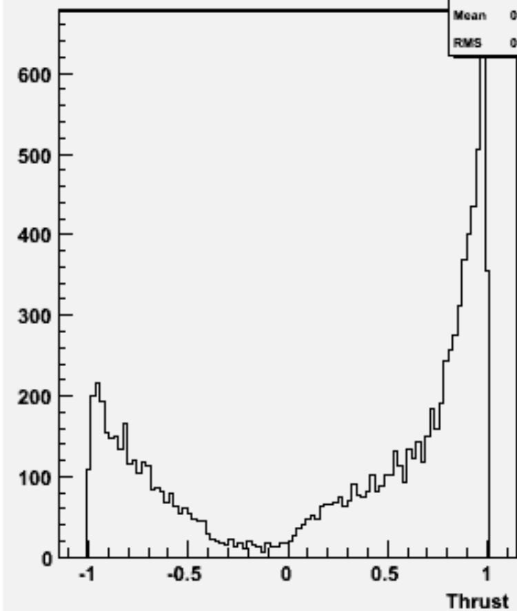
cos \Theta (thrust) w101595 uun1e1e1n1_o
