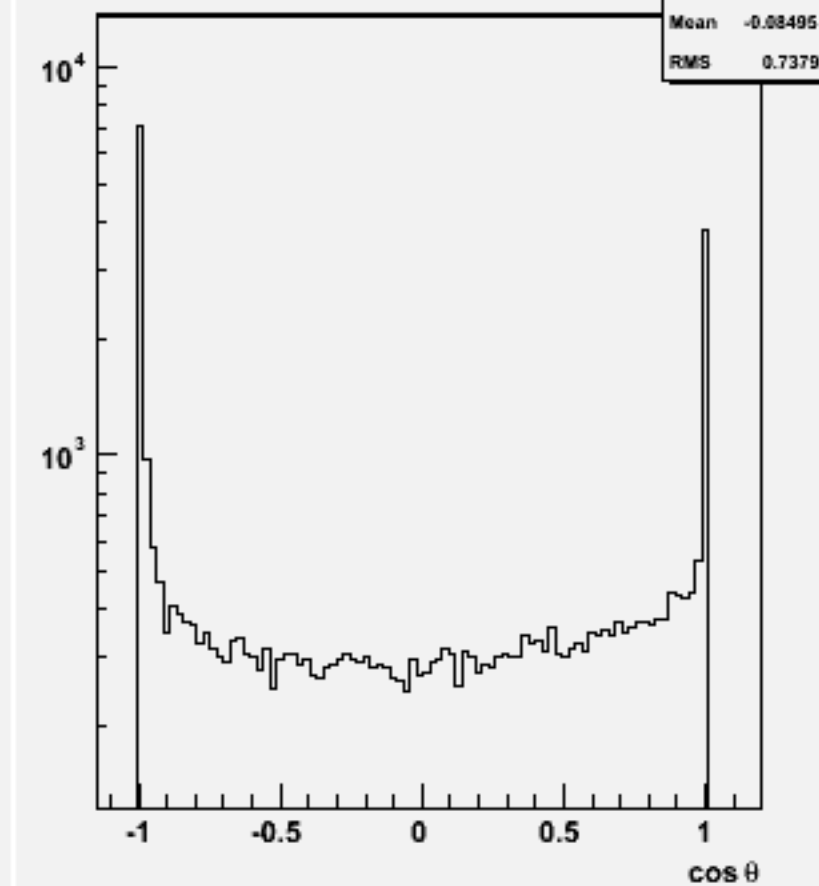
Jet cos \theta (All jets)w101595 uun1e1e1n1_o
