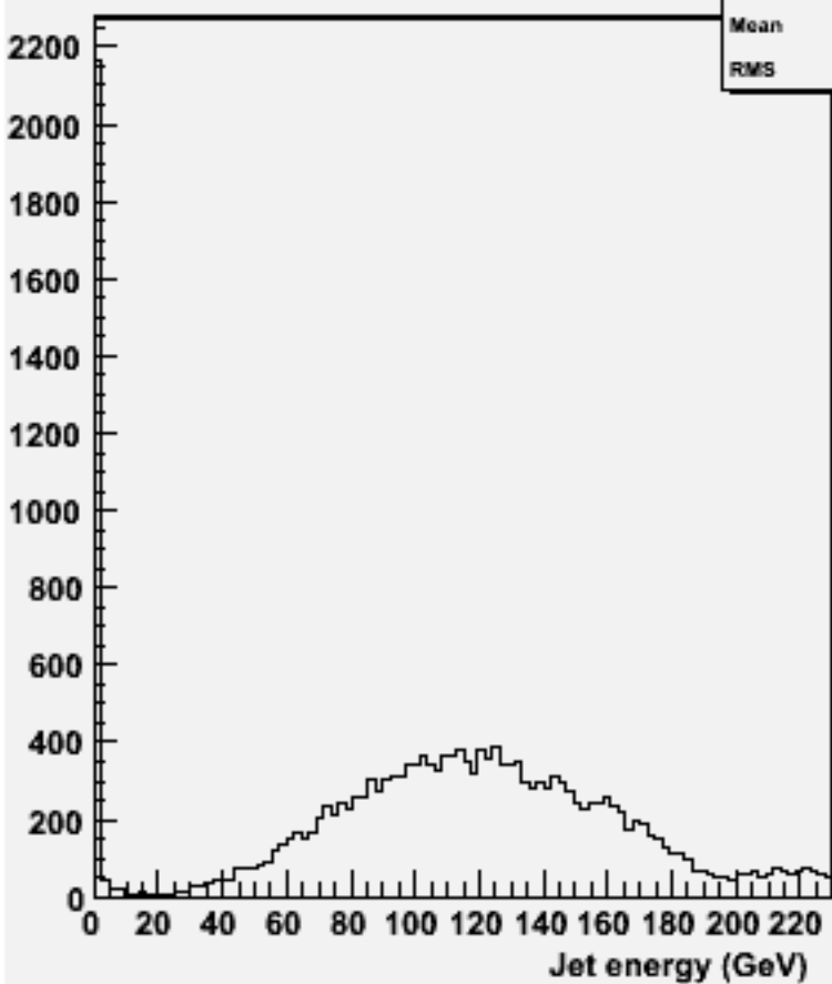
energy for 2-jets :w101595 uun1e1e1n1_o
