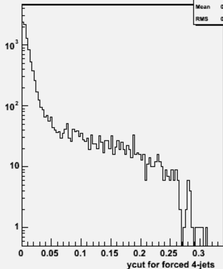
Ycut for 4-jets :w101593 n3n3cssc_o
