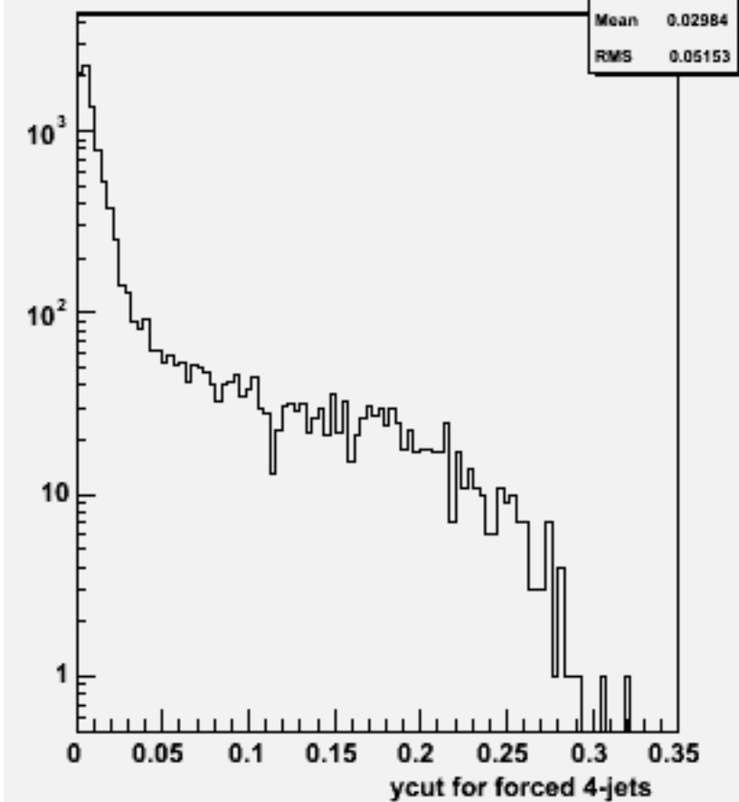
Ycut for 4-jets :w101592 n3n3cssc_o
