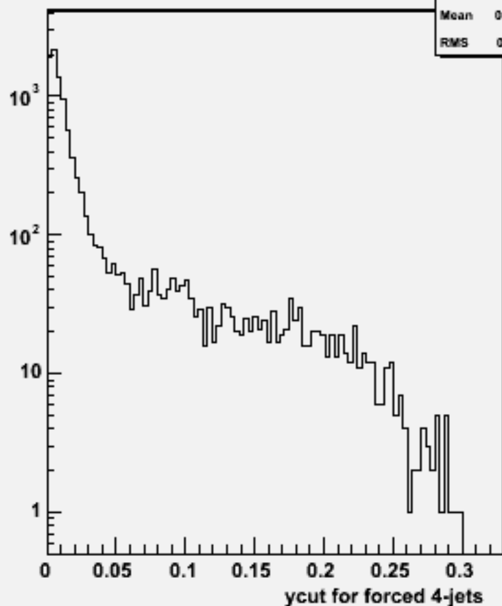
Ycut for 4-jets :w101589 n3n3csdu_o
