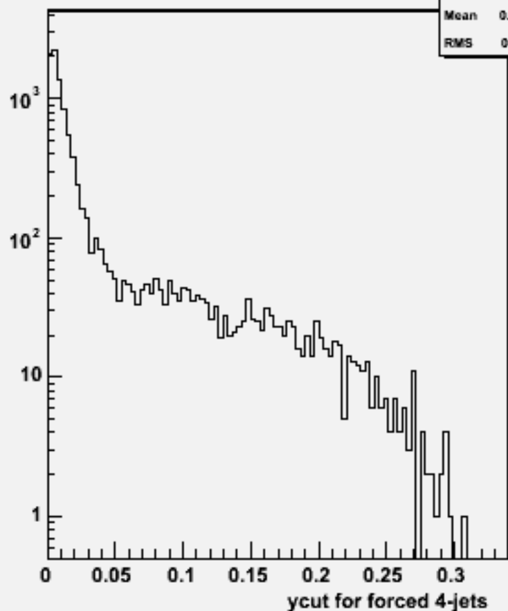
Ycut for 4-jets :w101588 n3n3csdu_o
