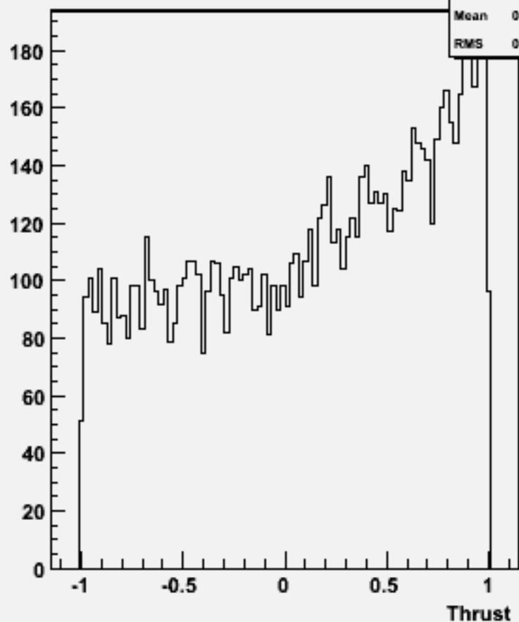
cos \Theta (thrust) w101581 n3n3cse2n2_o
