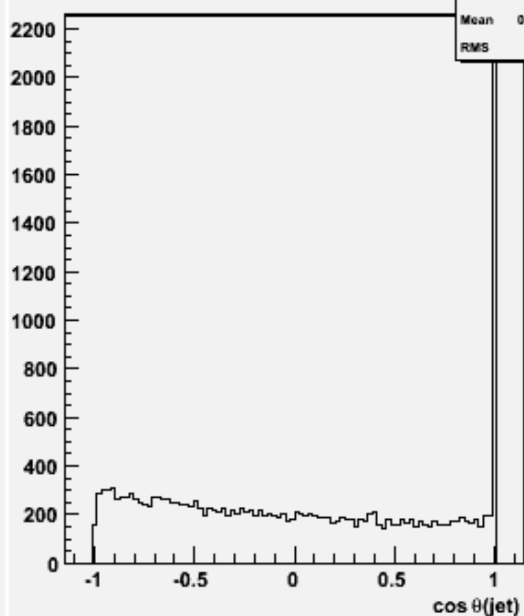
cos \Theta for 2-jets :w101581 n3n3cse2n2_o
