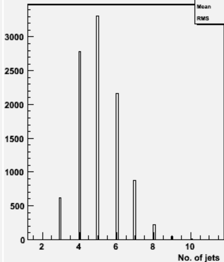
No. jets (ycut=0.001) : w101581 n3n3cse2n2_o
