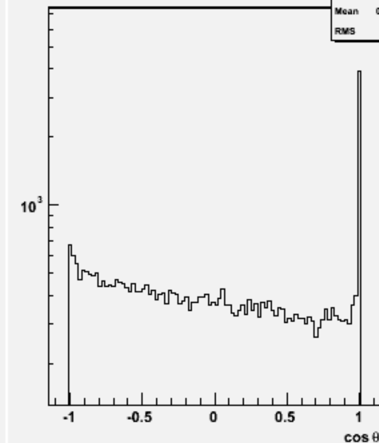
Jet cos \theta (All jets)w101581 n3n3cse2n2_o
