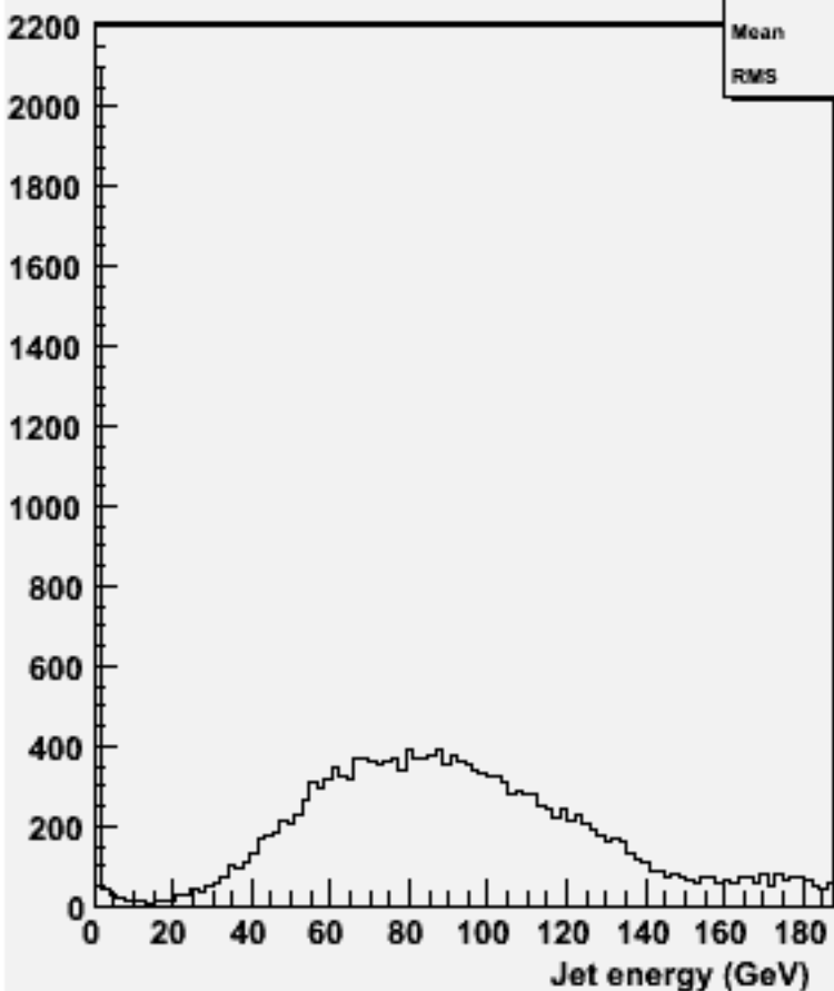
energy for 2-jets :w101581 n3n3cse2n2_o
