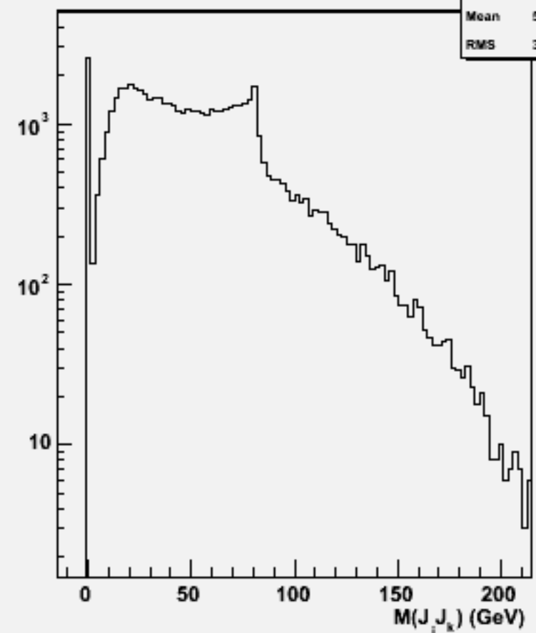
2jets mass(All comb)w101581 n3n3cse2n2_o
