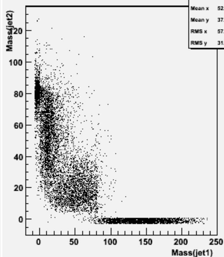
Jet mass for forced 2-jets : w101581 n3n3cse2n2_o
