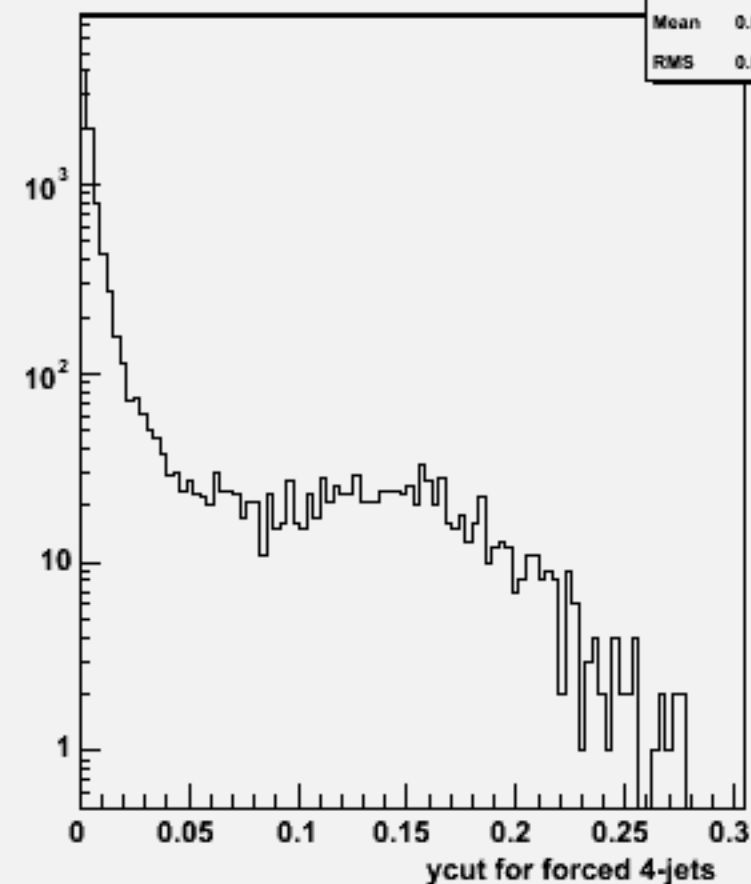
Ycut for 4-jets :w101581 n3n3cse2n2_o
