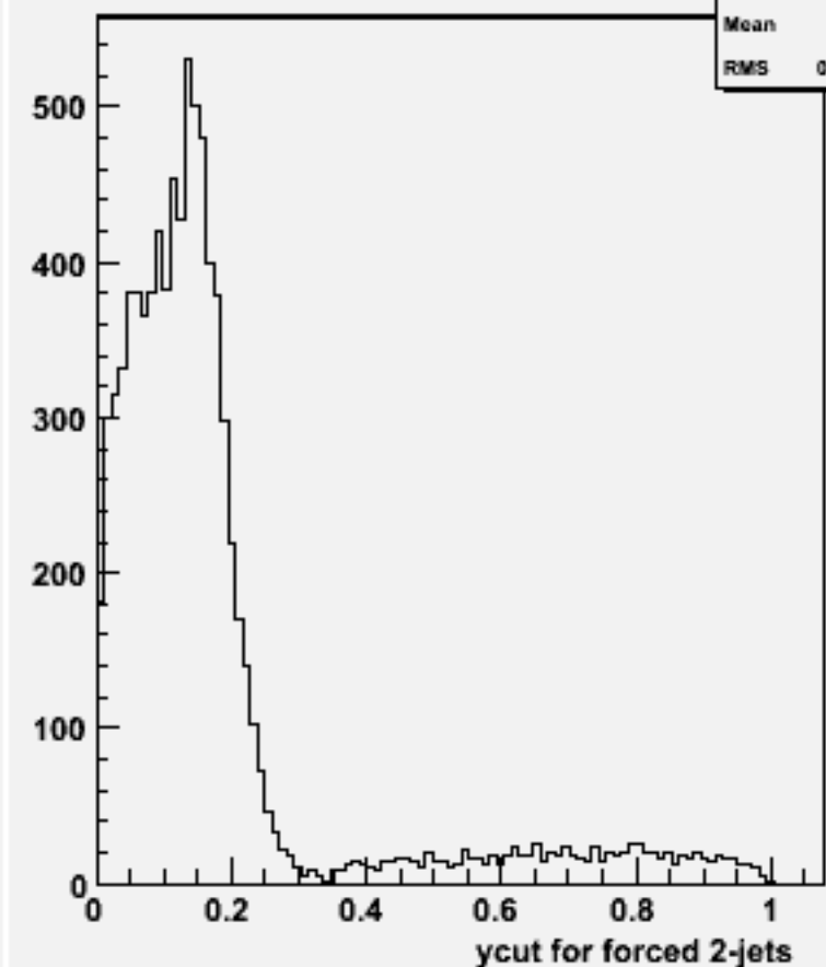
Ycut for 2-jets :w101581 n3n3cse2n2_o
