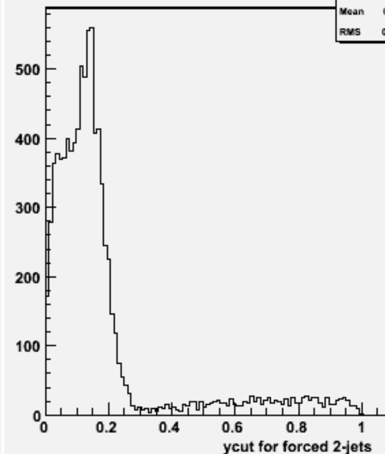
Ycut for 2-jets :w101580 n3n3cse2n2_o
