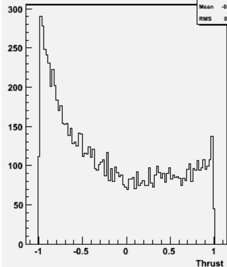
cos \Theta (thrust) w101580 n3n3cse2n2_o
