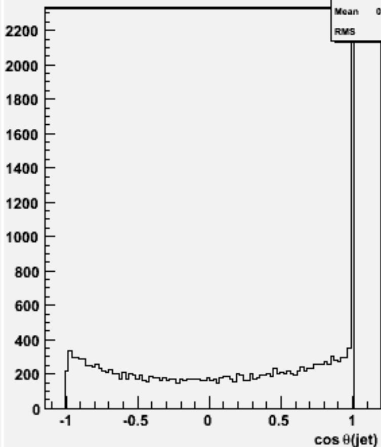
cos \theta for 2-jets :w101580 n3n3cse2n2_o
