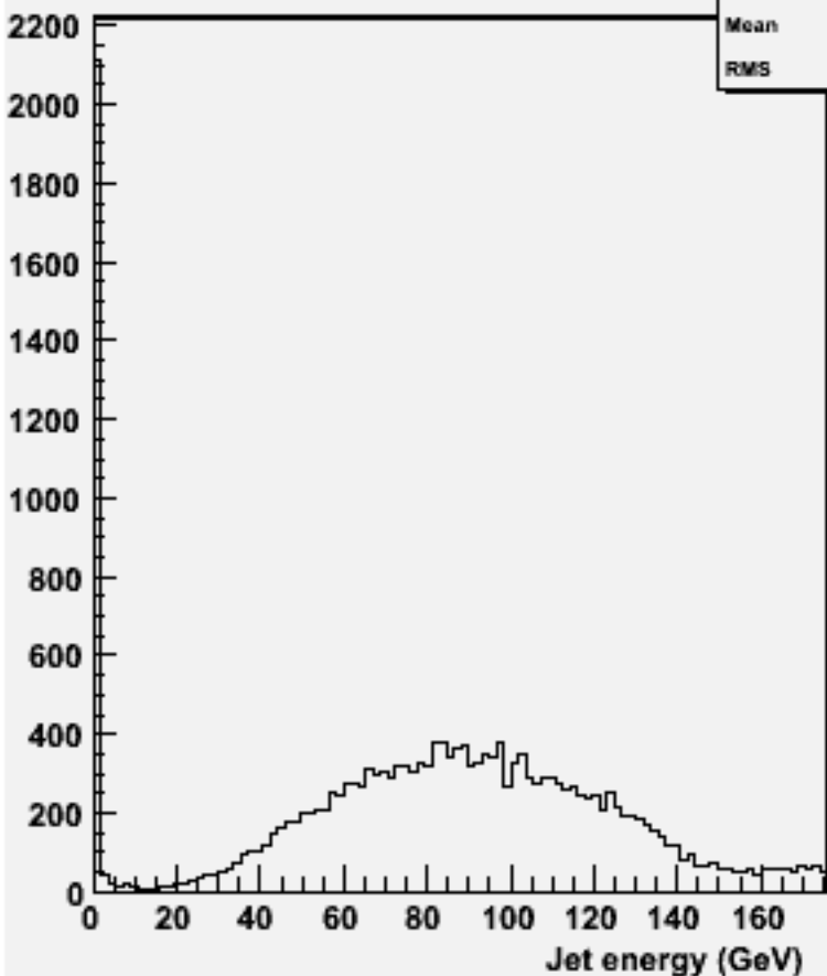
energy for 2-jets :w101580 n3n3cse2n2_o
