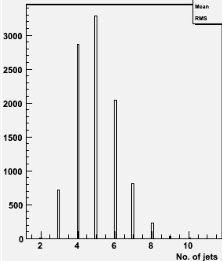
No. jets (ycut=0.001) : w101580 n3n3cse2n2_o
