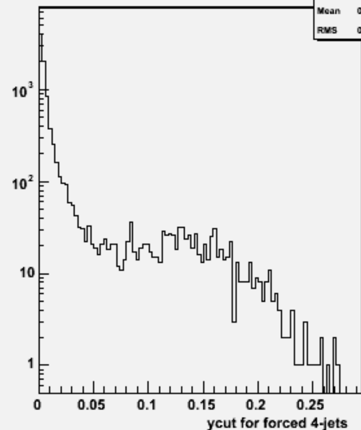
Ycut for 4-jets :w101580 n3n3cse2n2_o
