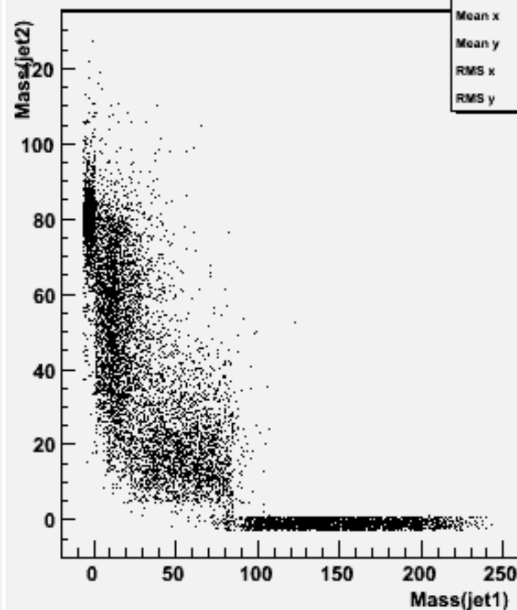
Jet mass for forced 2-jets : w101580 n3n3cse2n2_o
