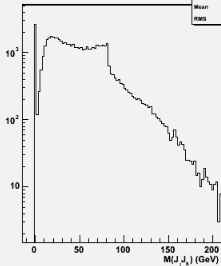
2jets mass(All comb)w101578 n3n3cse1n1_o
