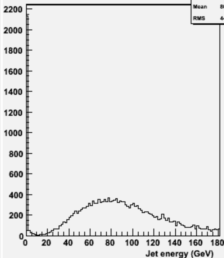
energy for 2-jets :w101578 n3n3cse1n1_o
