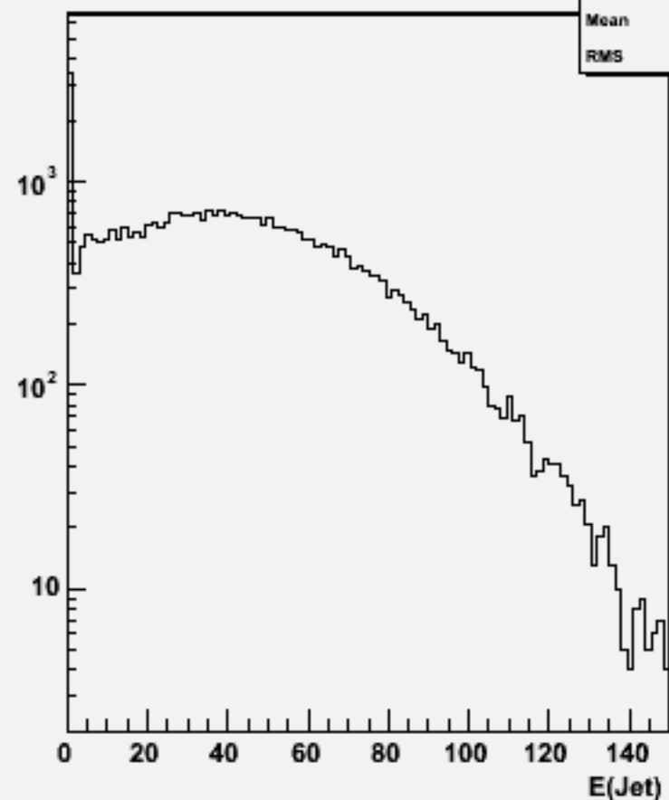
Jet energies(All jets)w101578 n3n3cse1n1_o
