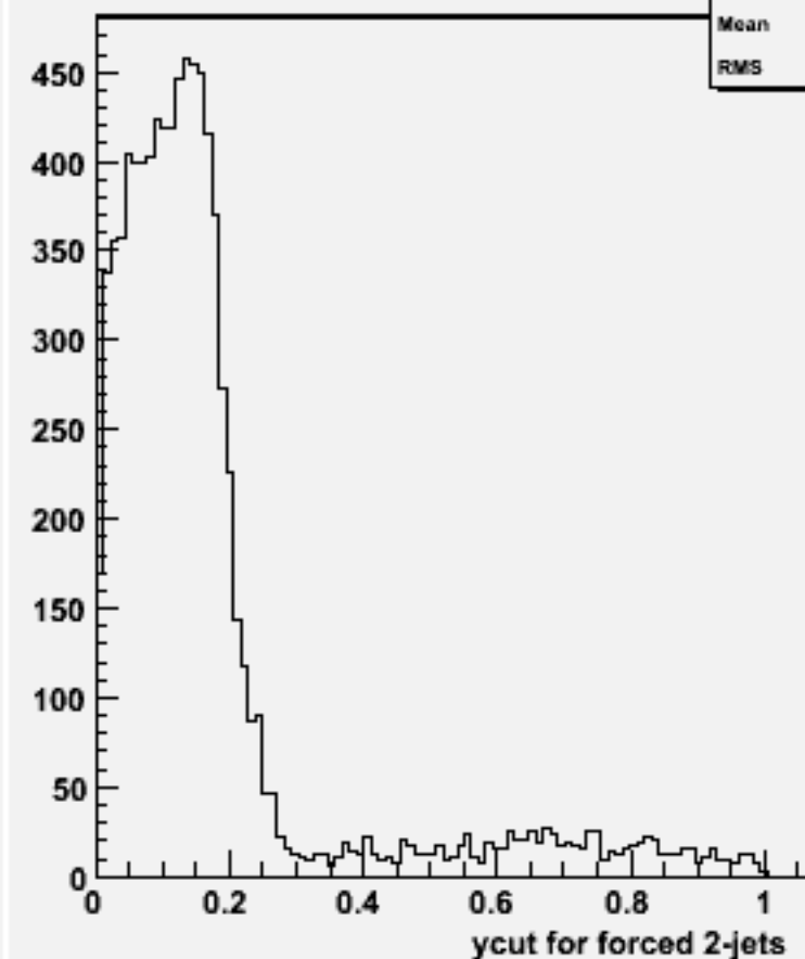
Ycut for 2-jets :w101578 n3n3cse1n1_o
