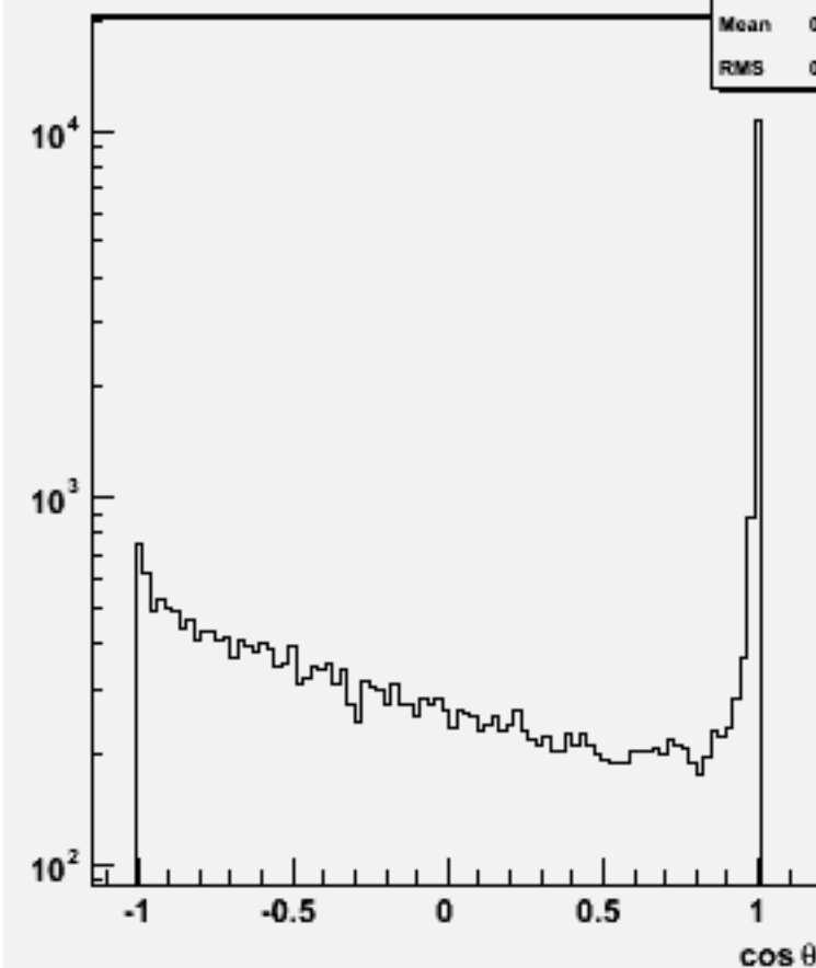
Jet cos \theta (All jets)w101578 n3n3cse1n1_o
