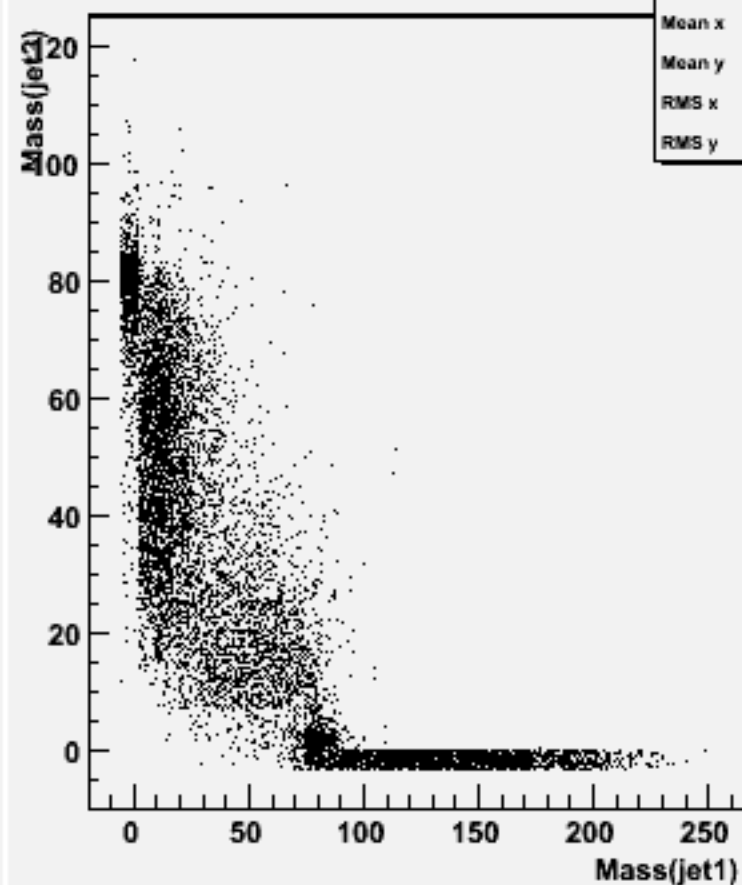
Jet mass for forced 2-jets : w101578 n3n3cse1n1_o
