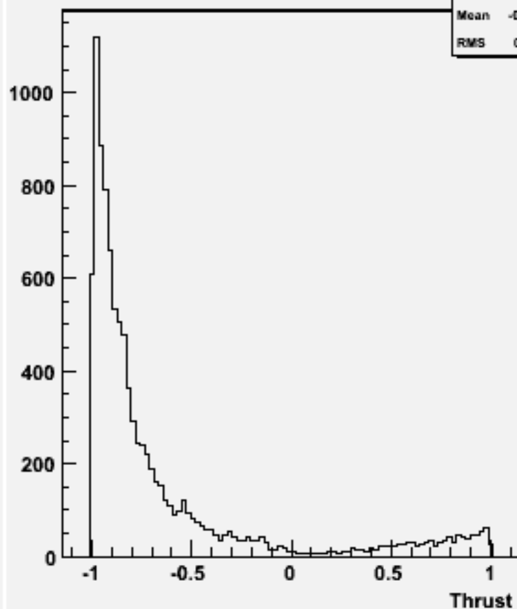
cos \Theta (thrust) w101578 n3n3cse1n1_o
