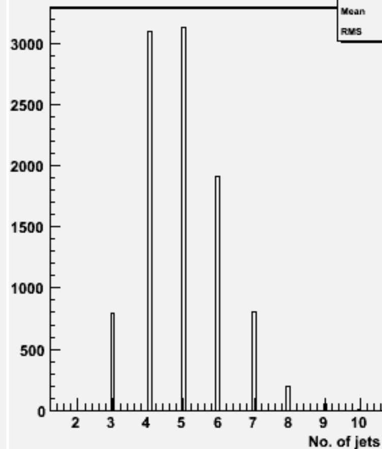
No. jets (ycut=0.001) : w101578 n3n3cse1n1_o
