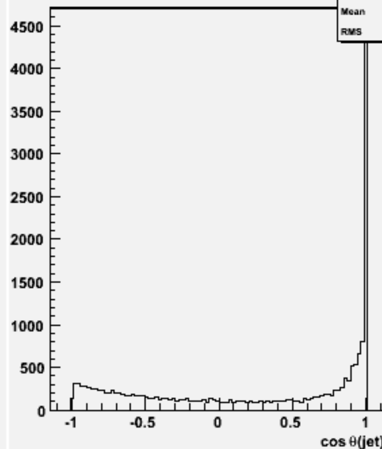
cos \theta for 2-jets :w101578 n3n3cse1n1_o
