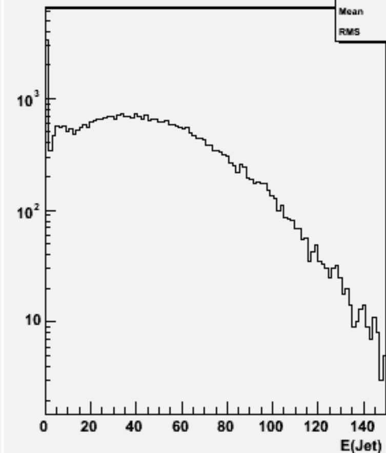
Jet energies(All jets)w101576 n3n3cse1n1_o
