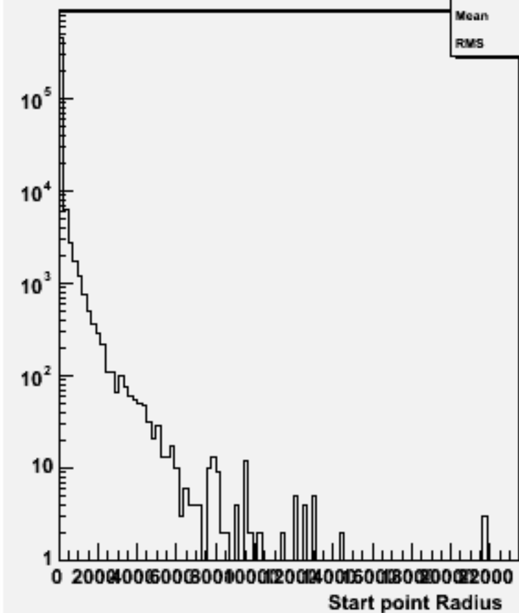
Start point R : w101576 n3n3cse1n1_o
