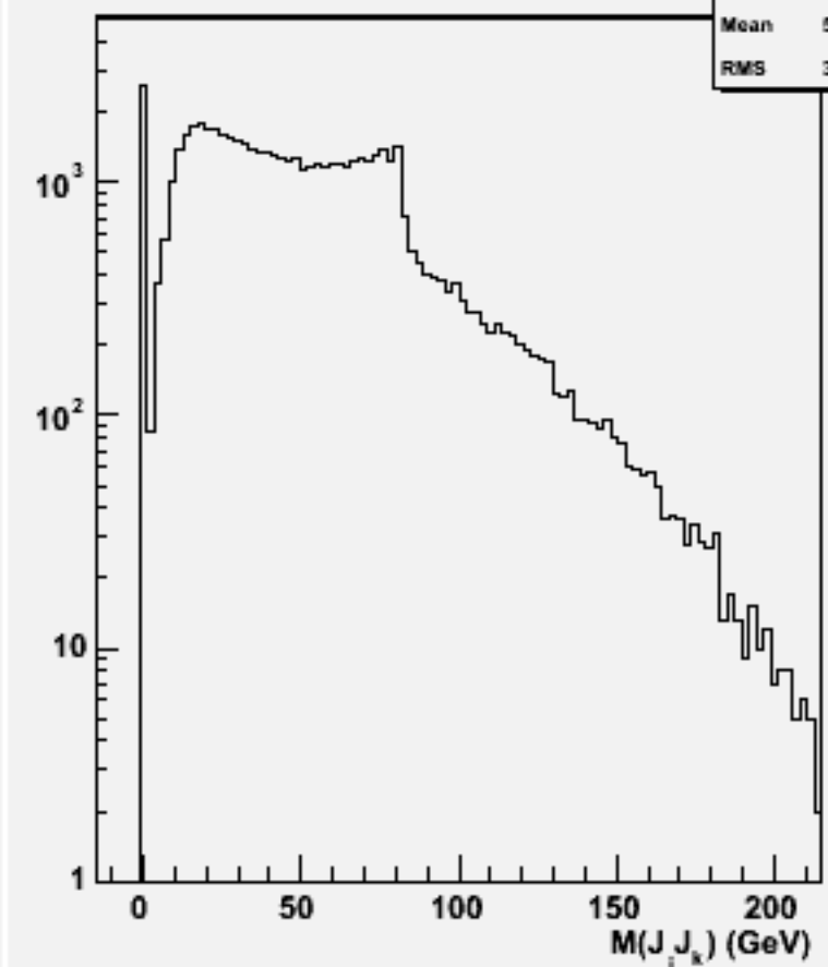
2jets mass(All comb)w101576 n3n3cse1n1_o
