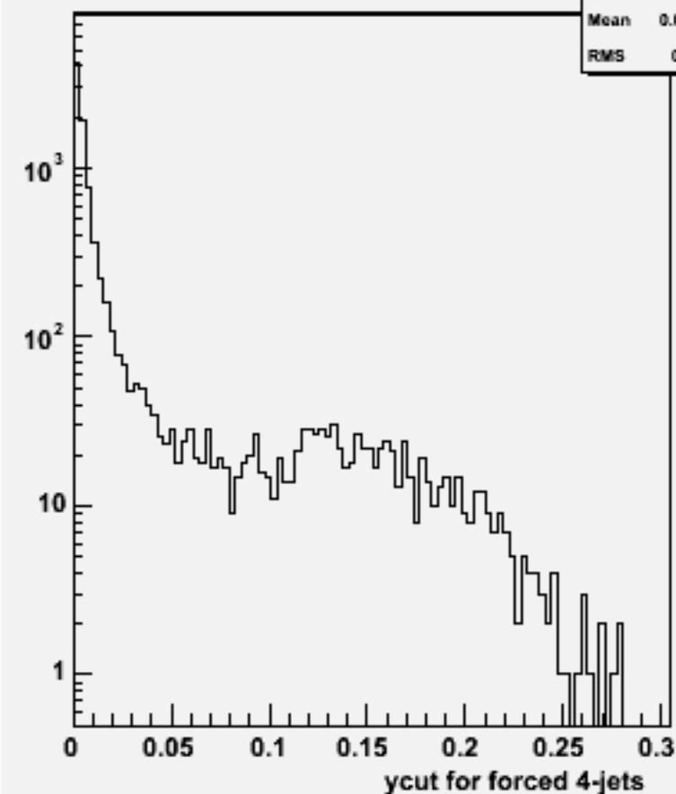
Ycut for 4-jets :w101576 n3n3cse1n1_o
