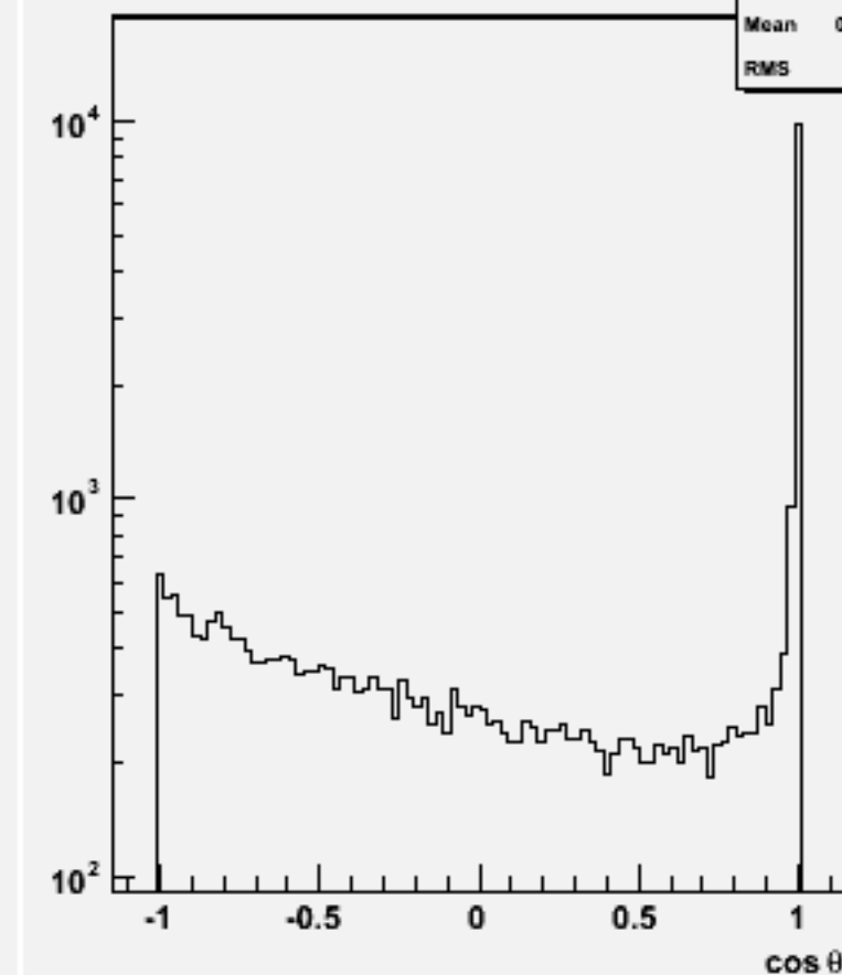
Jet cos \theta (All jets)w101576 n3n3cse1n1_o
