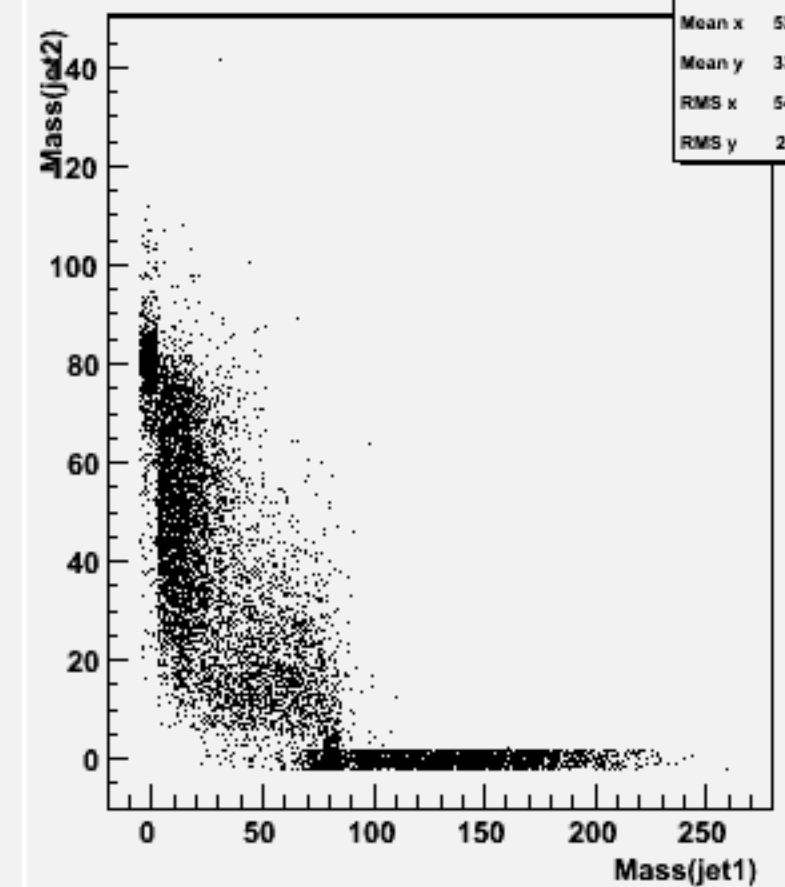
Jet mass for forced 2-jets : w101576 n3n3cse1n1_o
