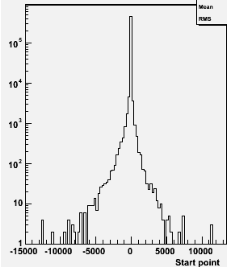
Start point Z : w101576 n3n3cse1n1_o
