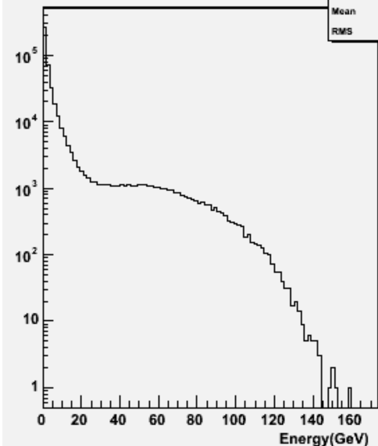
Particle Energy : w101576 n3n3cse1n1_o
