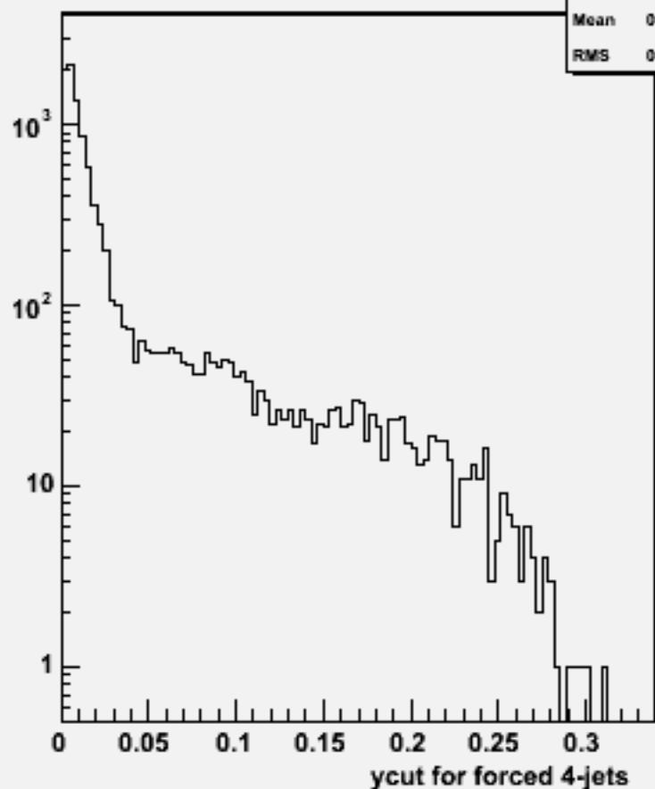
Ycut for 4-jets :w101573 n3n3udsc_o
