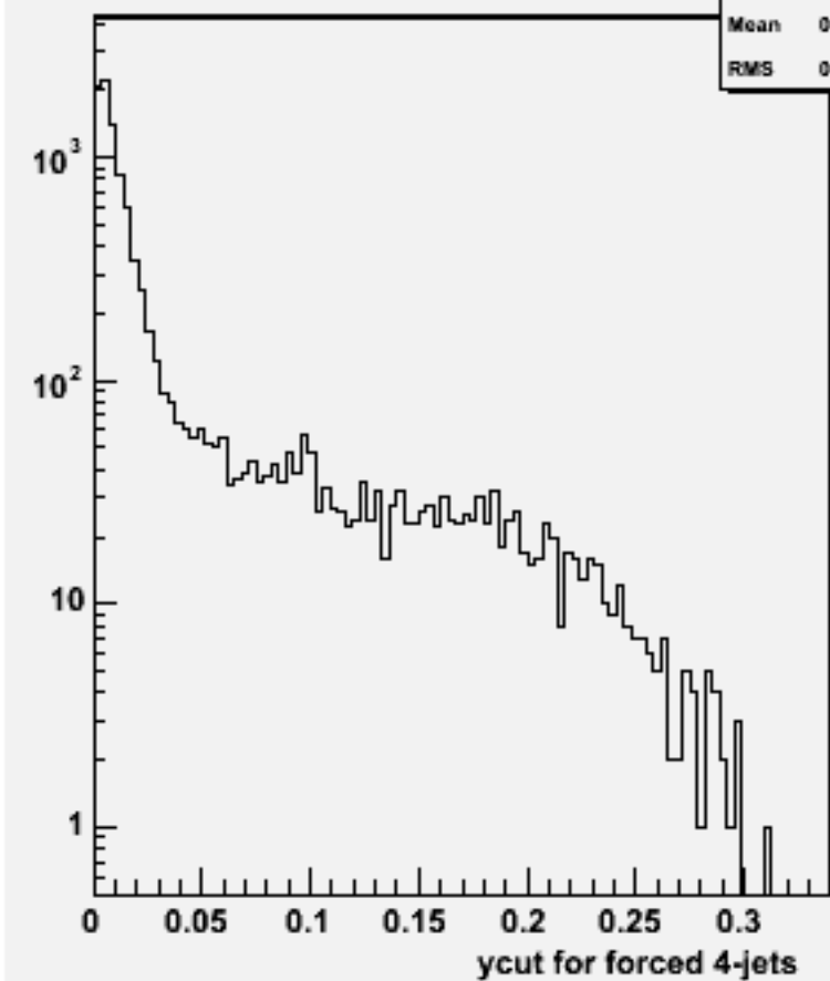
Ycut for 4-jets :w101572 n3n3udsc_o
