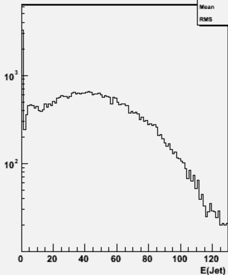
Jet energies(All jets)w101561 n3n3ude2n2_o
