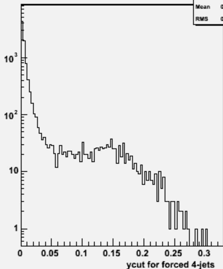
Ycut for 4-jets :w101561 n3n3ude2n2_o
