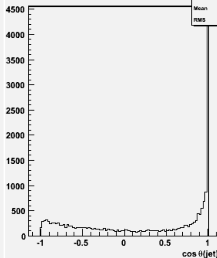
cos \theta for 2-jets :w101558 n3n3ude1n1_o
