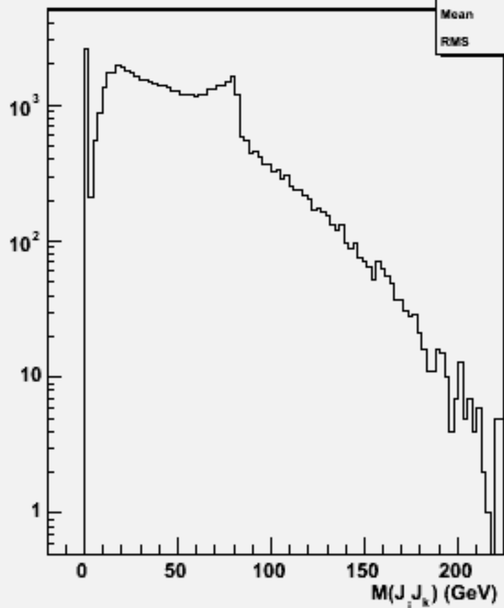
2jets mass(All comb)w101558 n3n3ude1n1_o
