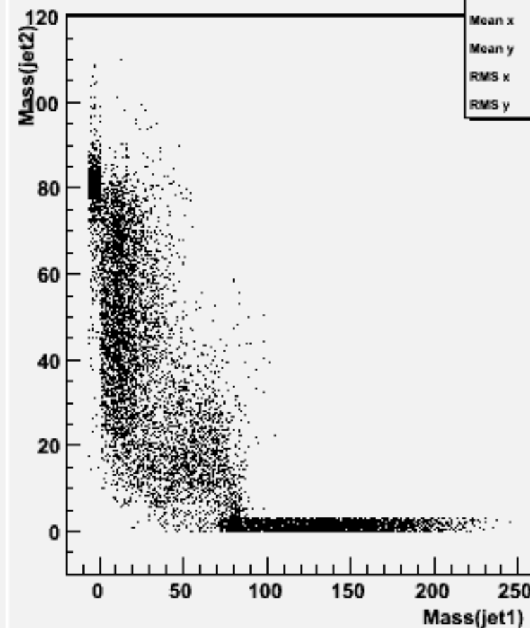
Jet mass for forced 2-jets : w101558 n3n3ude1n1_o
