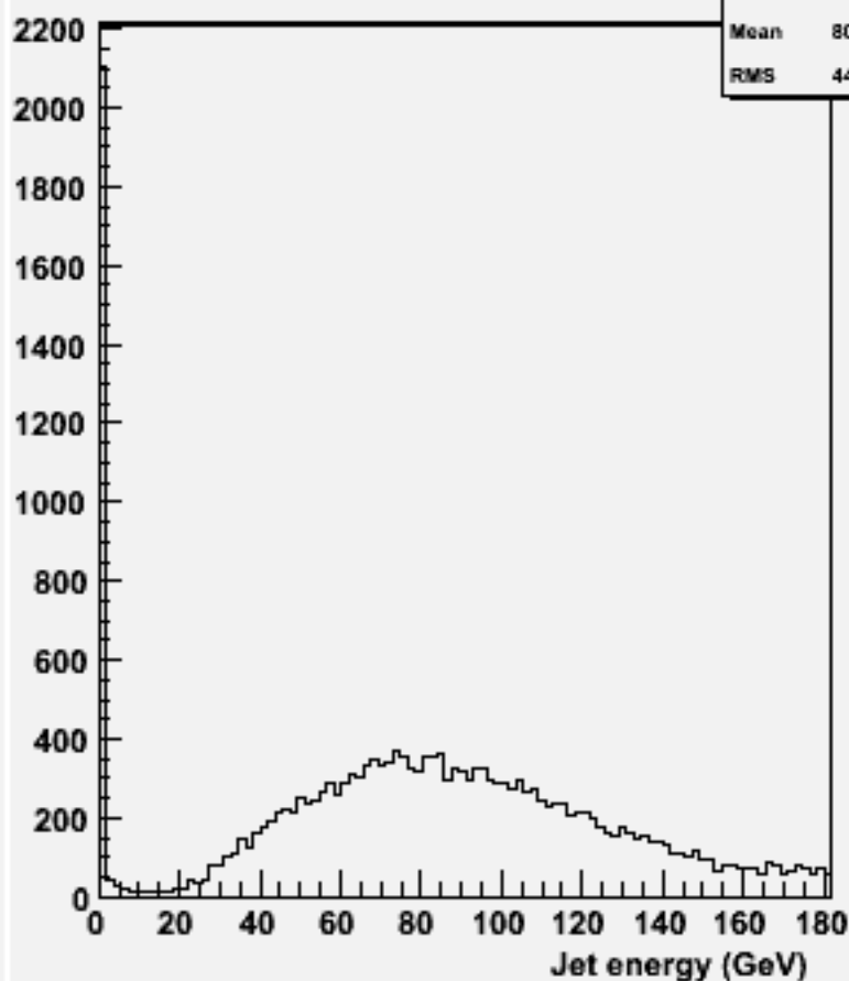
energy for 2-jets :w101558 n3n3ude1n1_o
