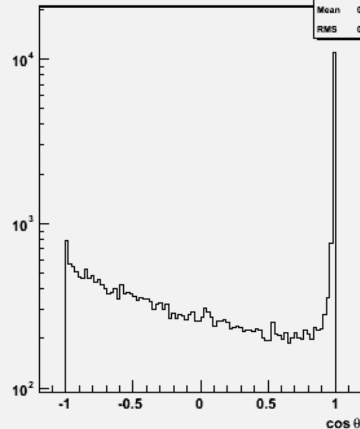
Jet cos \theta (All jets)w101558 n3n3ude1n1_o
