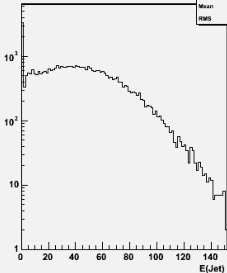
Jet energies(All jets)w101558 n3n3ude1n1_o
