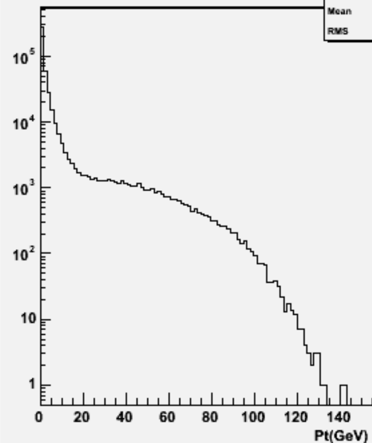
Start point Z : w101557 n3n3ude1n1_o
