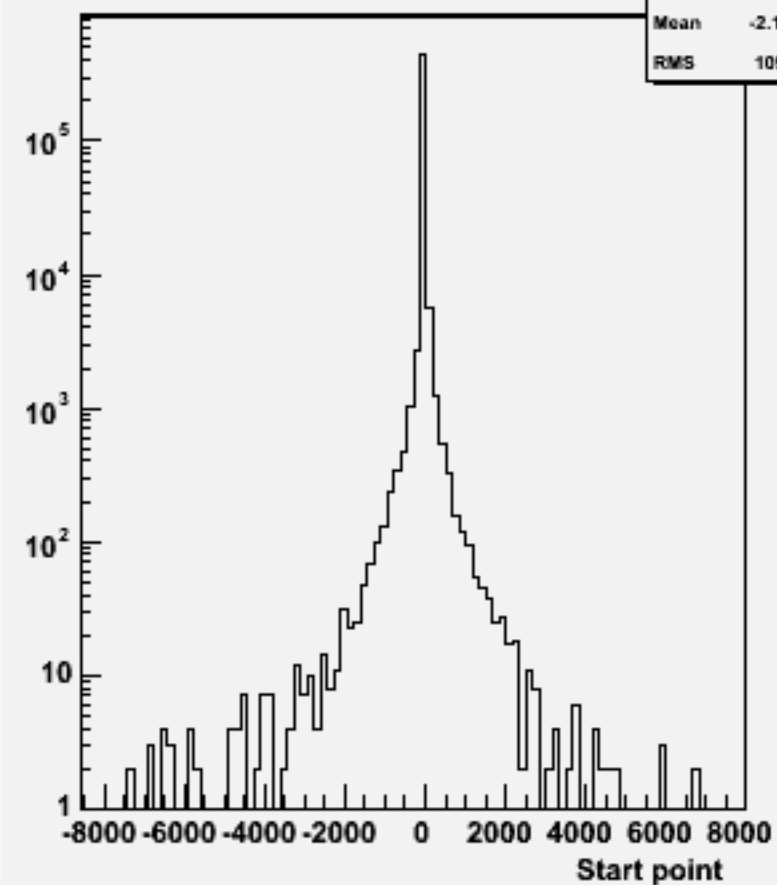
Start point Z : w101557 n3n3ude1n1_o
