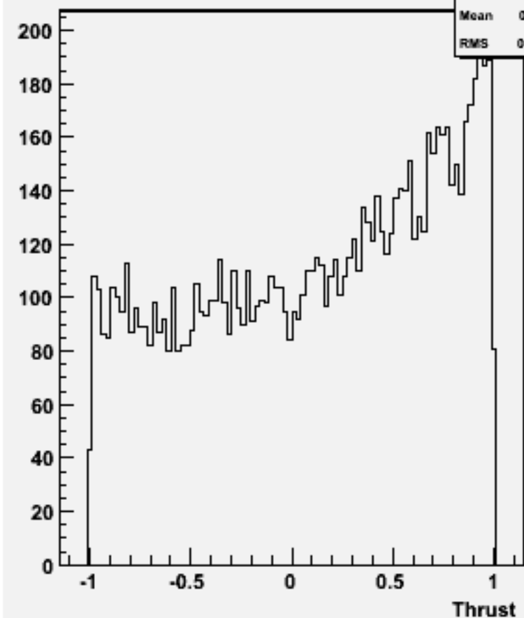
cos \Theta (thrust) w101557 n3n3ude1n1_o
