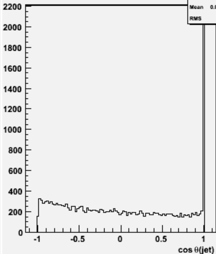
cos \theta for 2-jets :w101557 n3n3ude1n1_o
