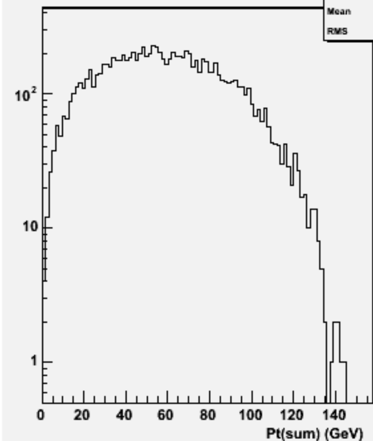
Pt Sum: w101557 n3n3ude1n1_o
