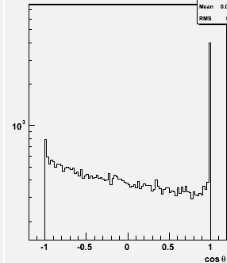
Jet cos \theta (All jets)w101557 n3n3ude1n1_o
