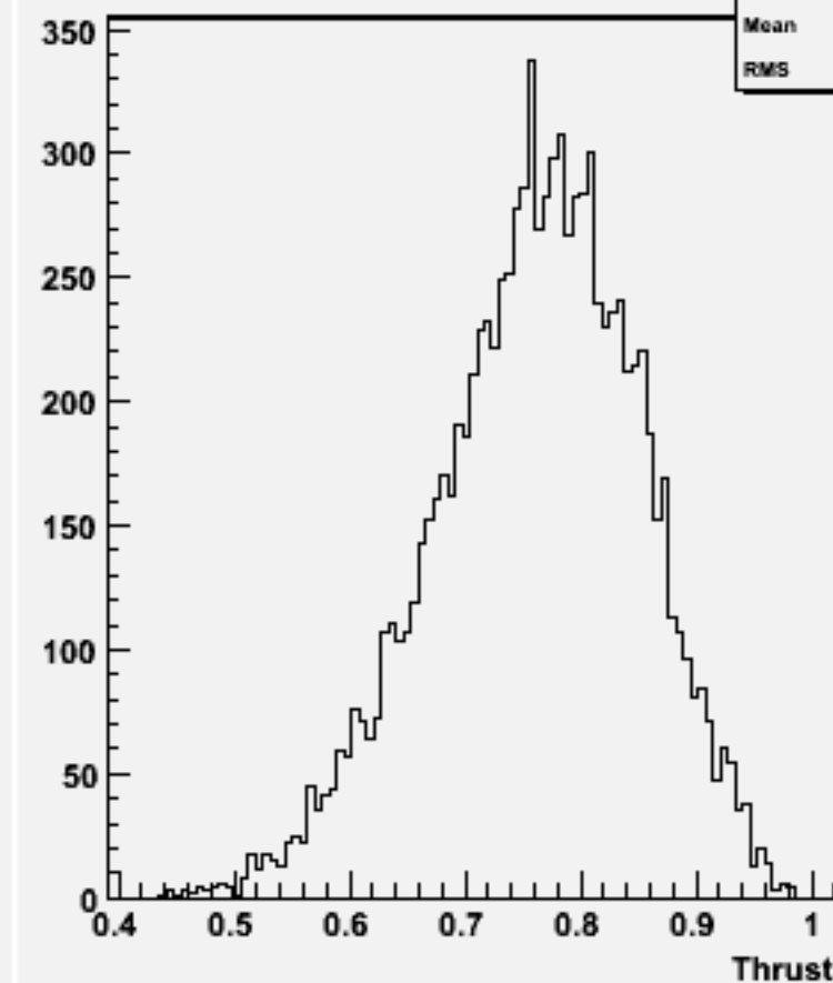
Thrust w101557 n3n3ude1n1_o
