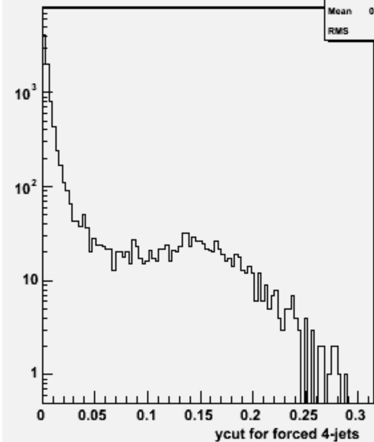
Ycut for 4-jets :w101557 n3n3ude1n1_o
