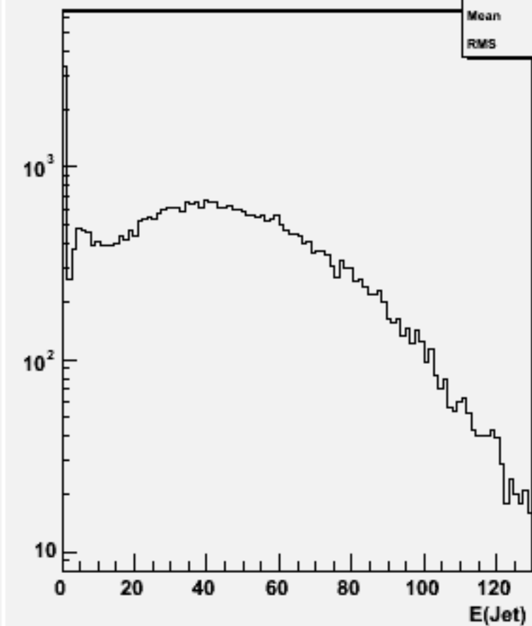
Jet energies(All jets)w101557 n3n3ude1n1_o
