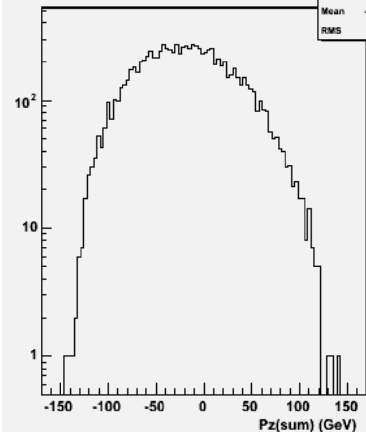
Pz Sum: w101557 n3n3ude1n1_o
