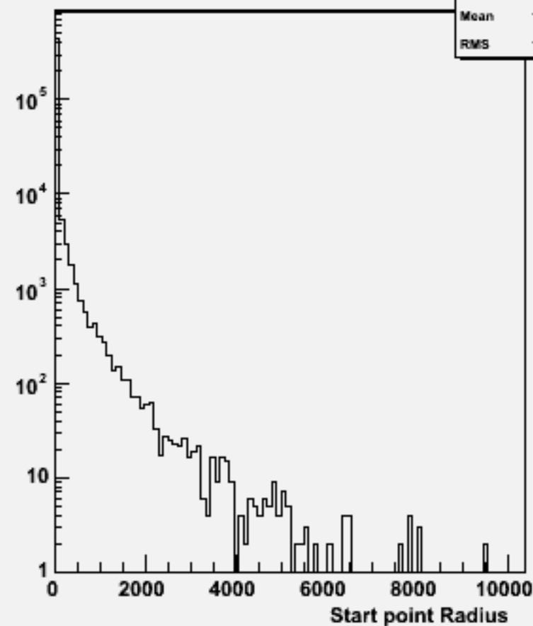
Start point R : w101557 n3n3ude1n1_o
