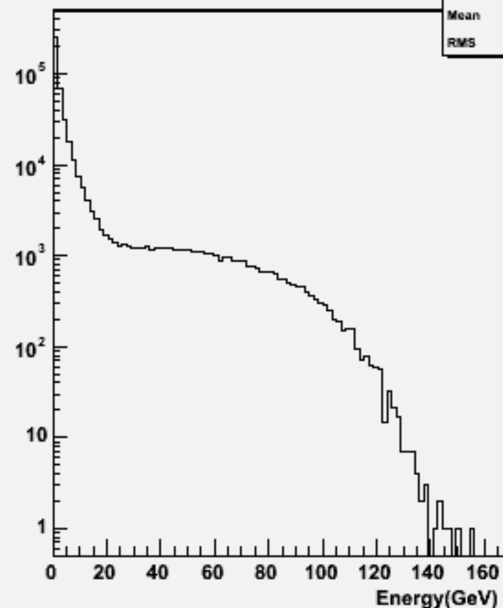
Start point R : w101557 n3n3ude1n1_o
