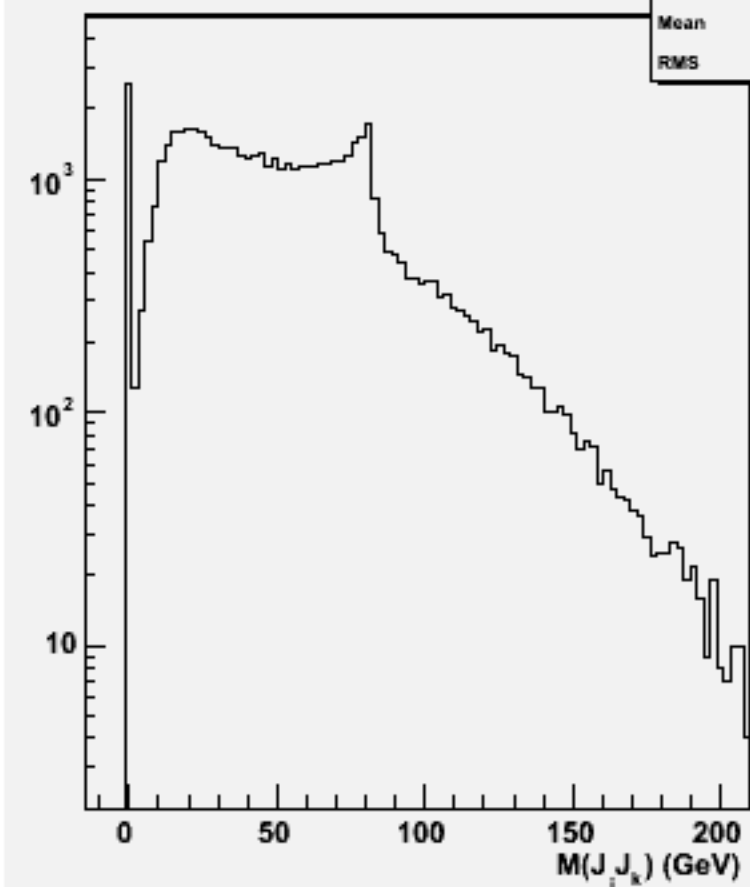
2jets mass(All comb)w101557 n3n3ude1n1_o
