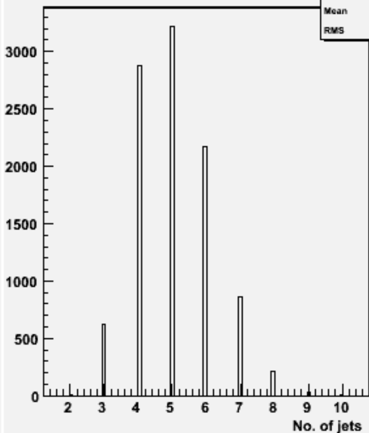
No. jets (ycut=0.001) : w101557 n3n3ude1n1_o
