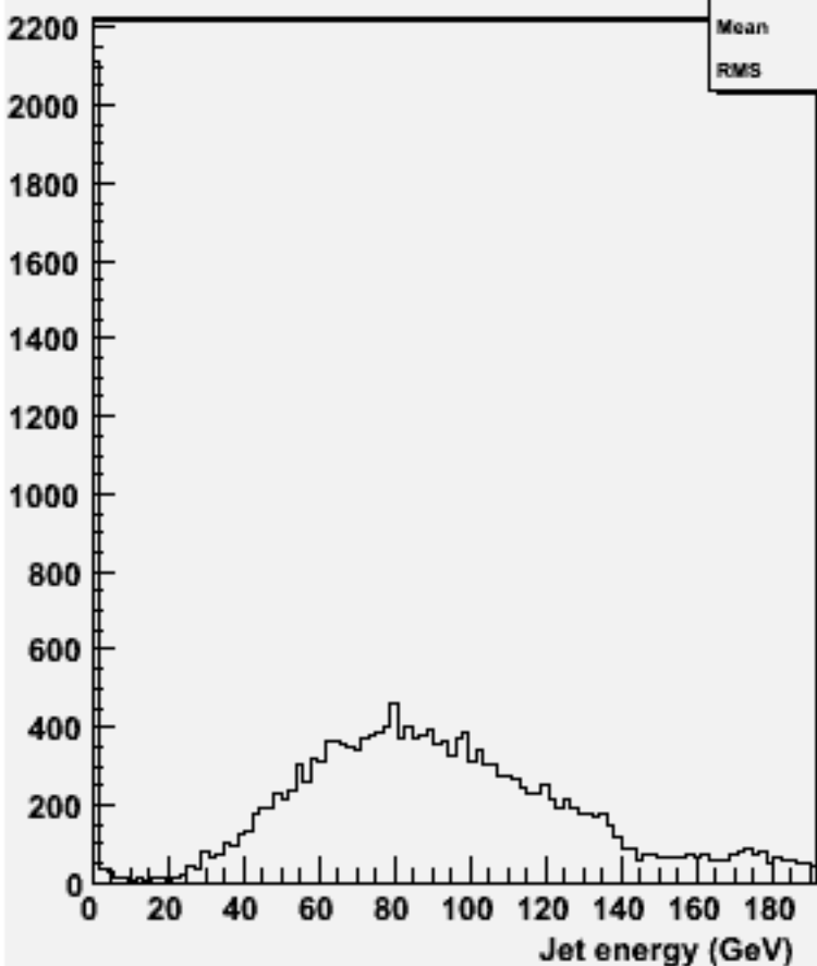
energy for 2-jets :w101557 n3n3ude1n1_o
