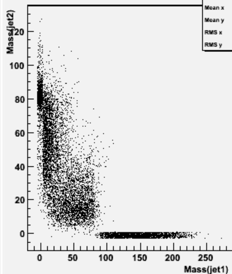
Jet mass for forced 2-jets : w101557 n3n3ude1n1_o
