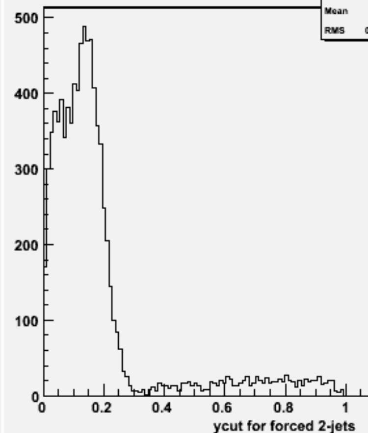
Ycut for 2-jets :w101557 n3n3ude1n1_o
