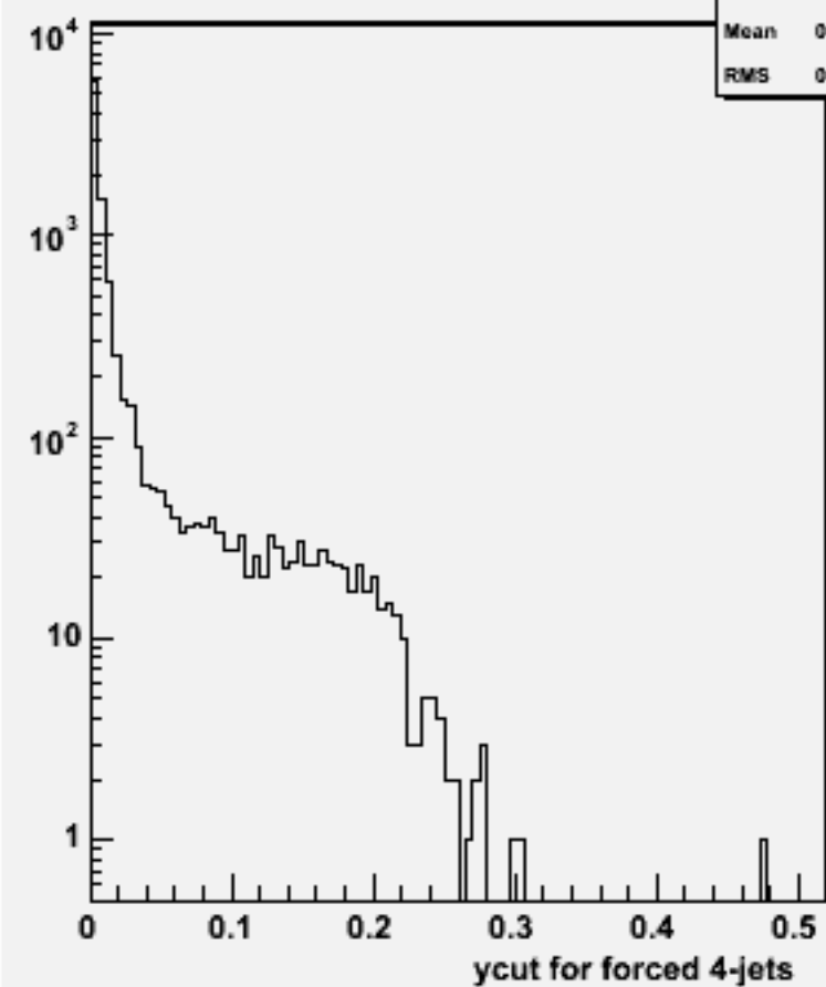
Ycut for 4-jets :w101553 n3n3n3e3sc_o
