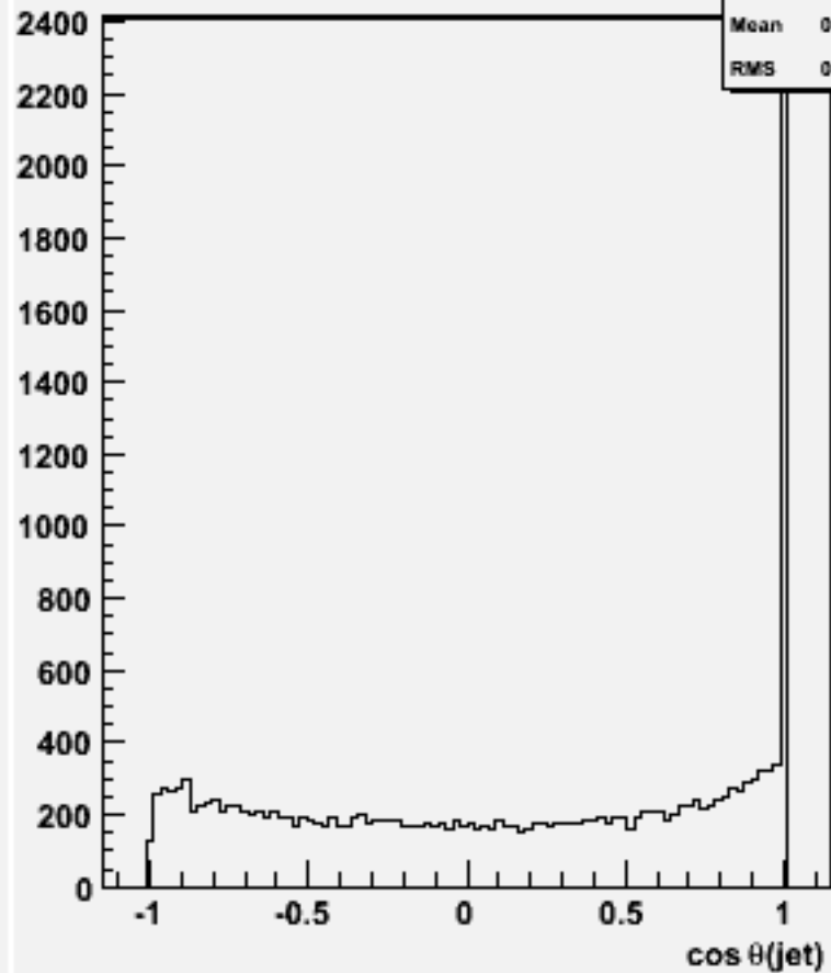
cos \theta for 2-jets :w101552 n3n3n3e3sc_o
