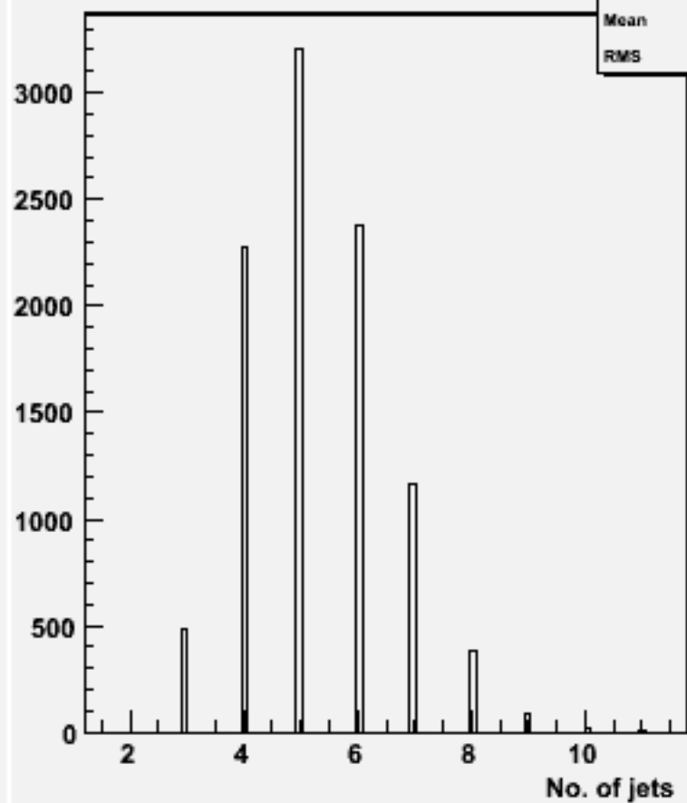
No. jets (ycut=0.001) : w101552 n3n3n3e3sc_o
