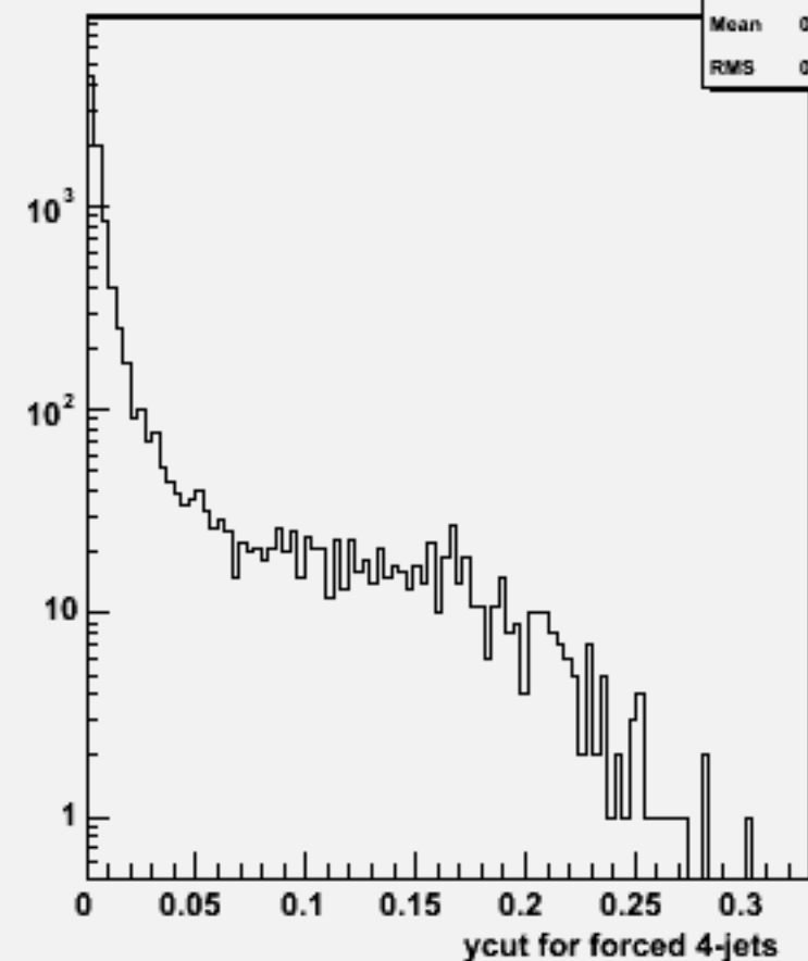
Ycut for 4-jets :w101552 n3n3n3e3sc_o
