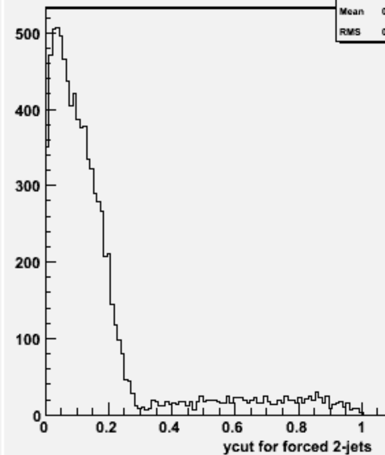
Ycut for 2-jets :w101552 n3n3n3e3sc_o
