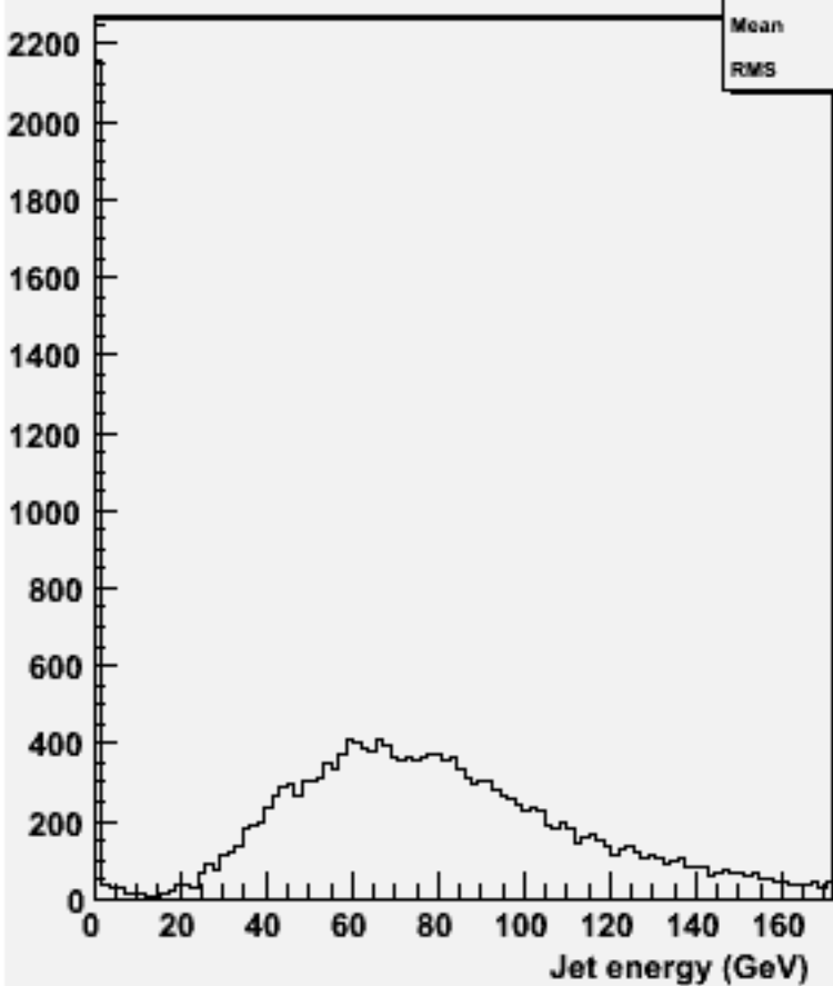
energy for 2-jets :w101552 n3n3n3e3sc_o
