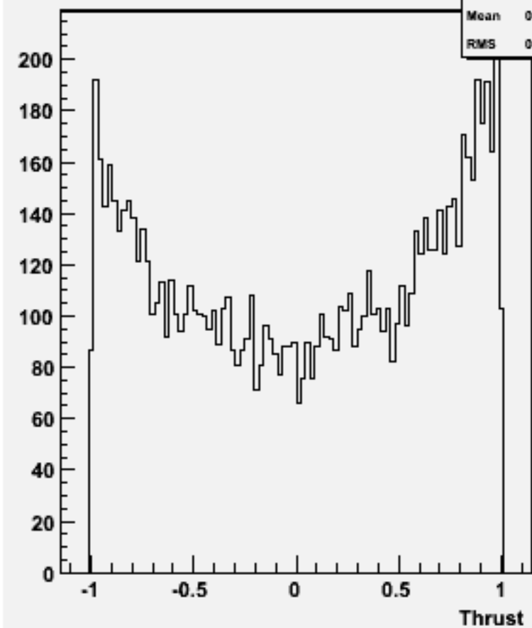
cos \Theta (thrust) w101552 n3n3n3e3sc_o
