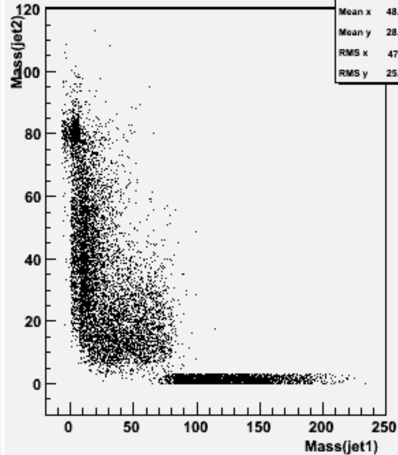
Jet mass for forced 2-jets : w101552 n3n3n3e3sc_o
