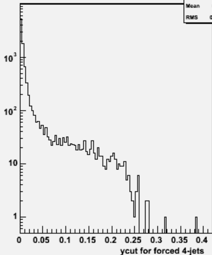
Ycut for 4-jets :w101549 n3n3n3e3du_o
