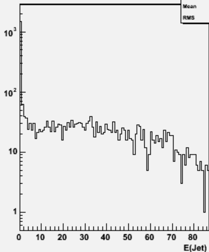
Jet energies(All jets)w101538 n3n3n3e3e1n1_o
