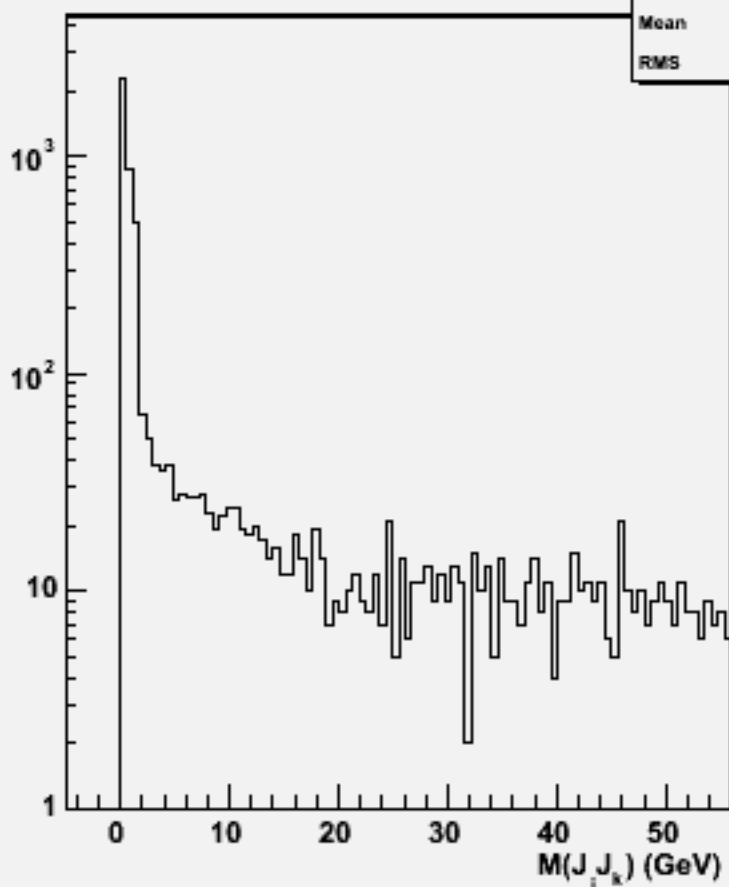
2jets mass(All comb)w101538 n3n3n3e3e1n1_o
