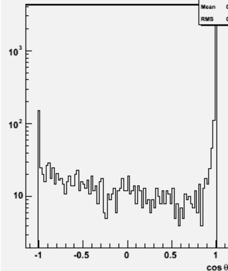
Jet cos \theta (All jets)w101538 n3n3n3e3e1n1_o
