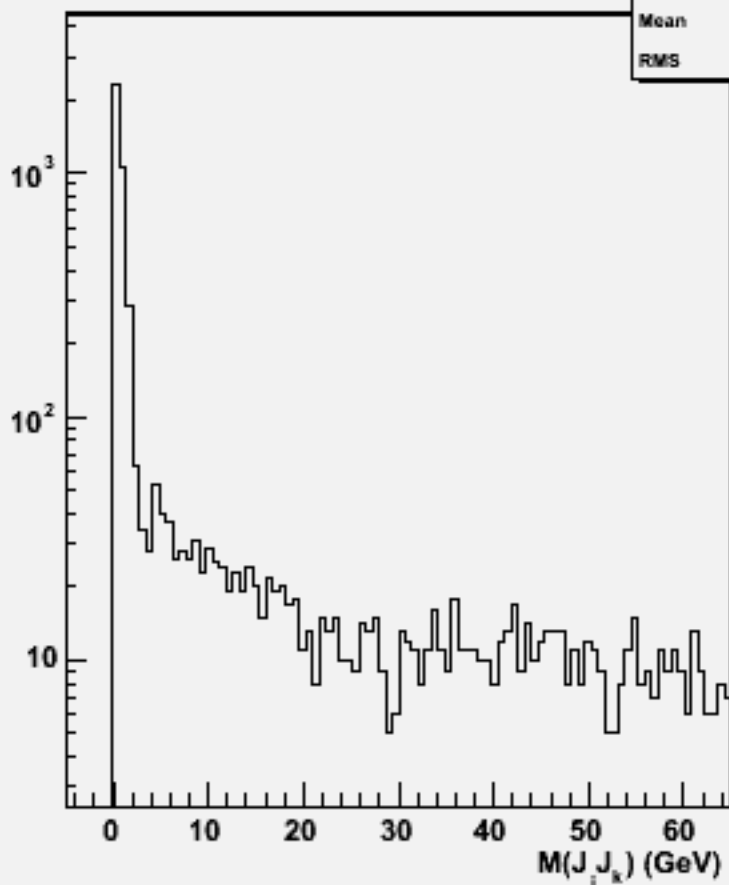
2jets mass(All comb)w101536 n3n3n3e3e1n1_o
