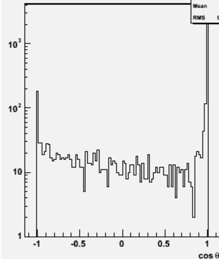
Jet cos \theta (All jets)w101536 n3n3n3e3e1n1_o
