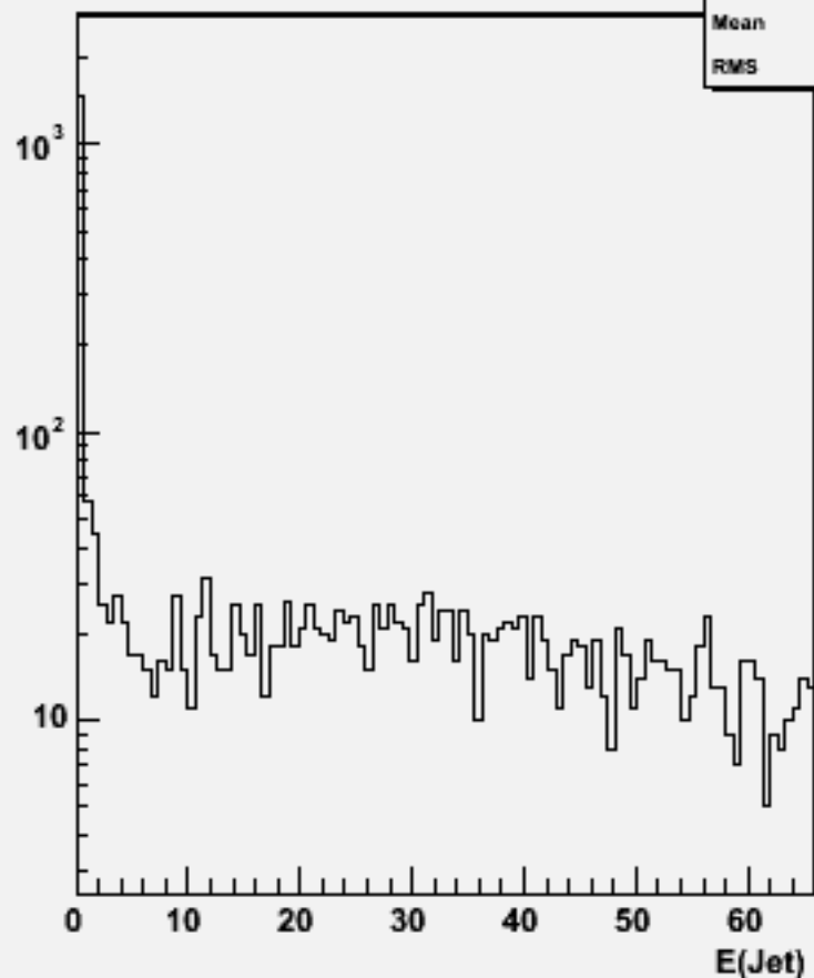
Jet energies(All jets)w101536 n3n3n3e3e1n1_o
