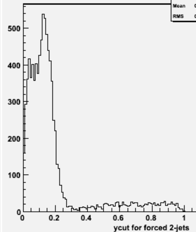
Ycut for 2-jets :w101532 n3n3n2e2sc_o
