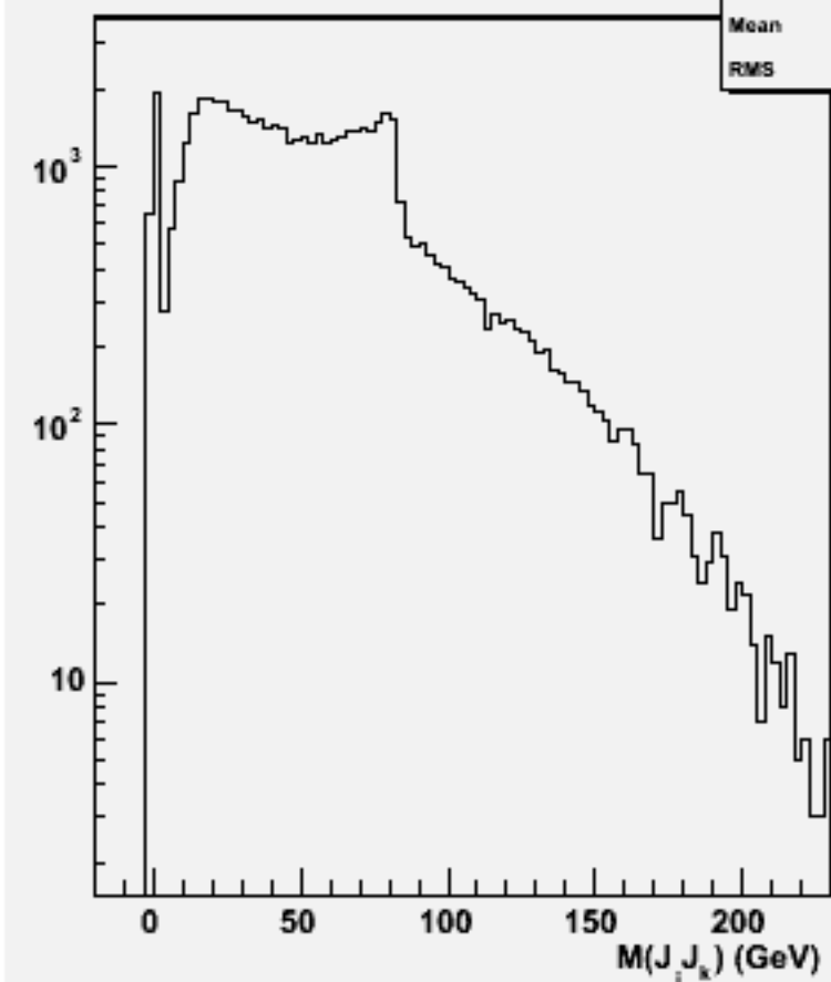
2jets mass(All comb)w101532 n3n3n2e2sc_o
