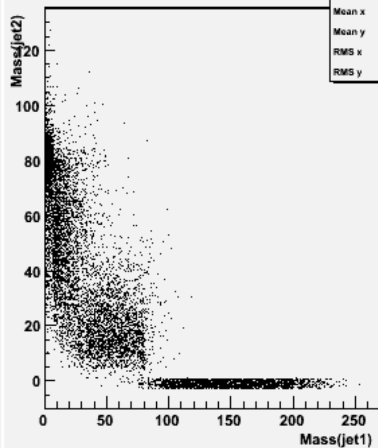
Jet mass for forced 2-jets : w101532 n3n3n2e2sc_o
