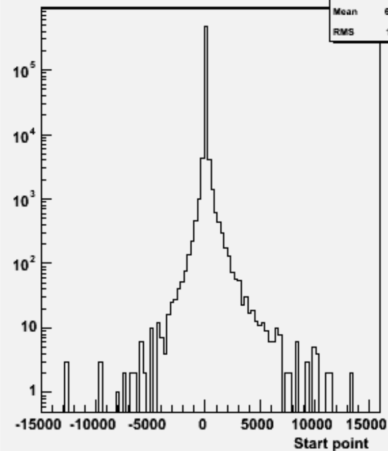
Start point Z : w101532 n3n3n2e2sc_o
