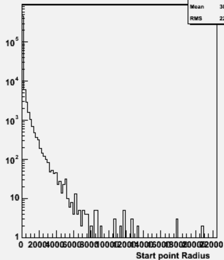
Start point R : w101532 n3n3n2e2sc_o
