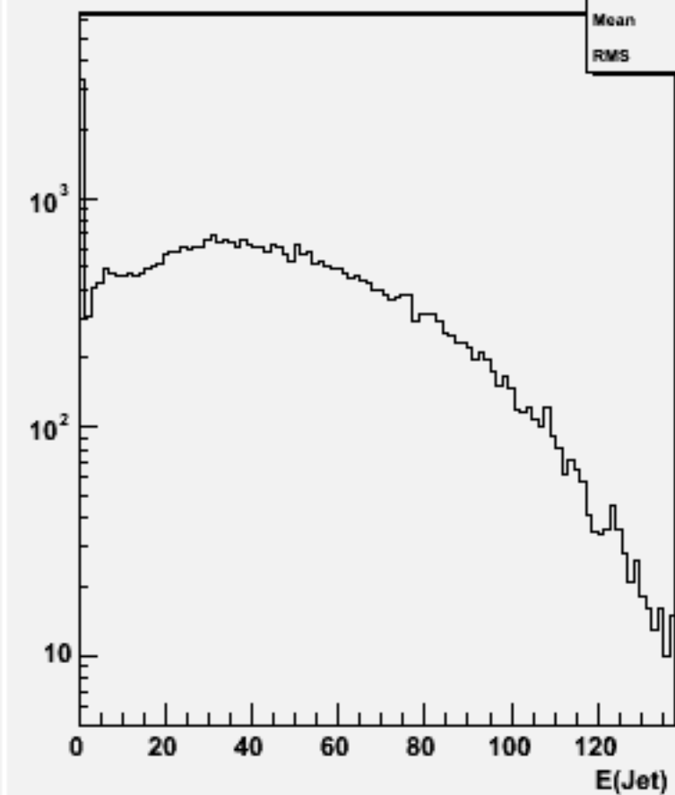
Jet energies(All jets)w101532 n3n3n2e2sc_o
