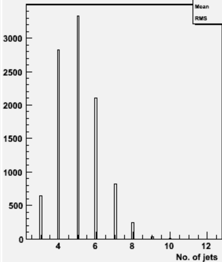
No. jets (ycut=0.001) : w101532 n3n3n2e2sc_o
