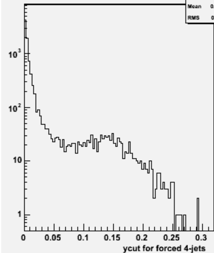
Ycut for 4-jets :w101532 n3n3n2e2sc_o
