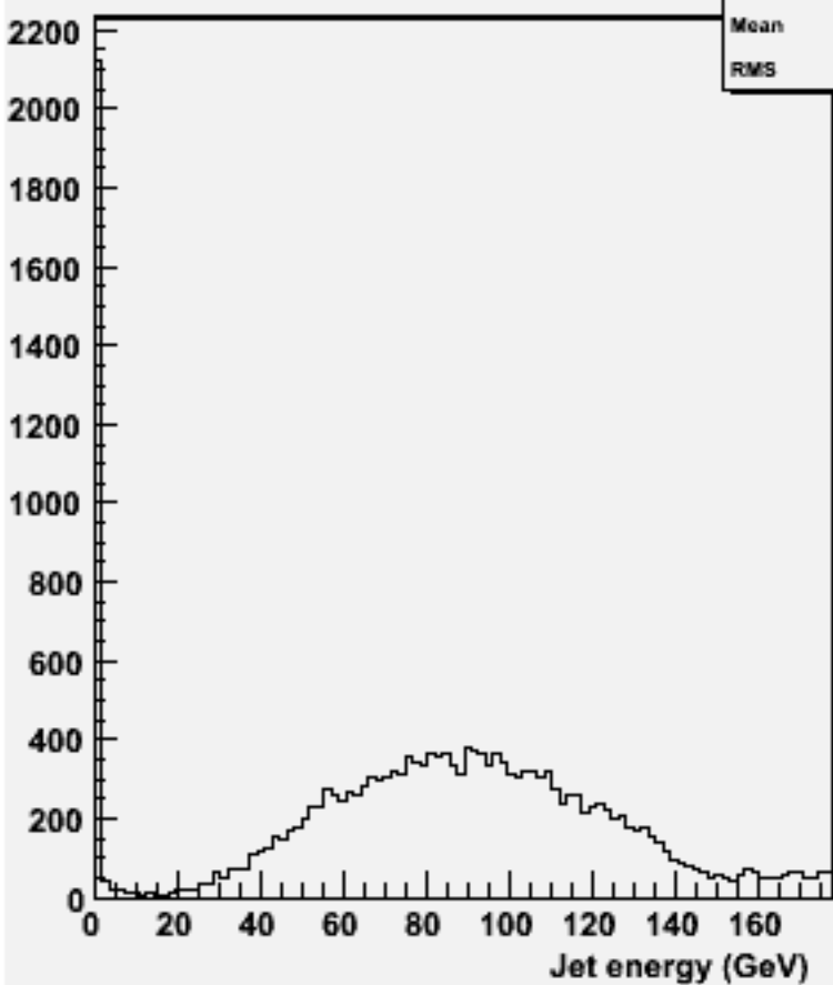
energy for 2-jets :w101532 n3n3n2e2sc_o
