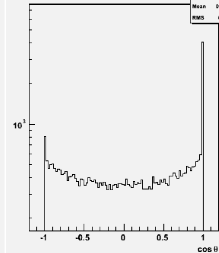
Jet cos \theta (All jets)w101532 n3n3n2e2sc_o
