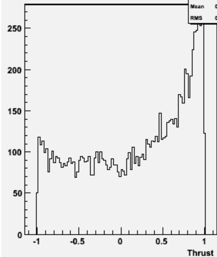
cos \Theta (thrust) w101532 n3n3n2e2sc_o
