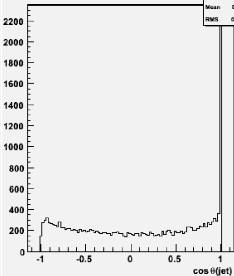
cos \theta for 2-jets :w101532 n3n3n2e2sc_o
