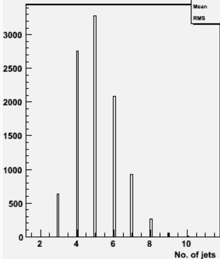
No. jets (ycut=0.001) : w101529 n3n3n2e2du_o
