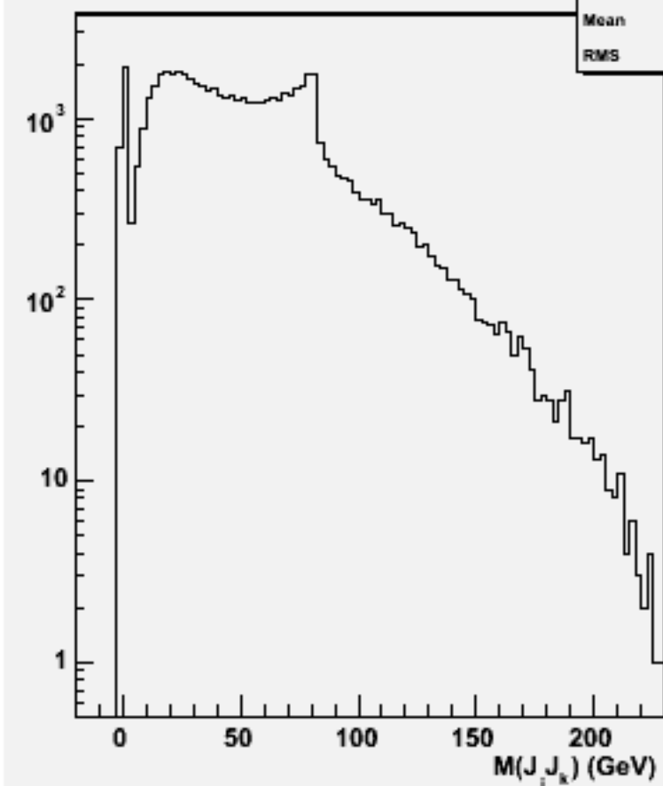
2jets mass(All comb)w101529 n3n3n2e2du_o
