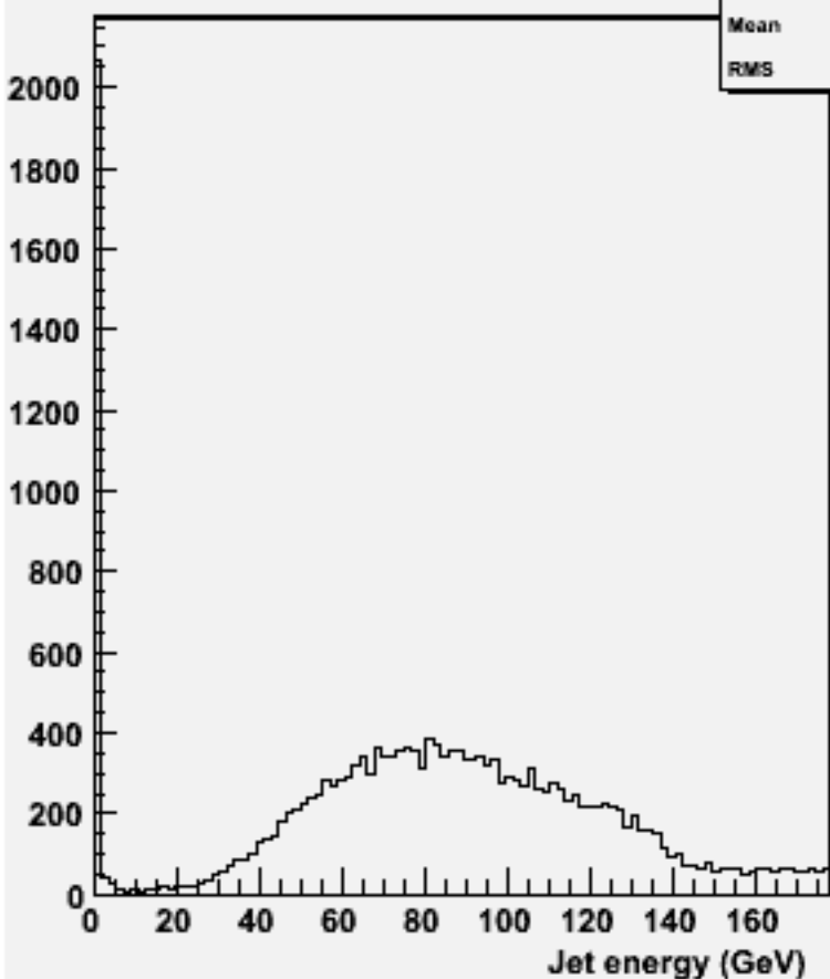
energy for 2-jets :w101529 n3n3n2e2du_o
