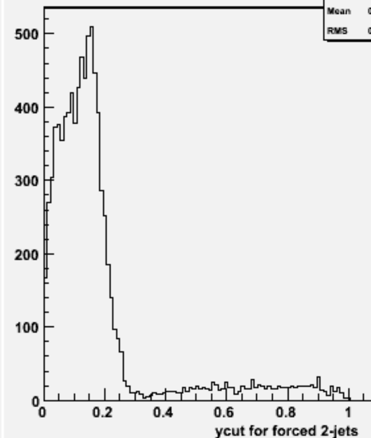
Ycut for 2-jets :w101529 n3n3n2e2du_o
