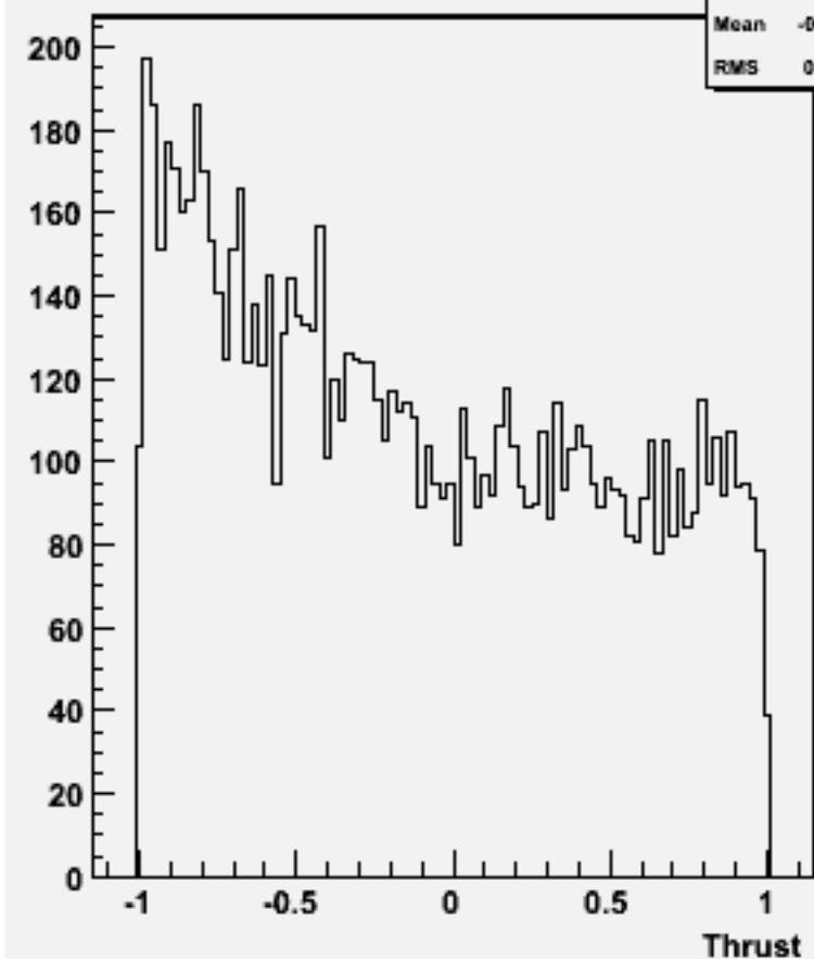
cos \Theta (thrust) w101529 n3n3n2e2du_o
