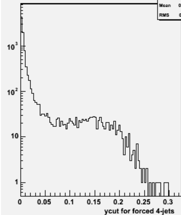
Ycut for 4-jets :w101529 n3n3n2e2du_o
