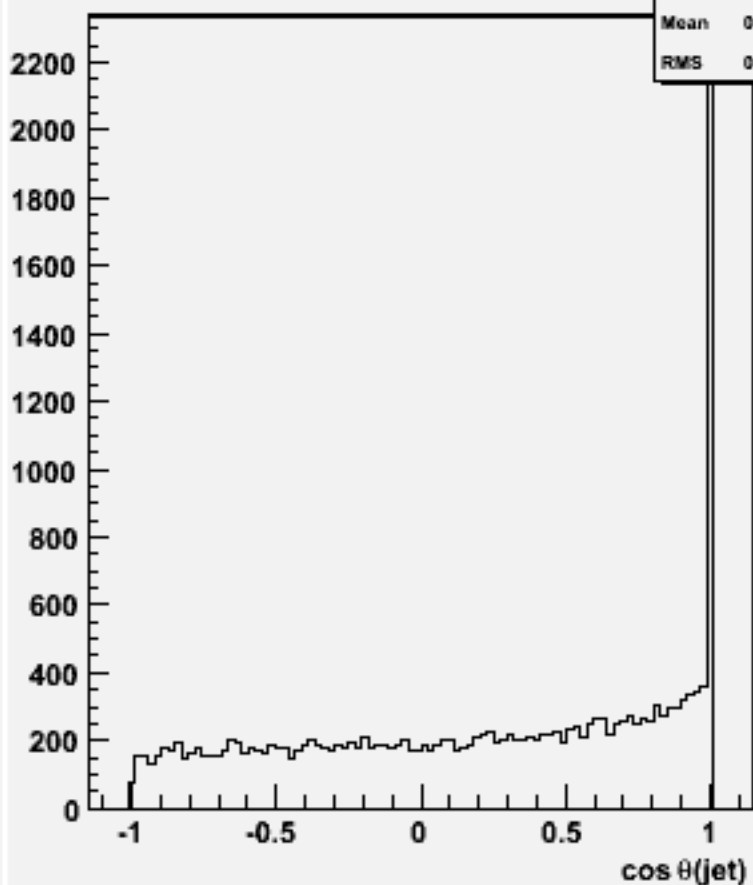
cos \theta for 2-jets :w101529 n3n3n2e2du_o
