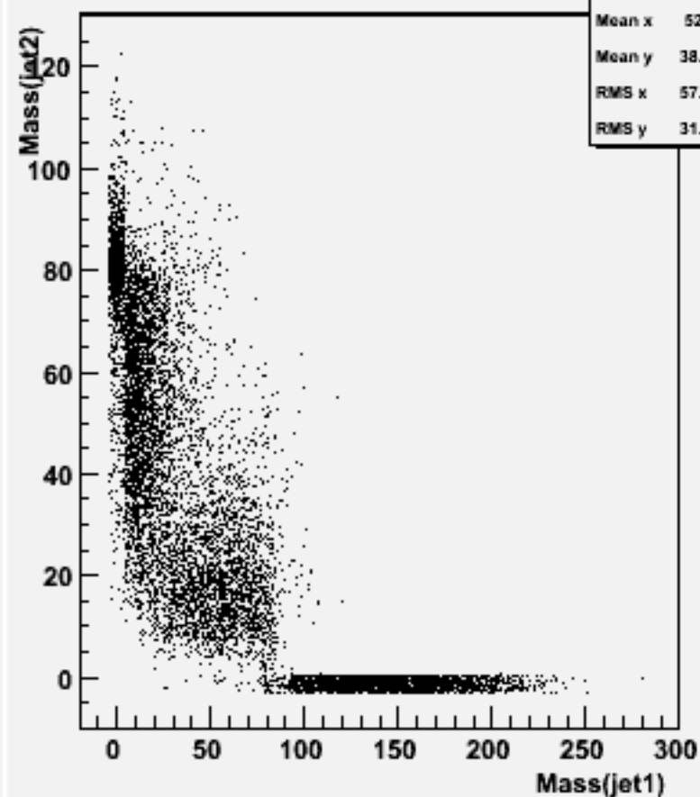
Jet mass for forced 2-jets : w101529 n3n3n2e2du_o
