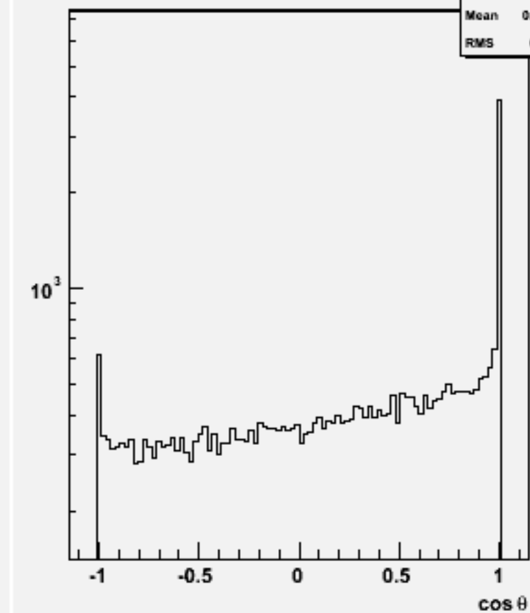
Jet cos \theta (All jets)w101529 n3n3n2e2du_o
