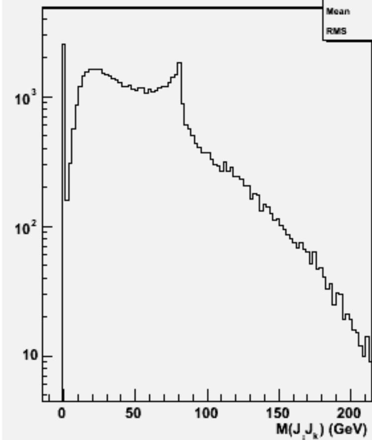
2jets mass(All comb)w101528 n3n3n2e2du_o
