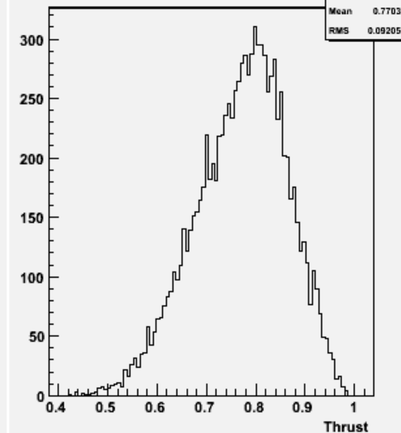
Thrust w101528 n3n3n2e2du_o
