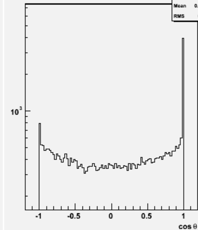
Jet cos \theta (All jets)w101528 n3n3n2e2du_o
