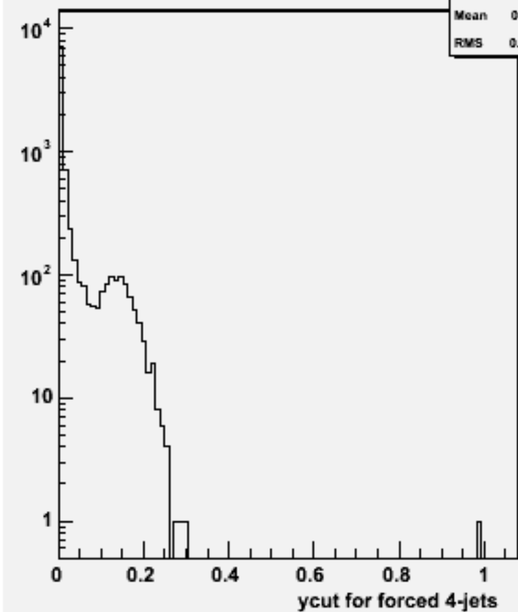
Ycut for 4-jets :w101528 n3n3n2e2du_o
