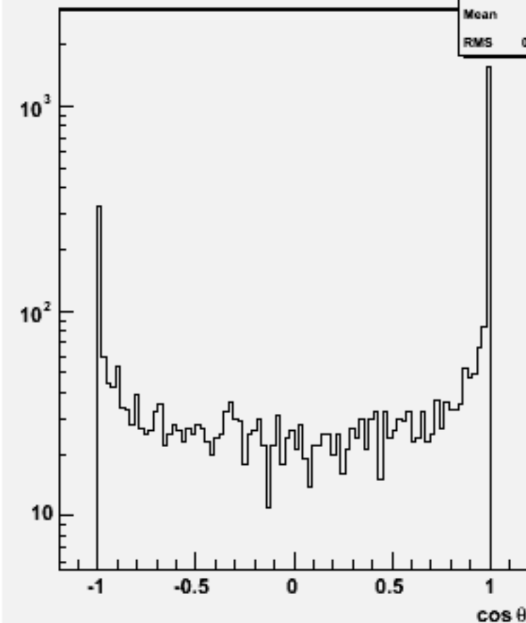
Jet cos \theta (All jets)w101521 n3n3n2e2e2n2_o
