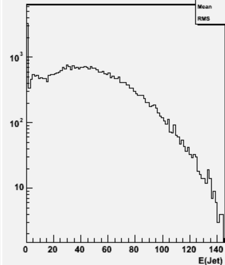
Jet energies(All jets)w101513 n3n3n1e1sc_o
