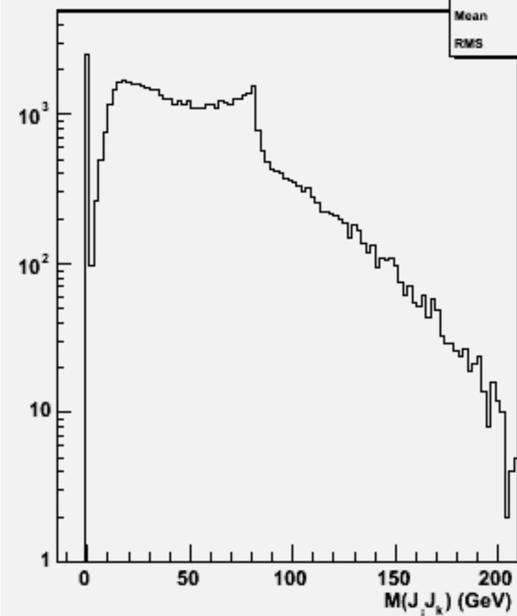
2jets mass(All comb)w101513 n3n3n1e1sc_o
