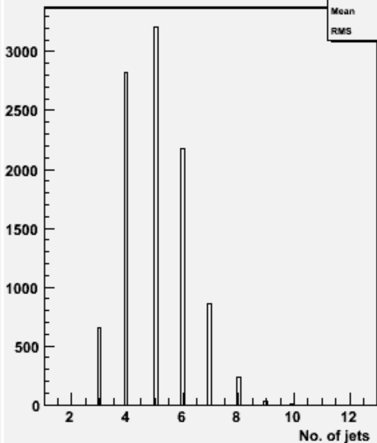
No. jets (ycut=0.001) : w101513 n3n3n1e1sc_o
