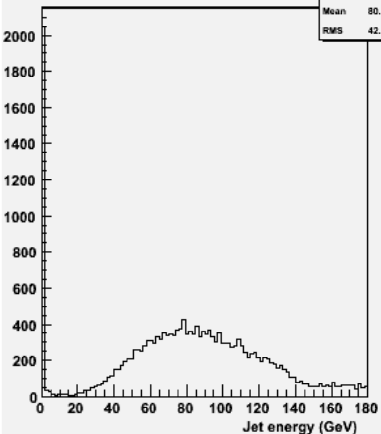
energy for 2-jets :w101513 n3n3n1e1sc_o
