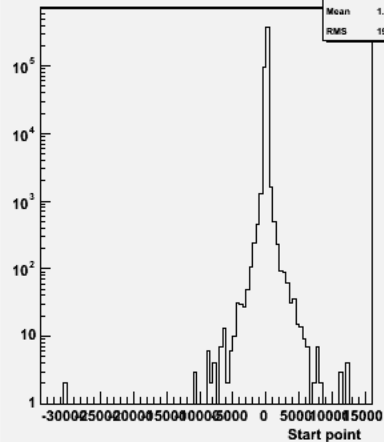
Start point Z : w101513 n3n3n1e1sc_o
