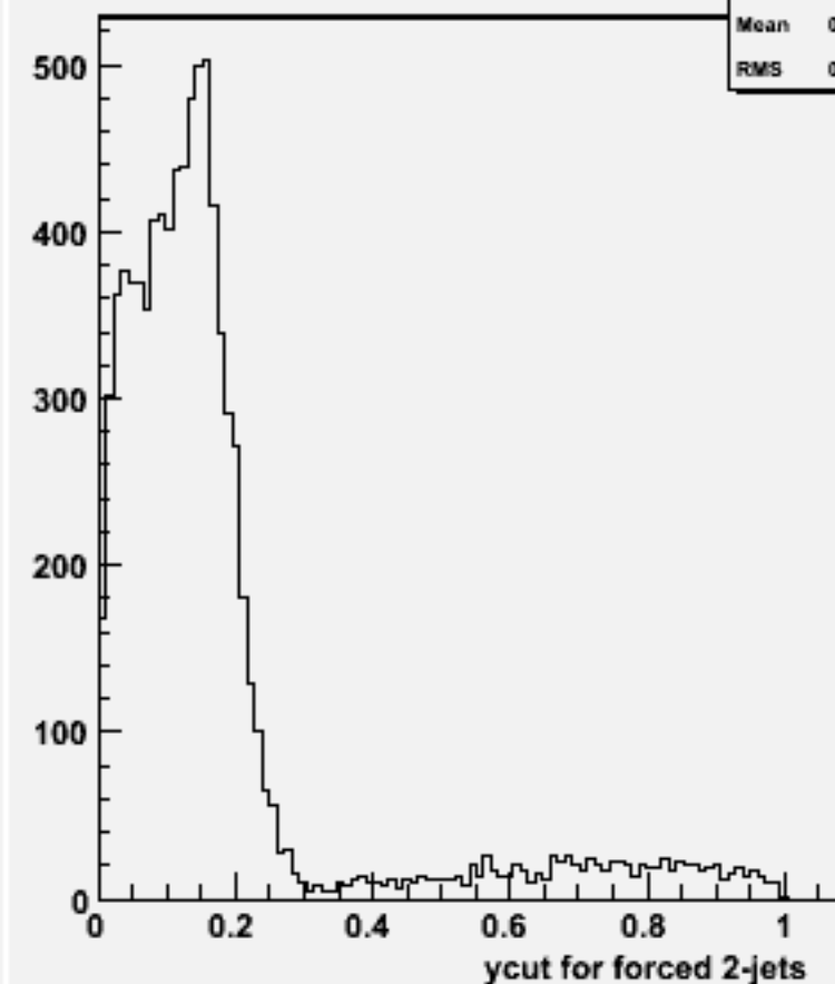
Ycut for 2-jets :w101513 n3n3n1e1sc_o
