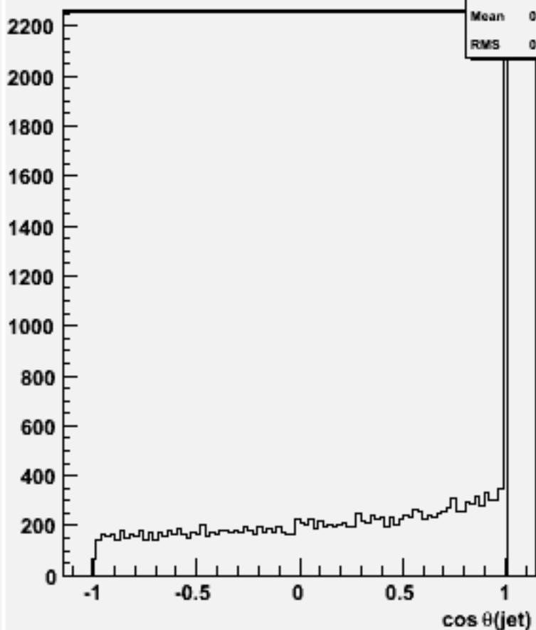
cos \theta for 2-jets :w101513 n3n3n1e1sc_o
