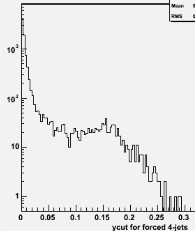
Ycut for 4-jets :w101513 n3n3n1e1sc_o
