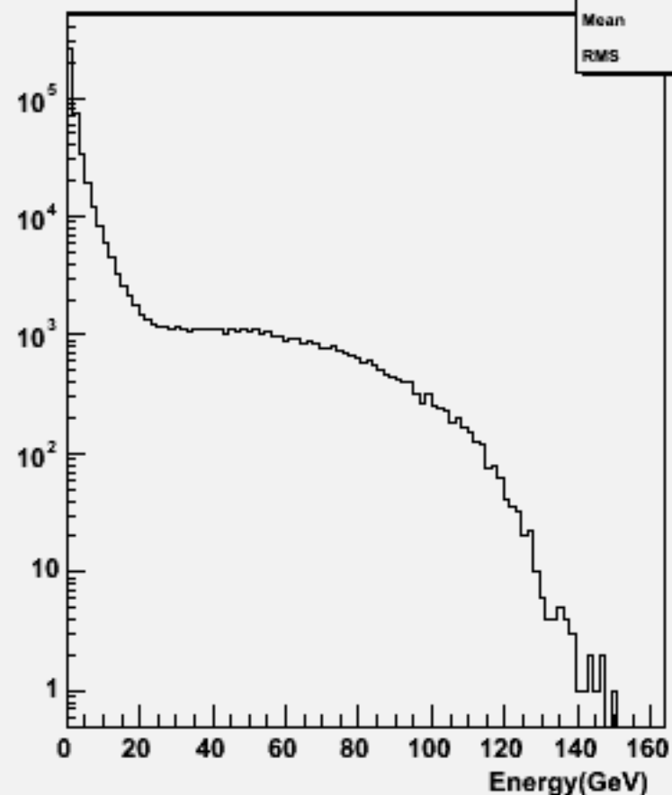
Particle Energy : w101513 n3n3n1e1sc_o
