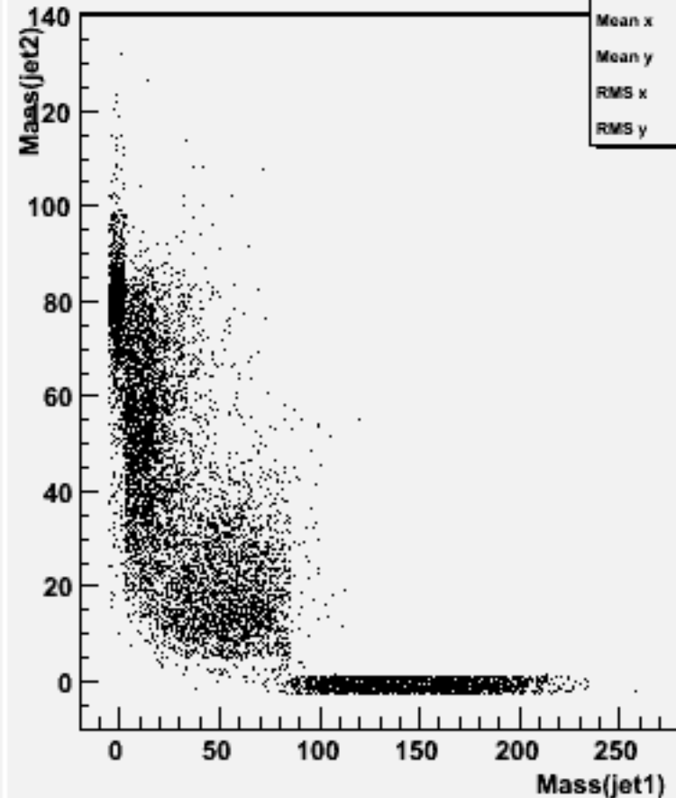
Jet mass for forced 2-jets : w101513 n3n3n1e1sc_o
