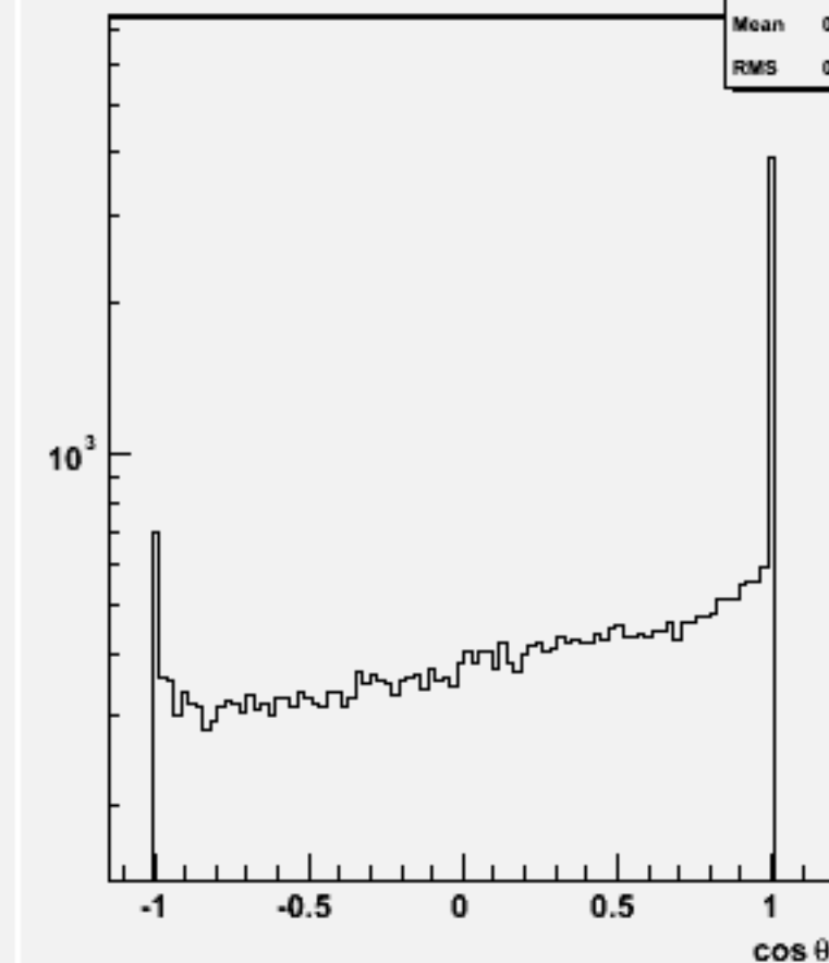
Jet cos \theta (All jets)w101513 n3n3n1e1sc_o
