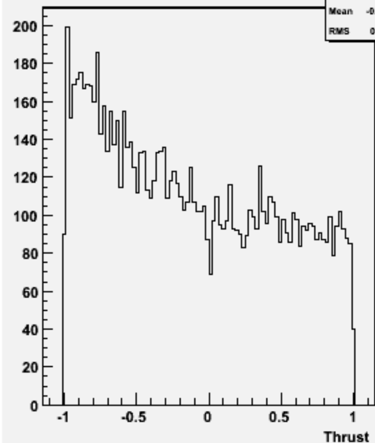
cos \Theta (thrust) w101513 n3n3n1e1sc_o
