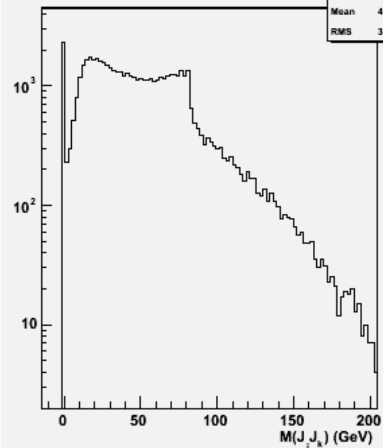
2jets mass(All comb)w101511 n3n3n1e1sc_o
