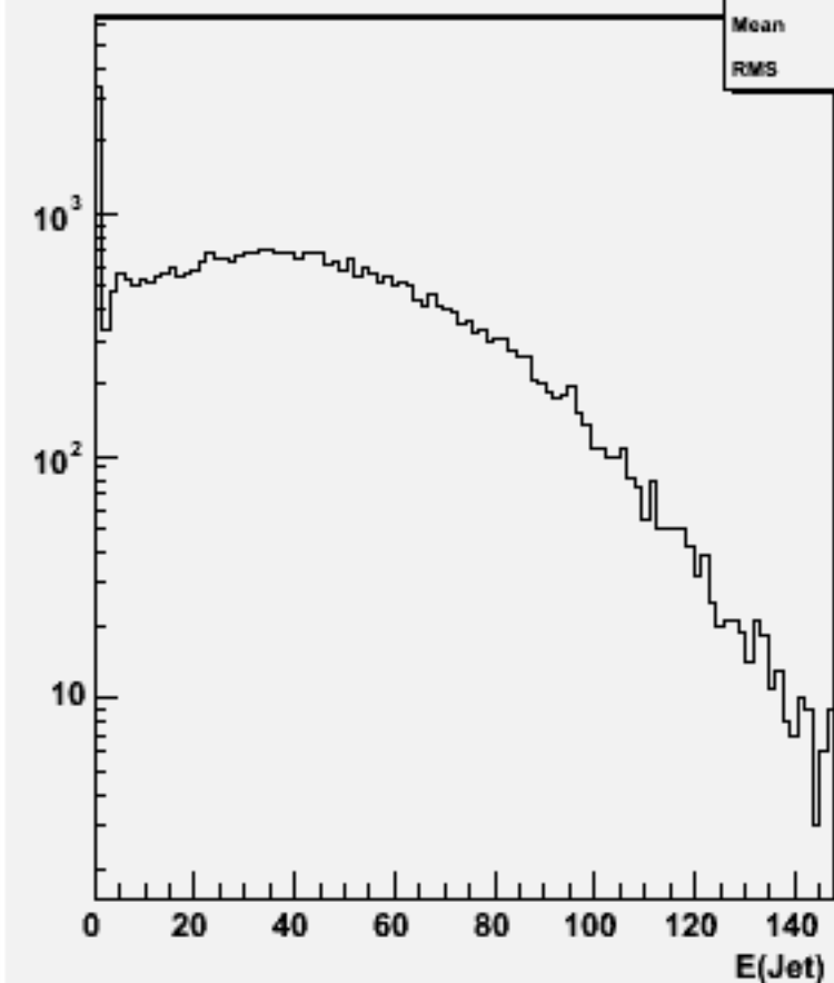
Jet energies(All jets)w101511 n3n3n1e1sc_o
