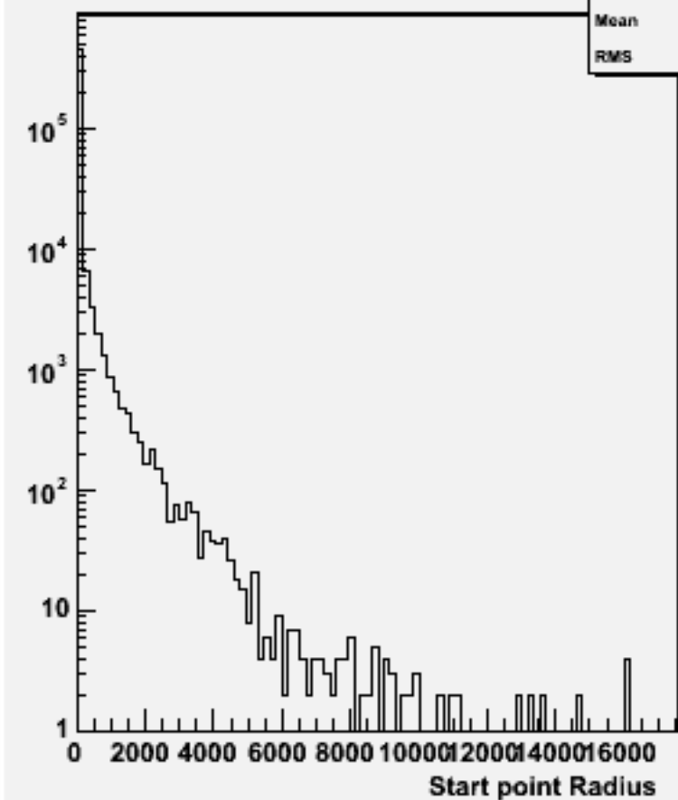
Start point R : w101511 n3n3n1e1sc_o
