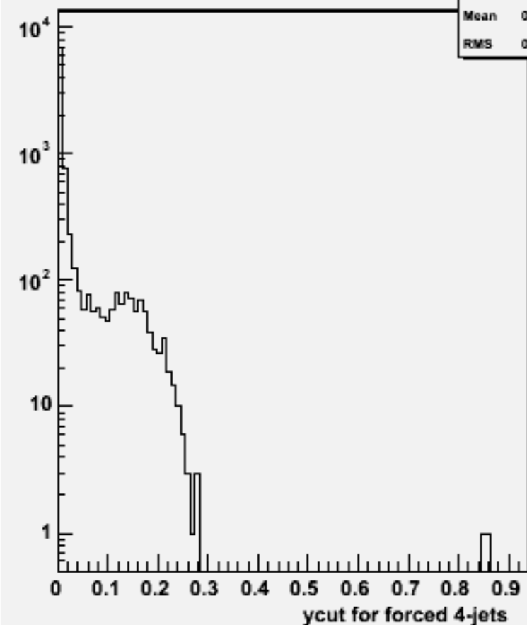
Ycut for 4-jets :w101511 n3n3n1e1sc_o
