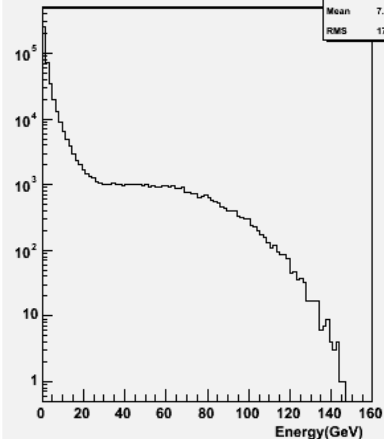
Particle Energy : w101511 n3n3n1e1sc_o
