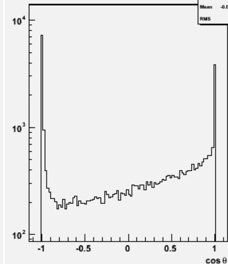
Jet cos \theta (All jets)w101511 n3n3n1e1sc_o
