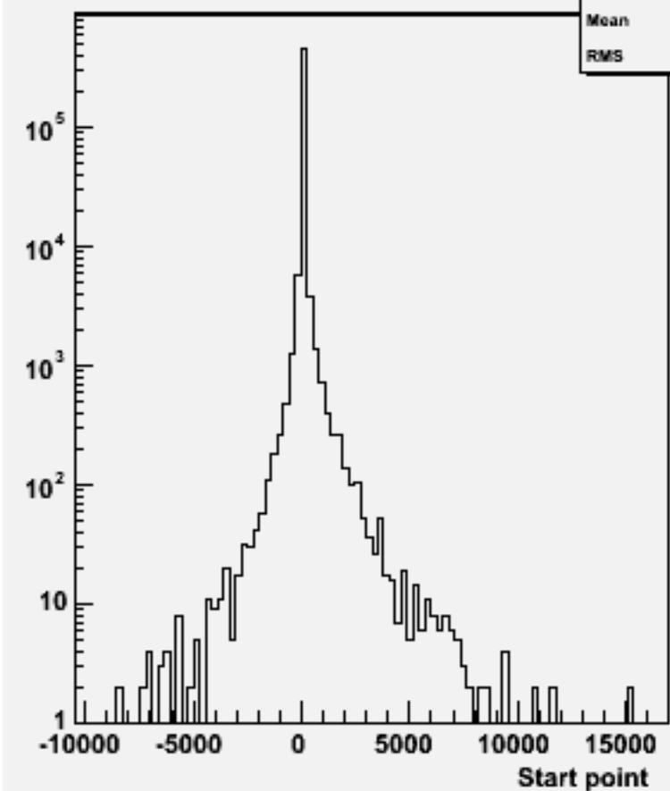
Start point Z : w101511 n3n3n1e1sc_o
