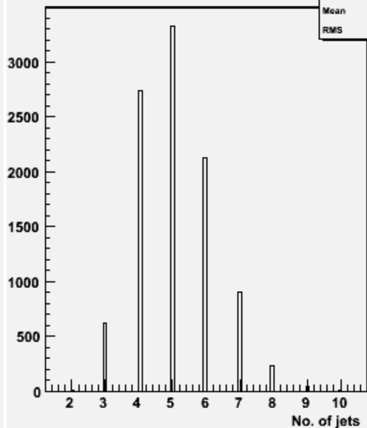
No. jets (ycut=0.001) : w101509 n3n3n1e1du_o
