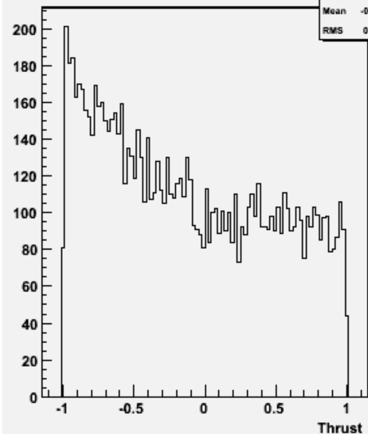
cos \Theta (thrust) w101509 n3n3n1e1du_o
