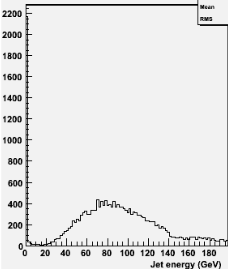
energy for 2-jets :w101509 n3n3n1e1du_o
