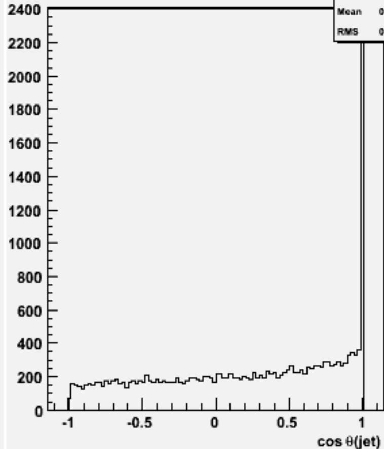
cos \theta for 2-jets :w101509 n3n3n1e1du_o
