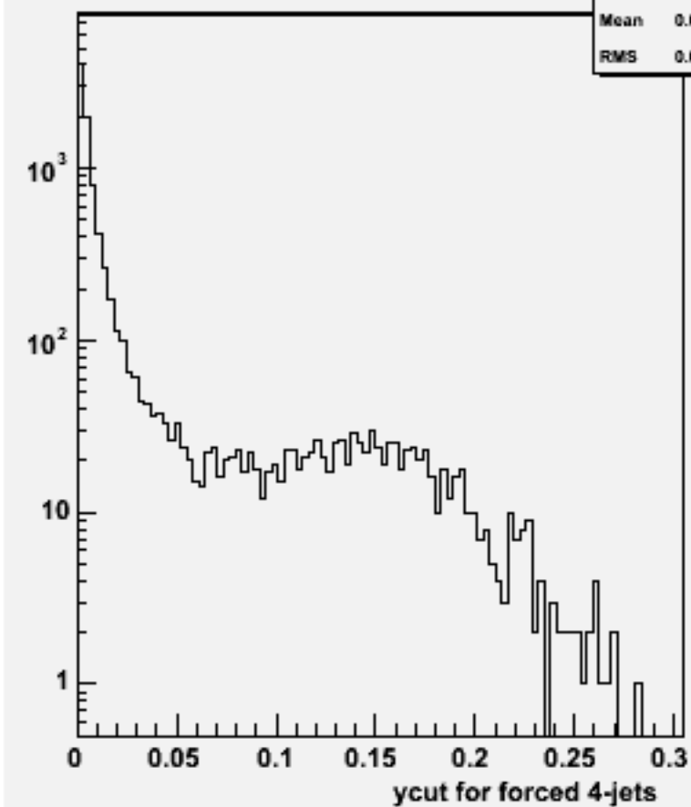
Ycut for 4-jets :w101509 n3n3n1e1du_o
