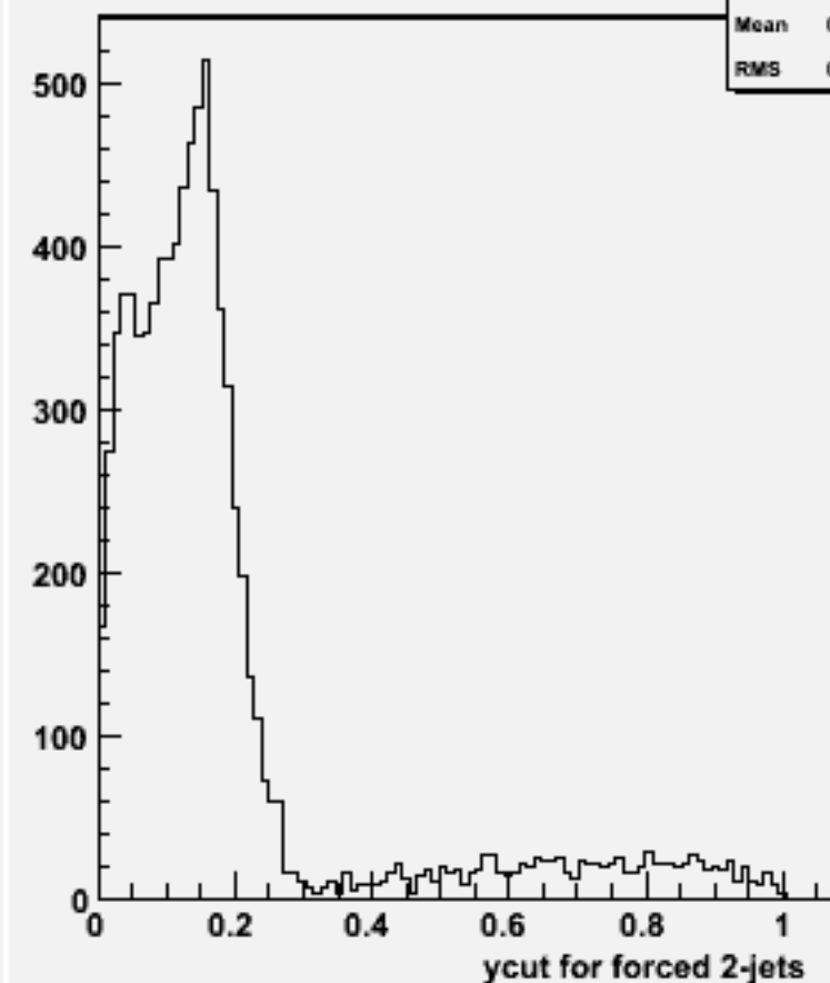
Ycut for 2-jets :w101509 n3n3n1e1du_o
