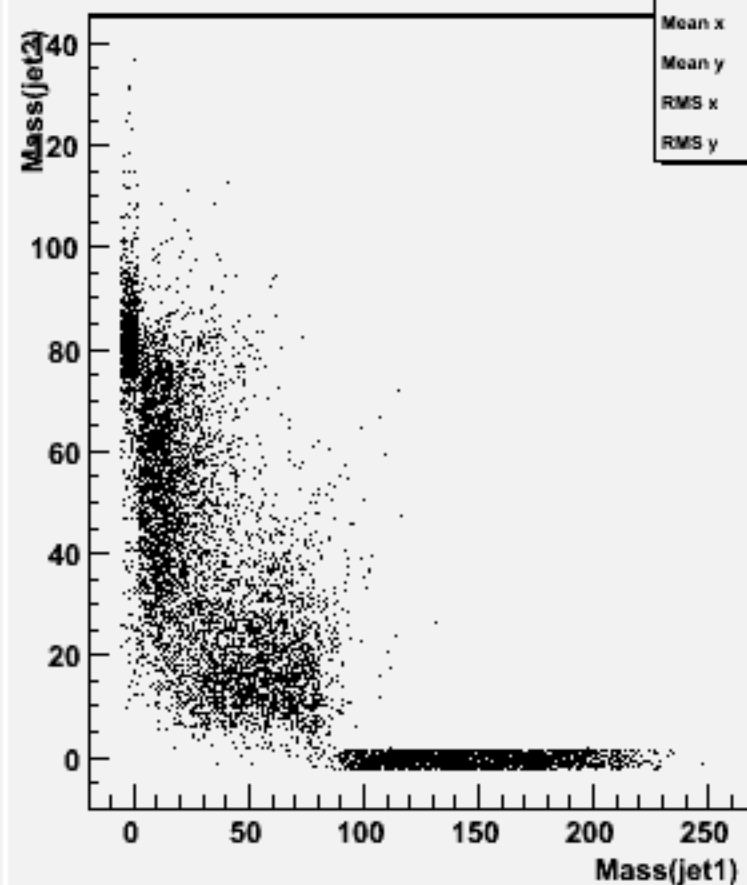
Jet mass for forced 2-jets : w101509 n3n3n1e1du_o
