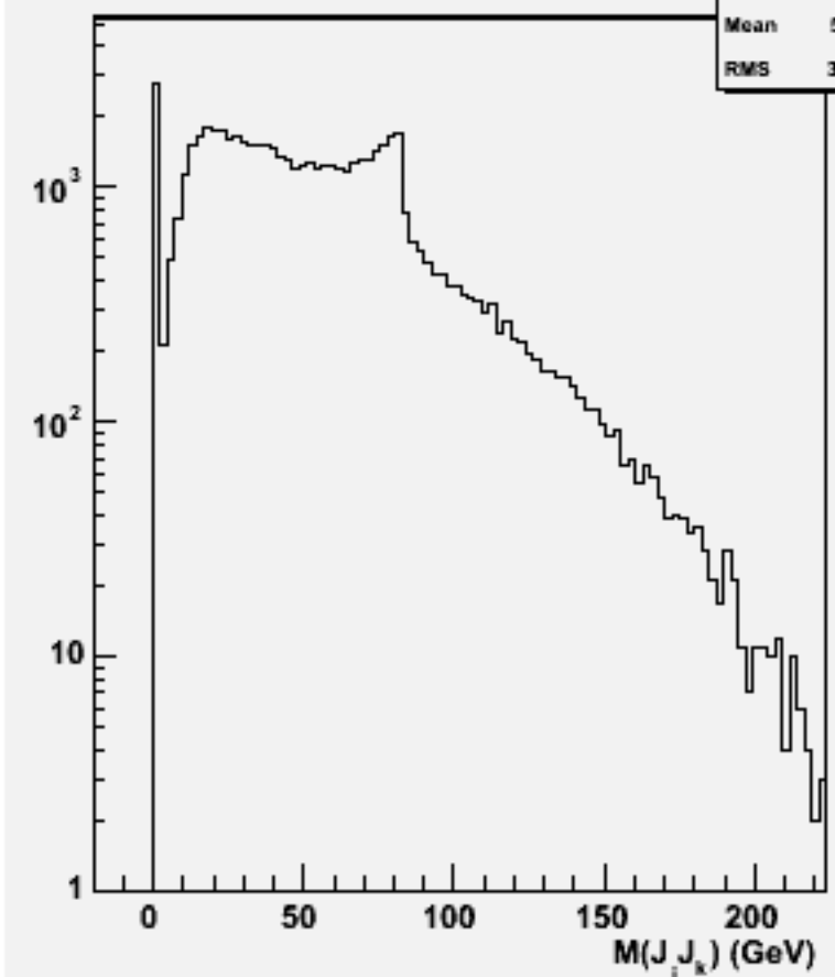
2jets mass(All comb)w101509 n3n3n1e1du_o
