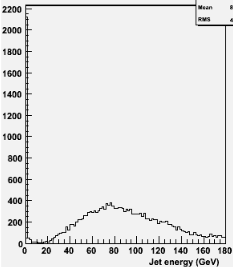
energy for 2-jets :w101508 n3n3n1e1du_o
