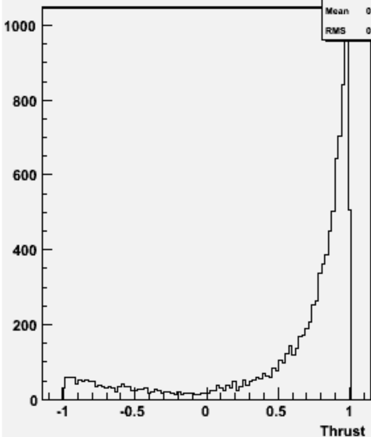
cos \Theta (thrust) w101508 n3n3n1e1du_o
