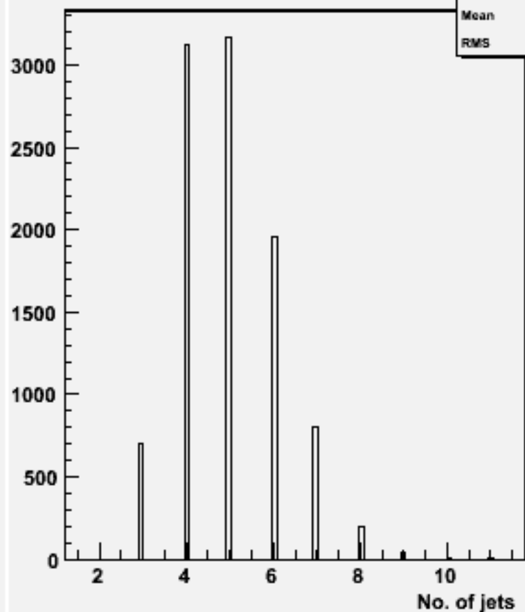
No. jets (ycut=0.001) : w101508 n3n3n1e1du_o
