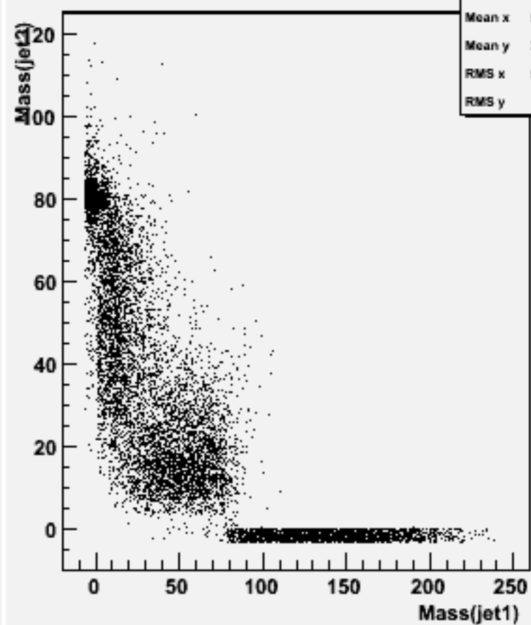
Jet mass for forced 2-jets : w101508 n3n3n1e1du_o
