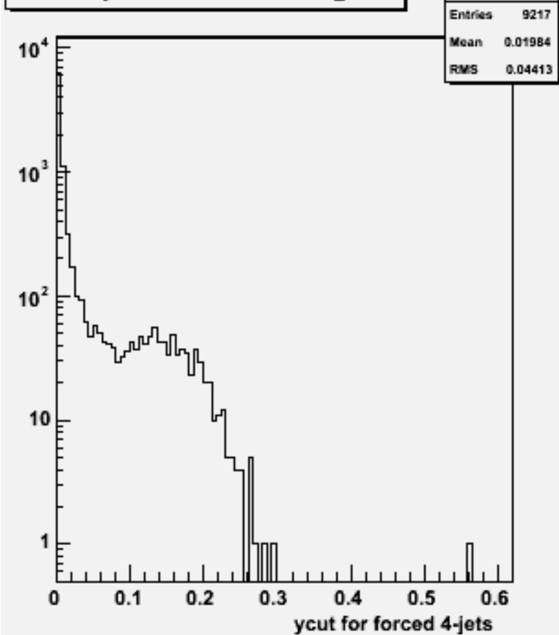
Ycut for 4-jets :w101507 n3n3n1e1du_o
