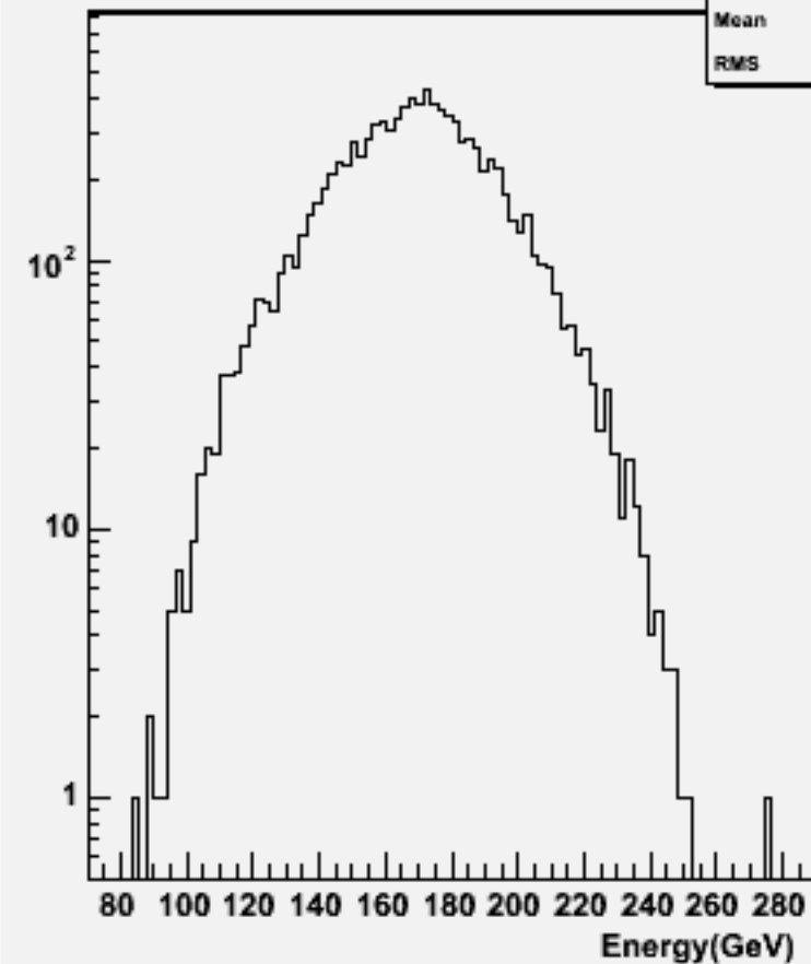
Thrust w101507 n3n3n1e1du_o
