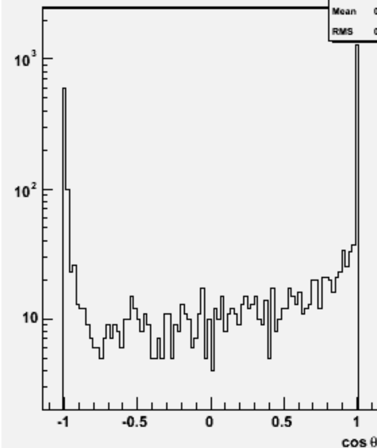
Jet cos \theta (All jets)w101504 n3n3n1e1e3n3_o
