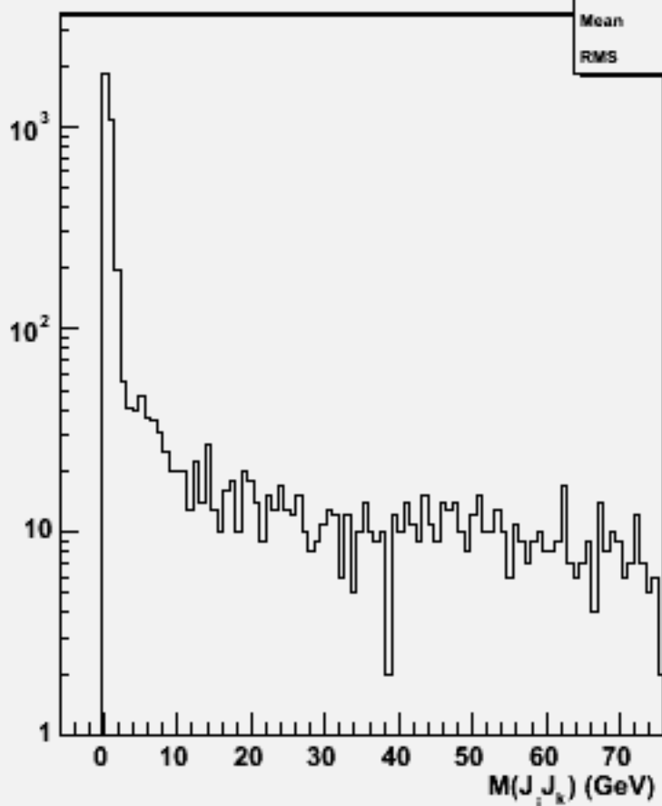
2jets mass(All comb)w101504 n3n3n1e1e3n3_o
