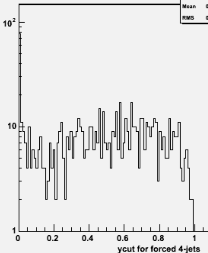
Ycut for 4-jets :w101503 n3n3n1e1e3n3_o
