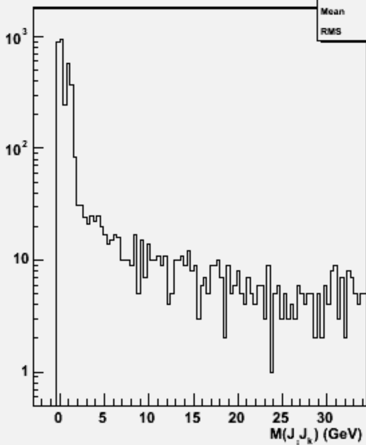
2jets mass(All comb)w101503 n3n3n1e1e3n3_o
