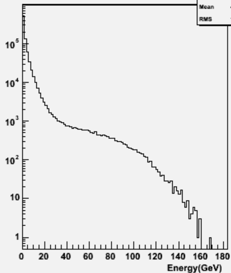
Particle Energy : w101493 n2n2cssc_o
