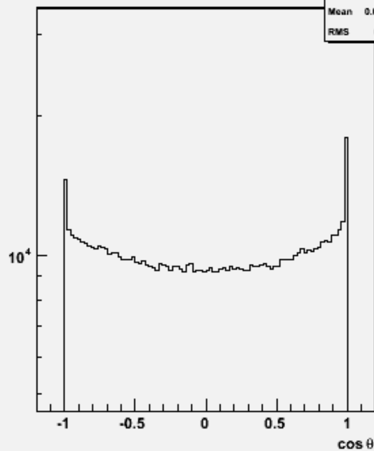
Particle cos \theta : w101493 n2n2cssc_o
