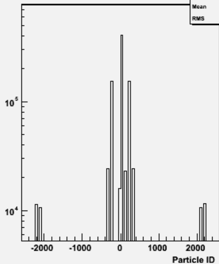
Particle ID : w101493 n2n2cssc_o
