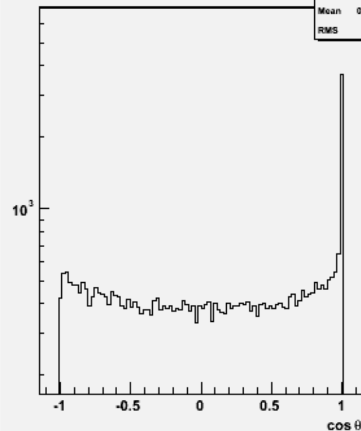
Jet cosθ (All jets)w101493 n2n2cssc_o
