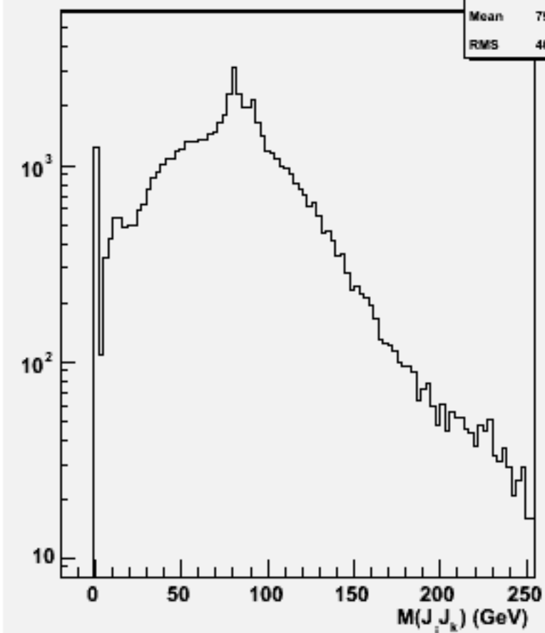
2jets mass(All comb)w101493 n2n2cssc_o
