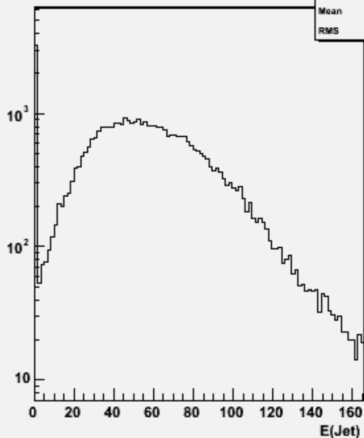
Jet energies(All jets)w101493 n2n2cssc_o
