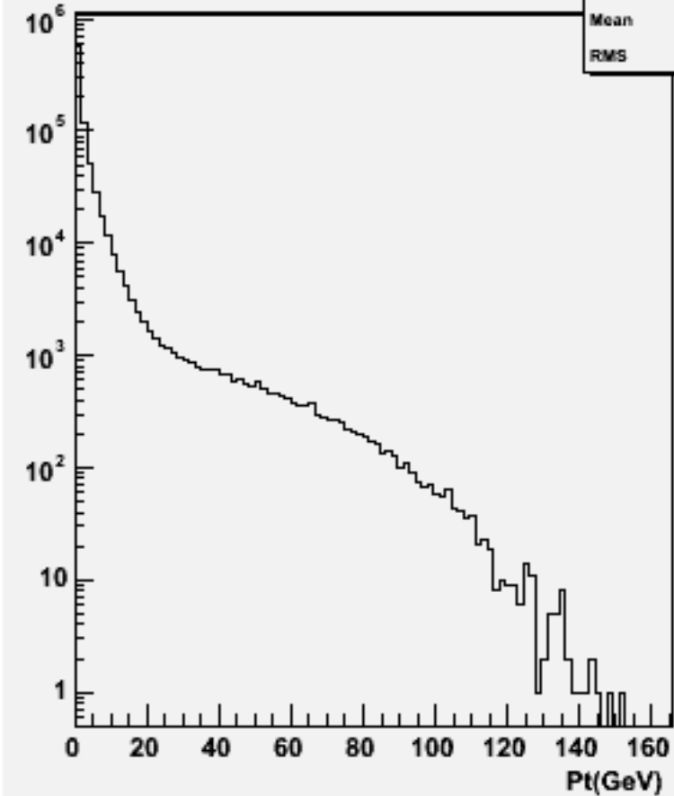
Particle Pt : w101493 n2n2cssc_o
