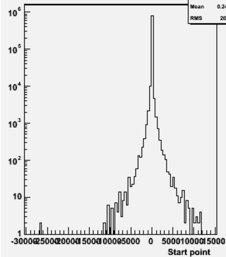
Start point Z : w101493 n2n2cssc_o
