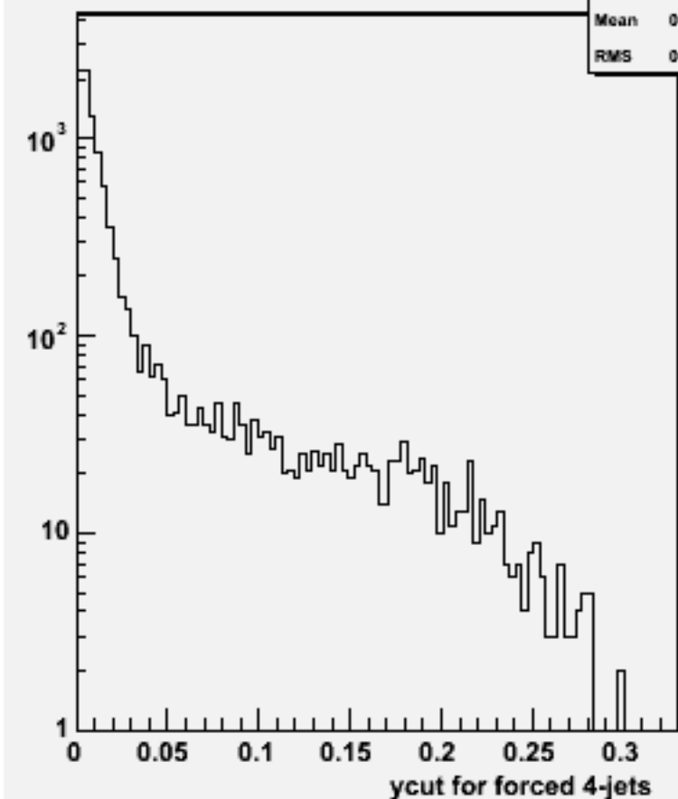
Ycut for 4-jets :w101493 n2n2cssc_o
