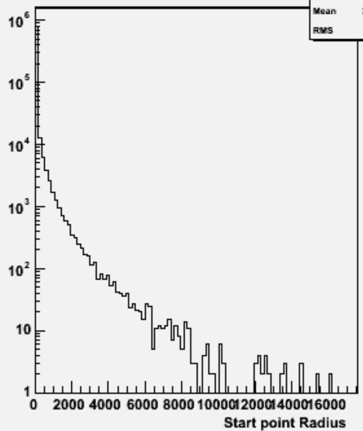
Start point R : w101493 n2n2cssc_o
