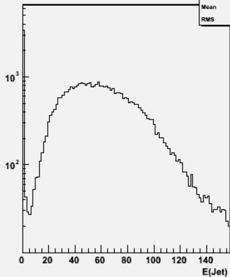
Jet energies(All jets)w101492 n2n2cssc_o
