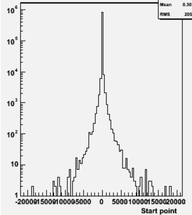
Start point Z : w101492 n2n2cssc_o
