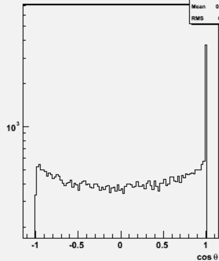
Jet cosθ (All jets)w101492 n2n2cssc_o
