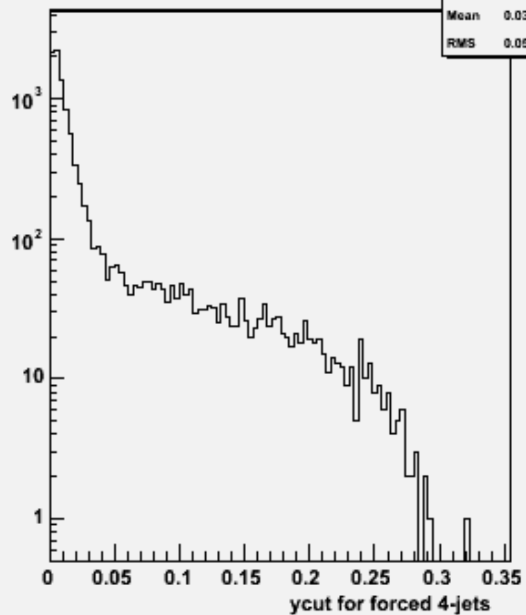
Ycut for 4-jets :w101492 n2n2cssc_o
