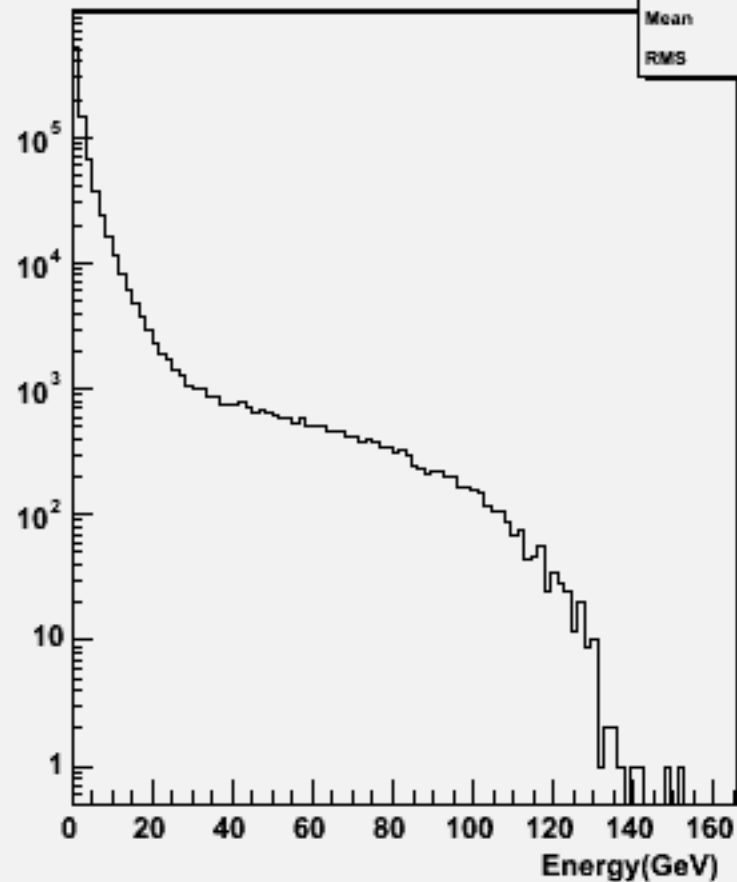
Start point R : w101492 n2n2cssc_o
