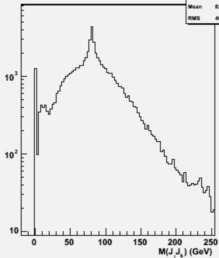
2jets mass(All comb)w101492 n2n2cssc_o
