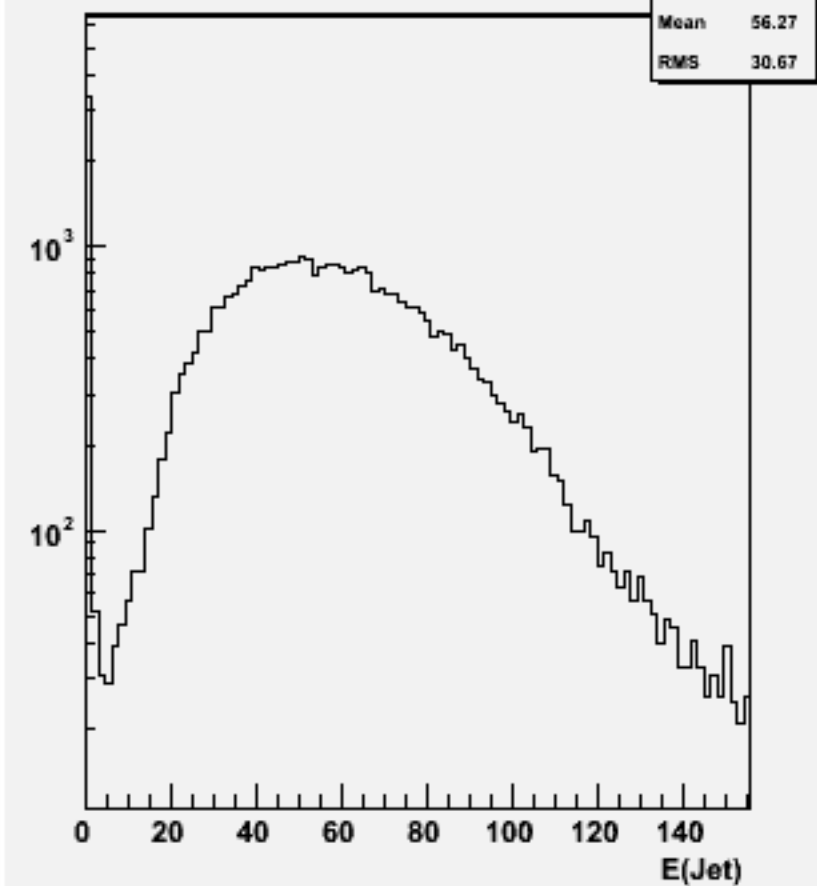
Jet energies(All jets)w101489 n2n2csdu_o
