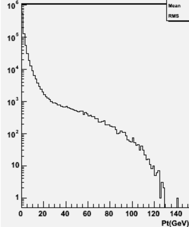
Particle Pt : w101489 n2n2csdu_o
