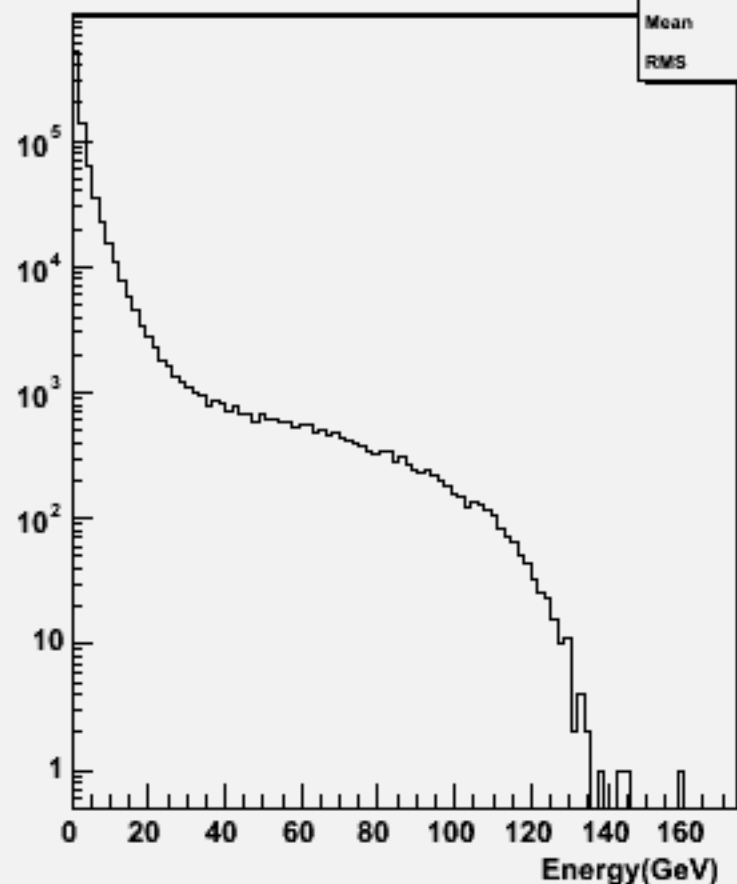
Particle Energy : w101489 n2n2csdu_o
