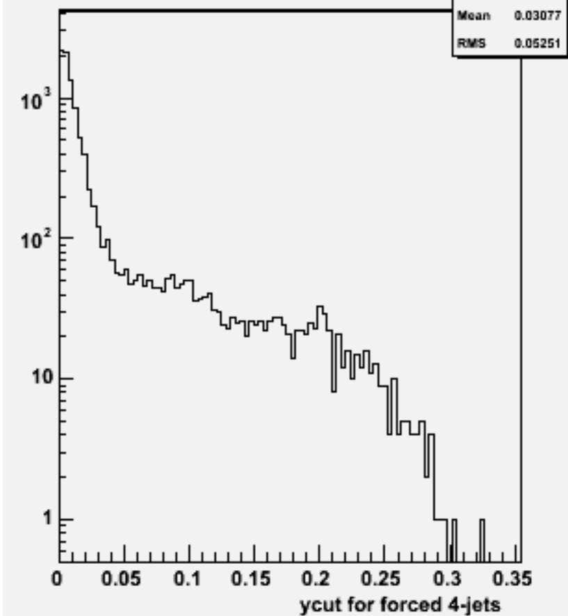
Ycut for 4-jets :w101489 n2n2csdu_o
