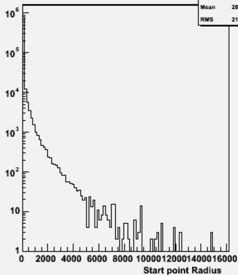
Start point R : w101489 n2n2csdu_o
