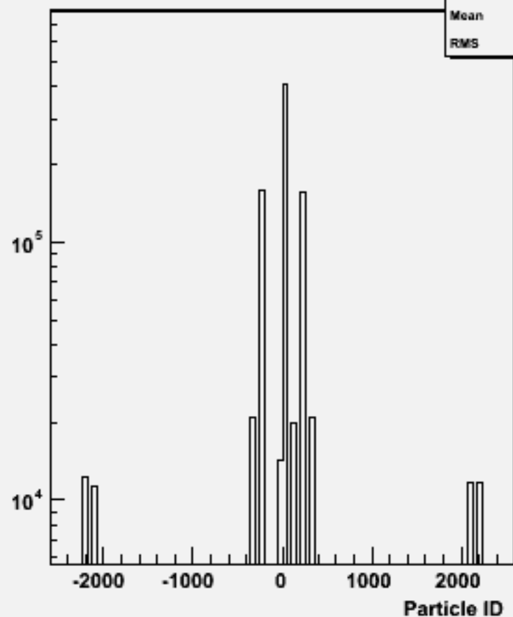
Particle ID : w101489 n2n2csdu_o
