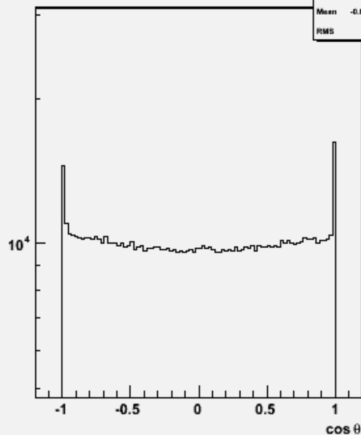
Particle cos \theta : w101489 n2n2csdu_o
