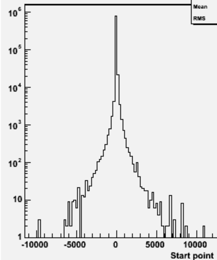
Start point Z : w101489 n2n2csdu_o
