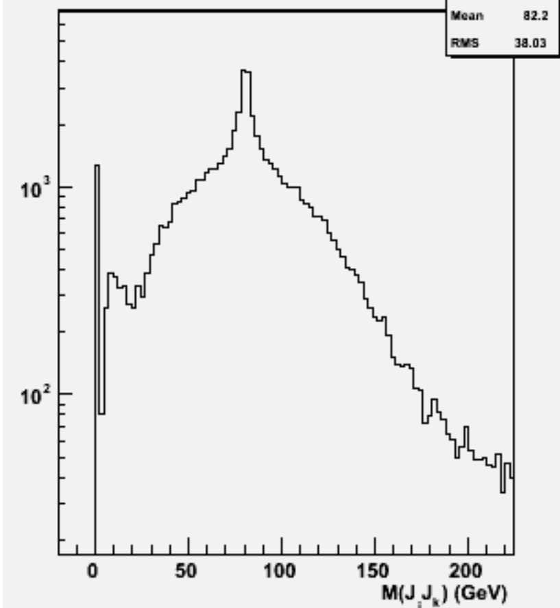
2jets mass(All comb)w101489 n2n2csdu_o
