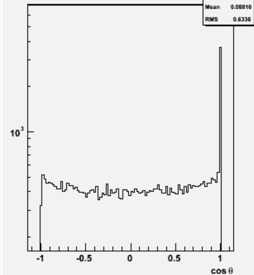
Jet cos \theta (All jets)w101489 n2n2csdu_o
