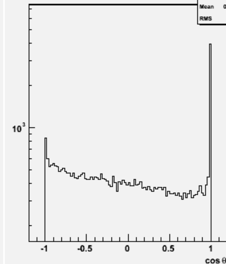
Jet cos \theta (All jets)w101485 n2n2cse3n3_o
