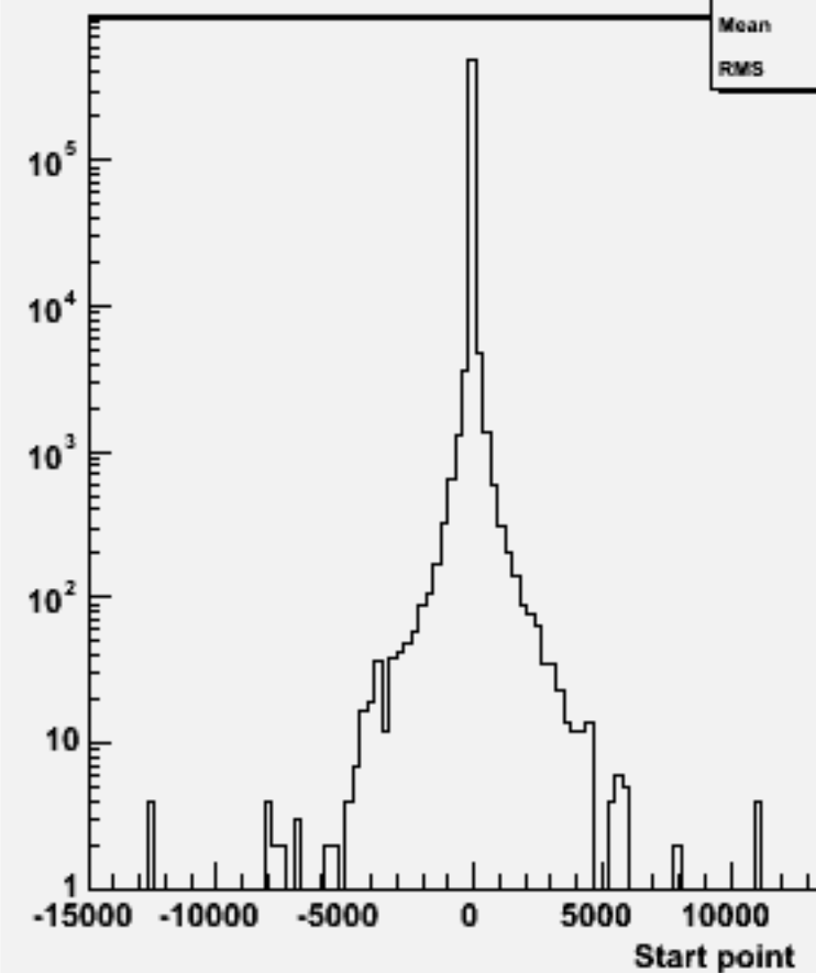
Start point Z : w101485 n2n2cse3n3_o
