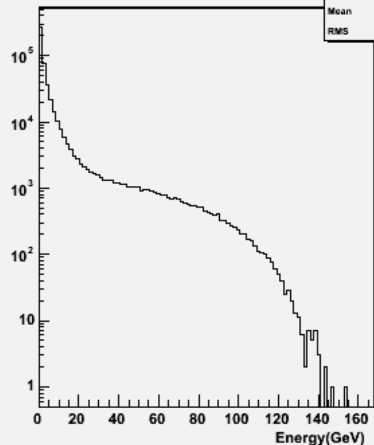
Start point R : w101485 n2n2cse3n3_o
