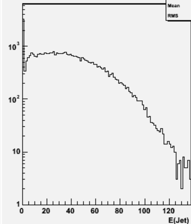
Jet energies(All jets)w101485 n2n2cse3n3_o
