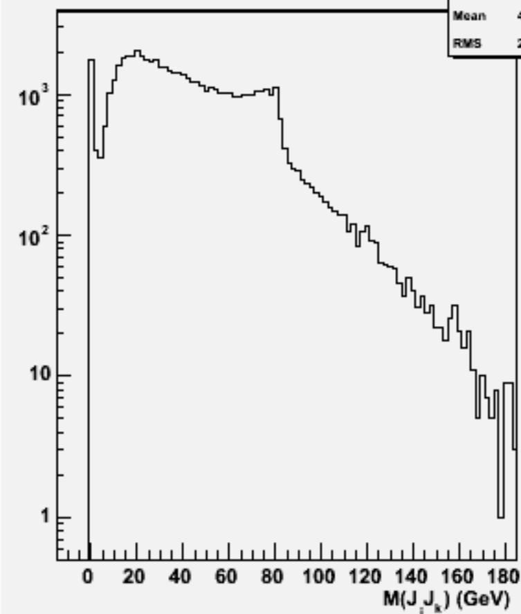
2jets mass(All comb)w101485 n2n2cse3n3_o
