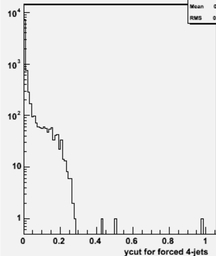
Ycut for 4-jets :w101485 n2n2cse3n3_o
