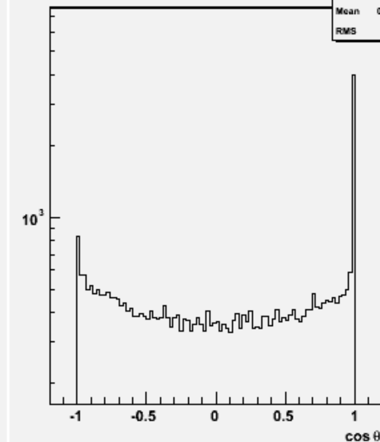
Jet cos \theta (All jets)w101484 n2n2cse3n3_o
