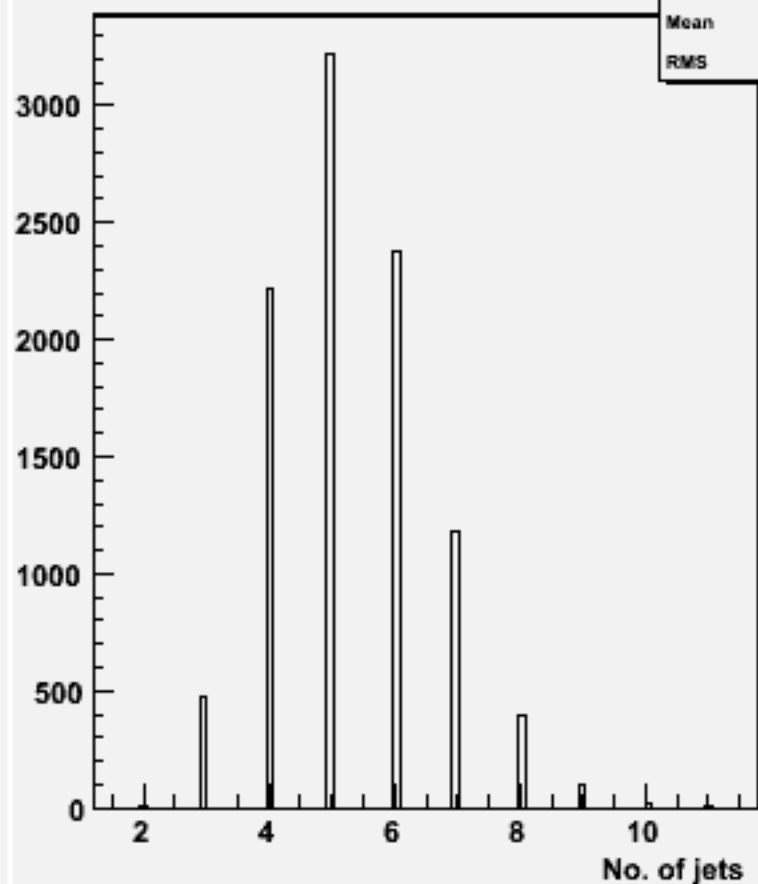
No. jets (ycut=0.001) : w101484 n2n2cse3n3_o
