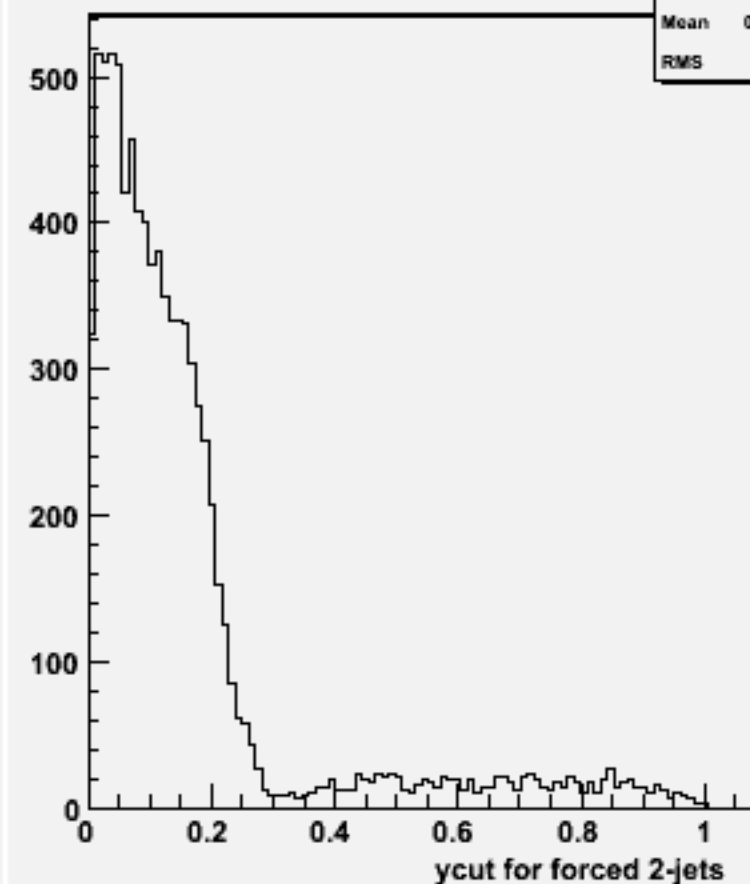
Ycut for 2-jets :w101484 n2n2cse3n3_o
