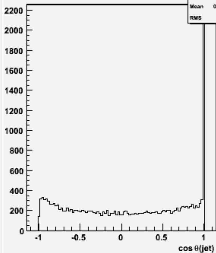
cos \theta for 2-jets :w101484 n2n2cse3n3_o
