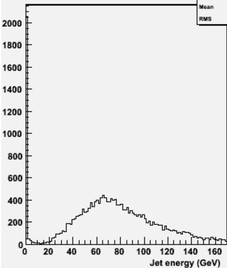
energy for 2-jets :w101484 n2n2cse3n3_o
