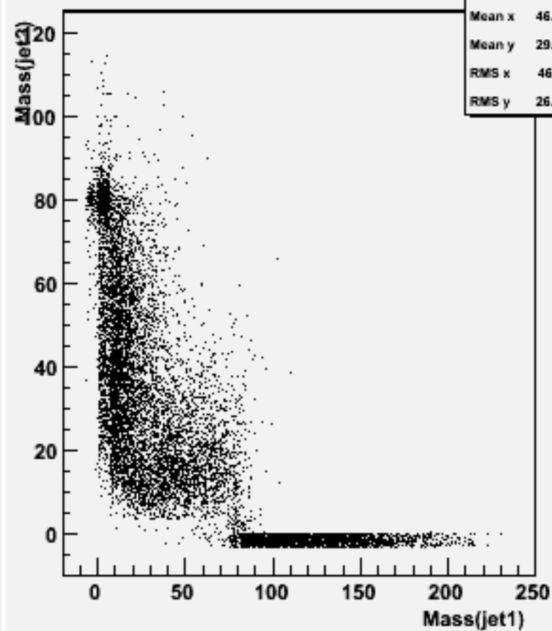
Jet mass for forced 2-jets : w101484 n2n2cse3n3_o
