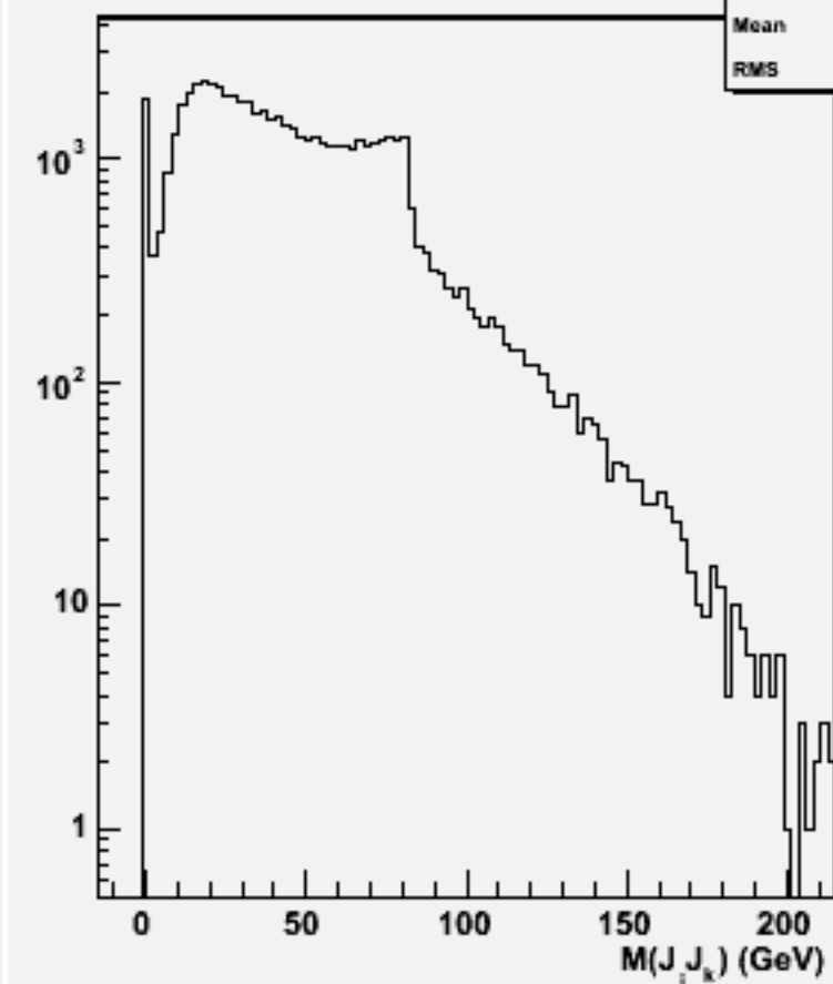
2jets mass(All comb)w101484 n2n2cse3n3_o
