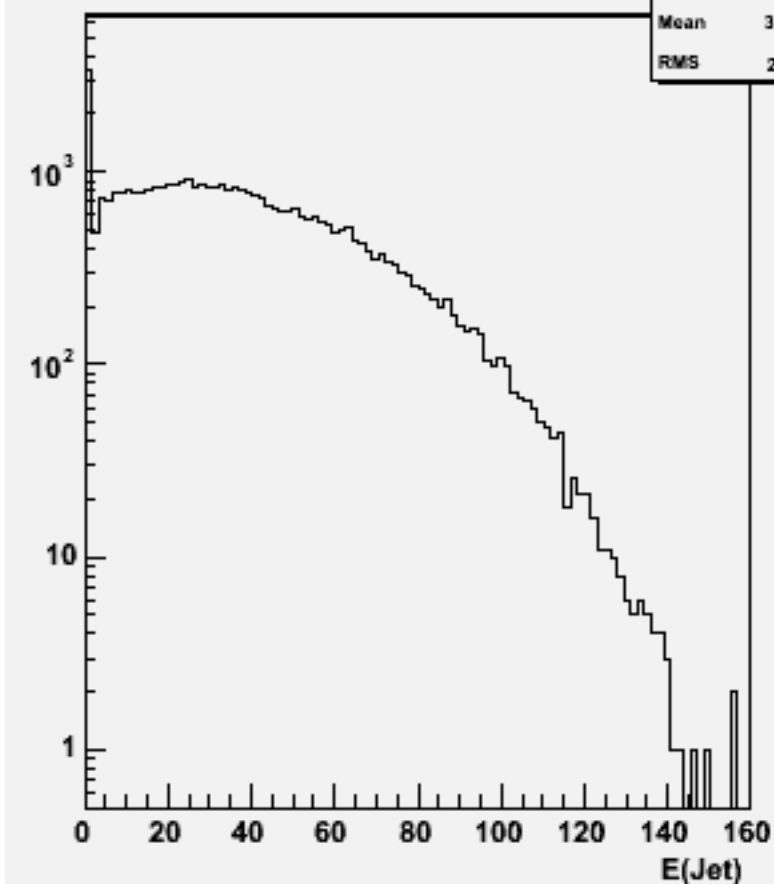
Jet energies(All jets)w101484 n2n2cse3n3_o
