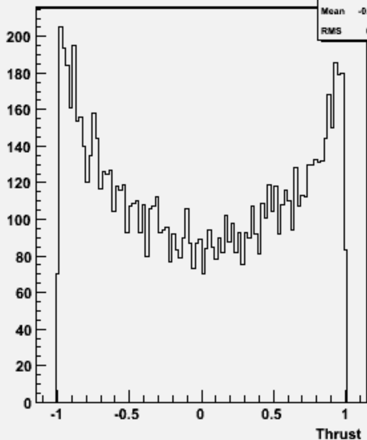
cos \Theta (thrust) w101484 n2n2cse3n3_o
