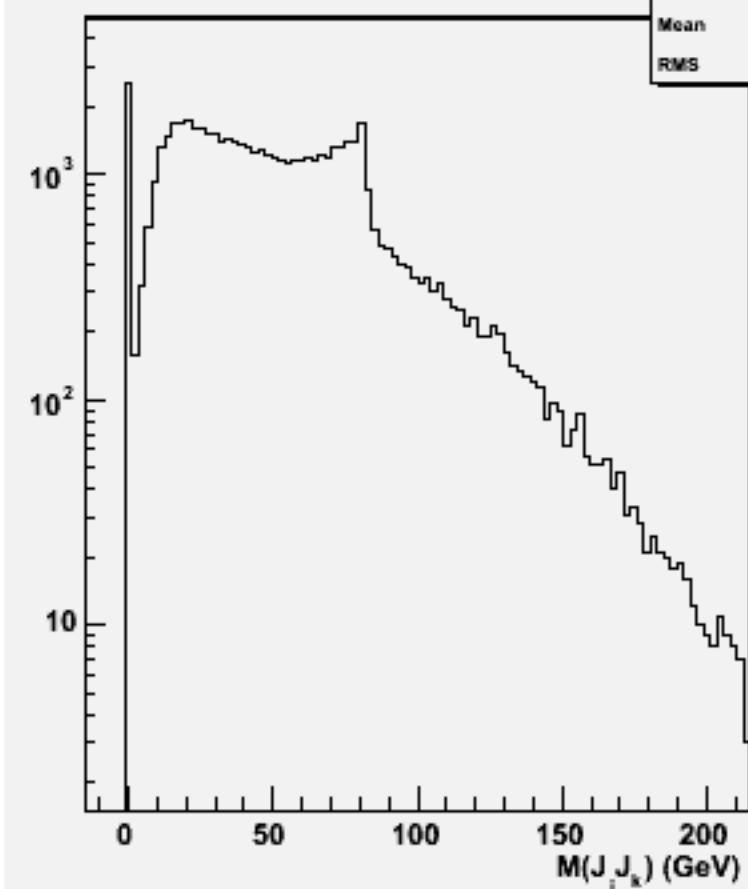
2jets mass(All comb)w101481 n2n2cse2n2_o
