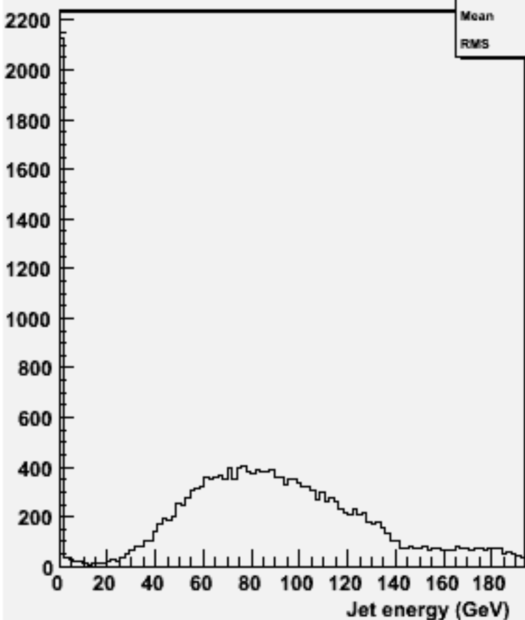
energy for 2-jets :w101481 n2n2cse2n2_o
