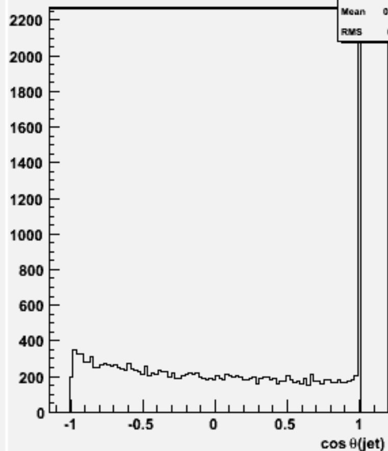
cos \theta for 2-jets :w101481 n2n2cse2n2_o
