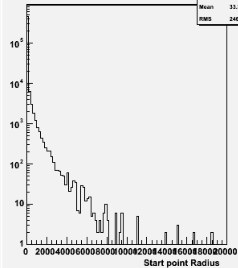
Start point R : w101481 n2n2cse2n2_o
