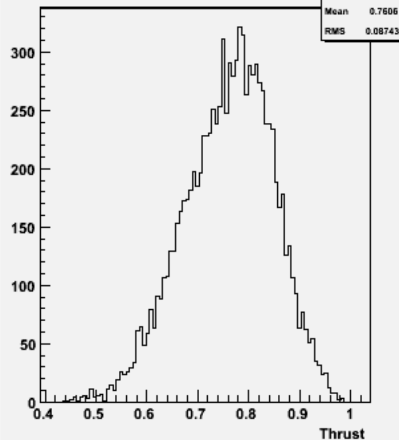
Thrust w101481 n2n2cse2n2_o
