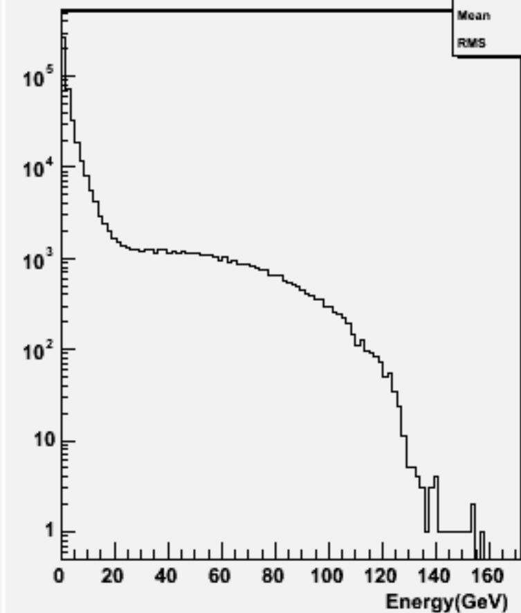
Start point R : w101481 n2n2cse2n2_o
