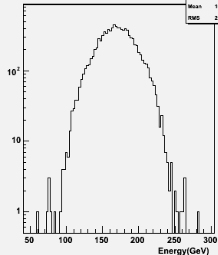
Thrust w101481 n2n2cse2n2_o
