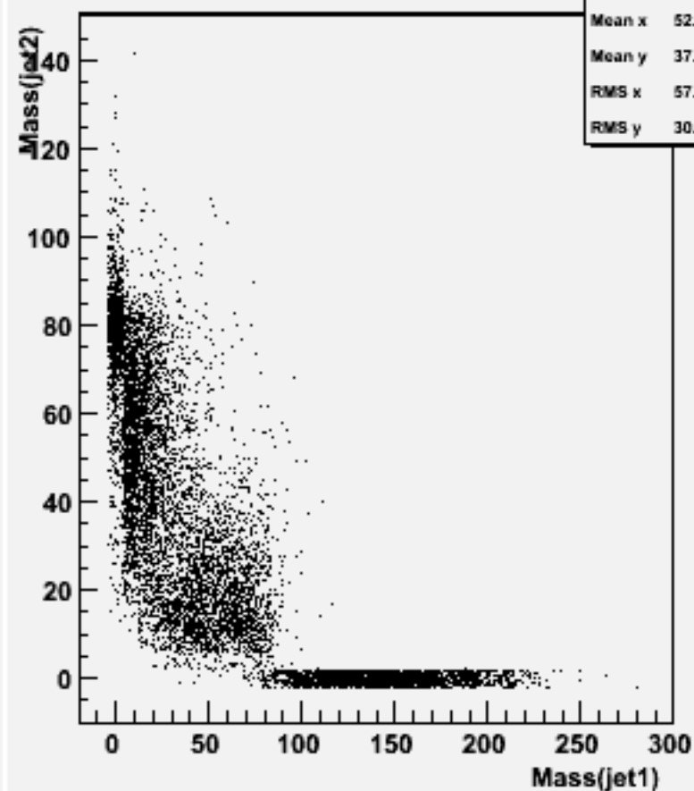
Jet mass for forced 2-jets : w101481 n2n2cse2n2_o
