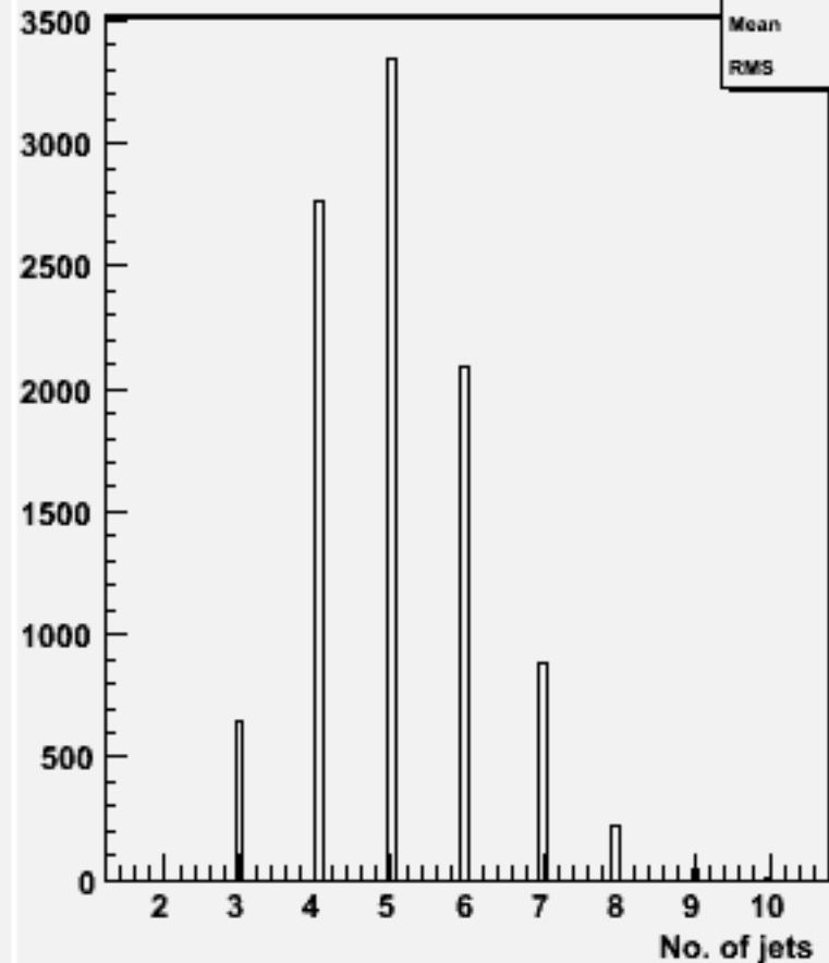
No. jets (ycut=0.001) : w101481 n2n2cse2n2_o
