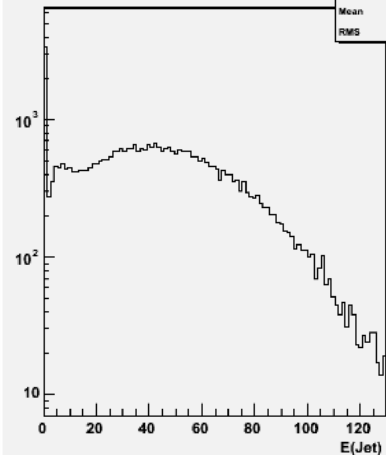
Jet energies(All jets)w101481 n2n2cse2n2_o
