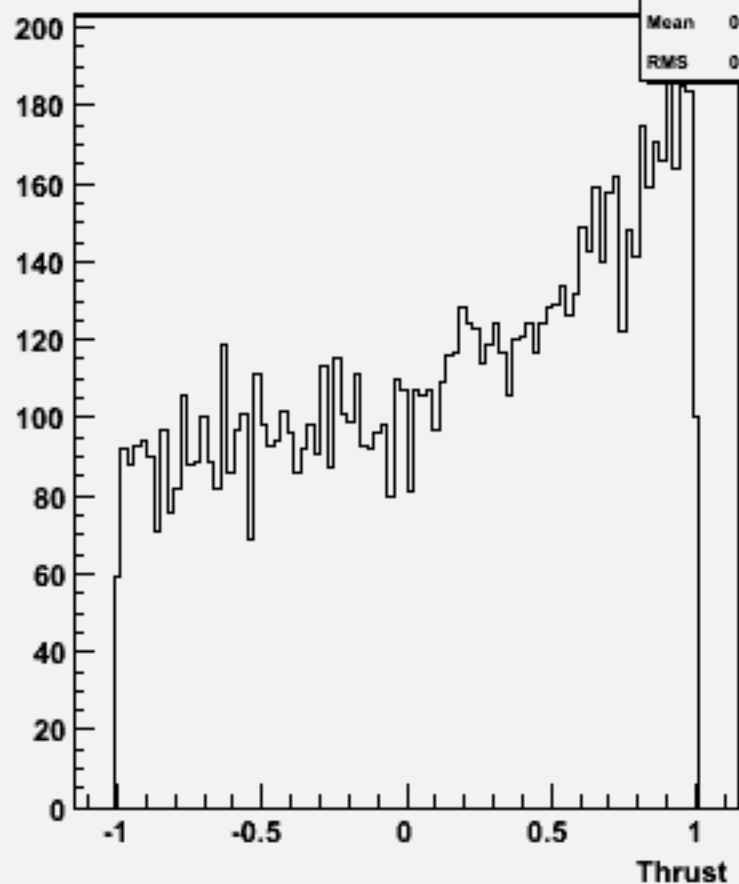
cos \Theta (thrust) w101481 n2n2cse2n2_o
