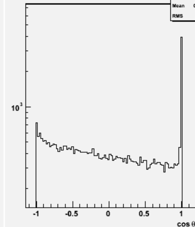
Jet cos \theta (All jets)w101481 n2n2cse2n2_o
