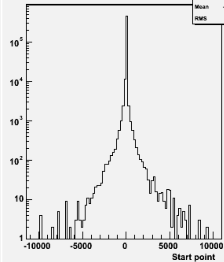
Start point Z : w101481 n2n2cse2n2_o
