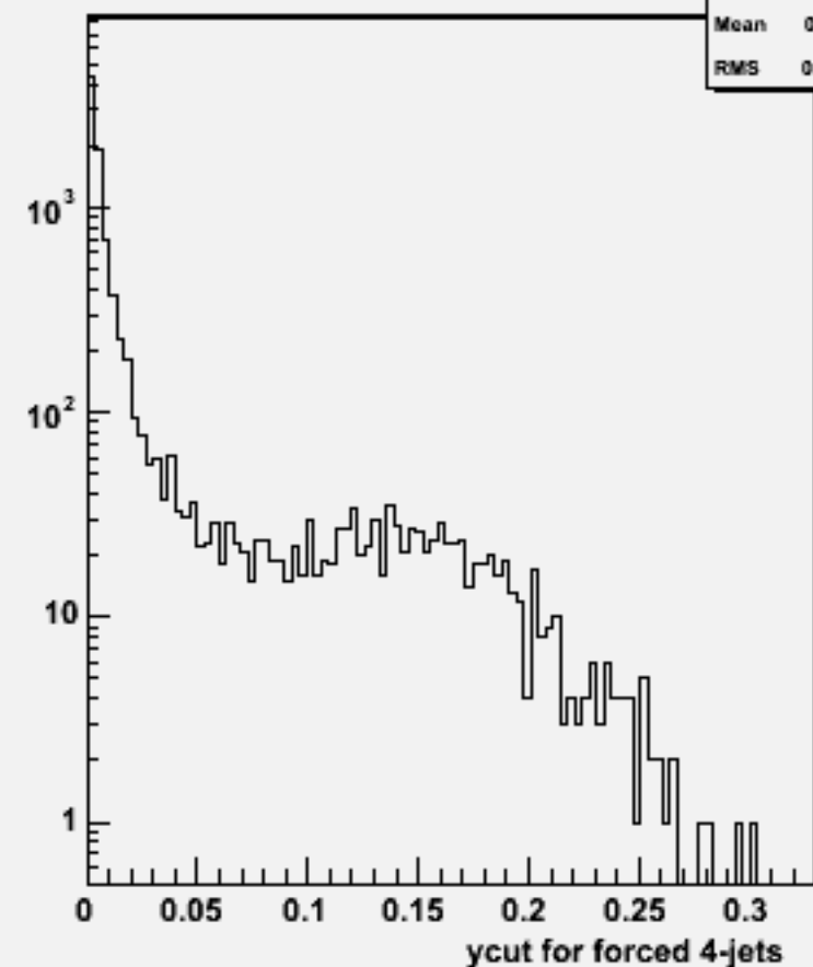
Ycut for 4-jets :w101481 n2n2cse2n2_o
