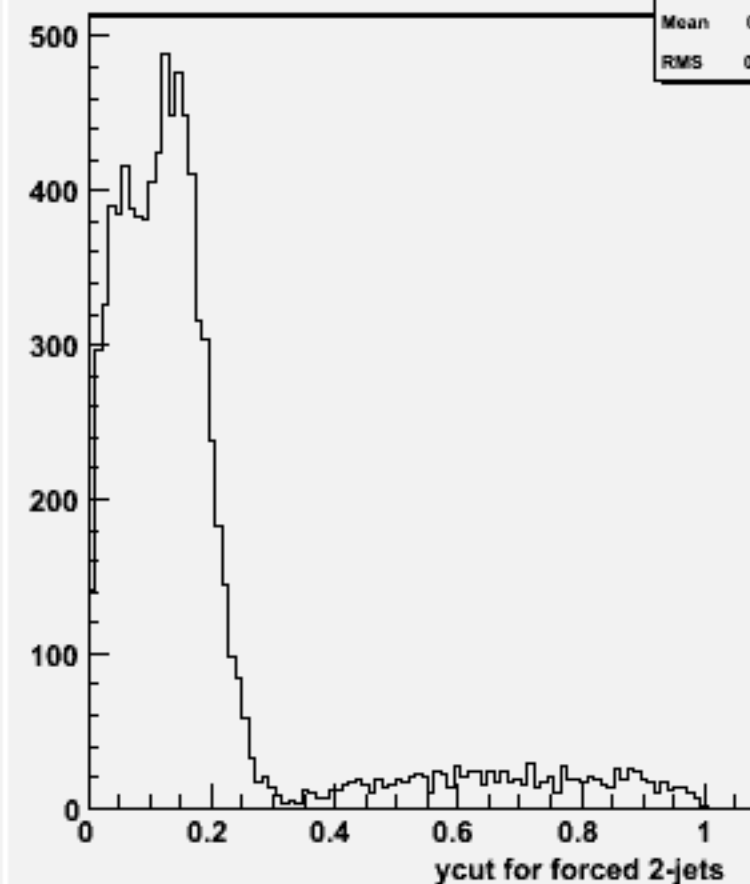
Ycut for 2-jets :w101481 n2n2cse2n2_o
